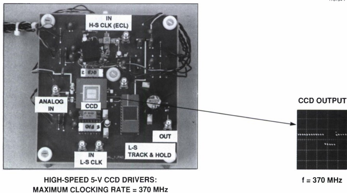
Figure 9. Multilayer board and output of the nonuniform, short-channel CCD for f_c = 370 MHz.
