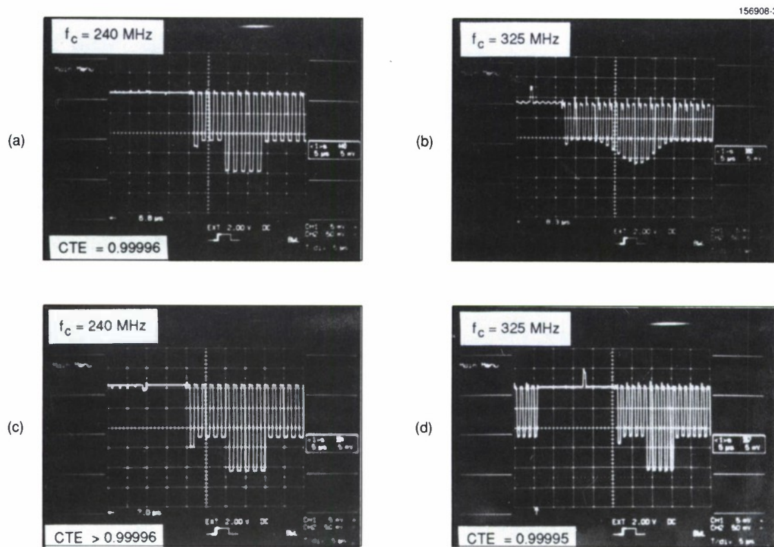
Figure 8. Output from the CCDs when the input is one pulse and five clock periods long for the following cases: (a) uniform doping, f_c = 240 MHz, (b) uniform doping, f_c = 325 MHz, (c) step doping, f_c = 240 MHz, and (d) step doping, f_c = 325 MHz.
