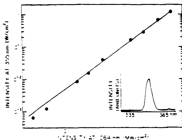
Fig. 1. Log-log plot of the third harmonic intensity (W/cm 2 ) as a function of the fundamental intensity (MW/cm 2 ). The solid line indicates a cubic dependence of the third harmonic intensities on the fundamental intensity. The inset shows that the spectral content of the third harmonic is resolution limited at 355 nm.
