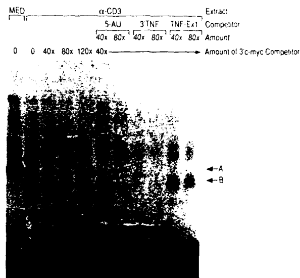
FIG. 4. Specificity of factor B binding. Cytoplasmic extracts from unstimulated (MED) T cells or from T cells that had been stimulated for 6 h with \alpha -CD3 antibody ( \alpha -CD3) were incubated with 4 fmol of [ ^{32} P]UTP-labeled GM-CSF 5-AU riboprobe. A 40-fold (40 \times ), 80-fold (80 \times ), or 120-fold (120 \times ) molar excess of unlabeled c-myc 3' UTR competitor RNA (3'c-myc Competitor) was included in the indicated reactions. A 40-fold molar excess of c-myc 3' UTR RNA competed for complex A but not complex B. Therefore competition of complex B was carried out in the presence of a 40-fold molar excess of c-myc 3' UTR RNA as well as a 40-fold (40 \times ) or 80-fold (80 \times ) molar excess of GM-CSF 5-AU (5-AU), TNF- \alpha 3' UTR (3'TNF), or TNF exon 1 (TNF-Ex1) competitor RNA. Arrows A and B indicate the positions of migration of complexes A and B, respectively.
