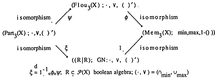
Figure 6.1. Summary of isomorphisms among ((R|R); \text{GN}) , \text{Mem}_3(X) , \text{Flou}_3(X) , \text{Part}_3(X) .
