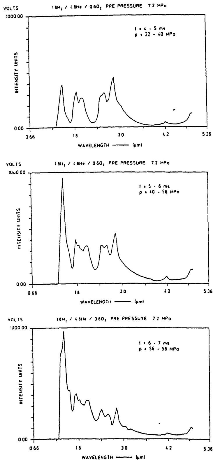
Fig. 15. Series of IR spectra from \text{H}_2/\text{O}_2 combustion; helium diluent
