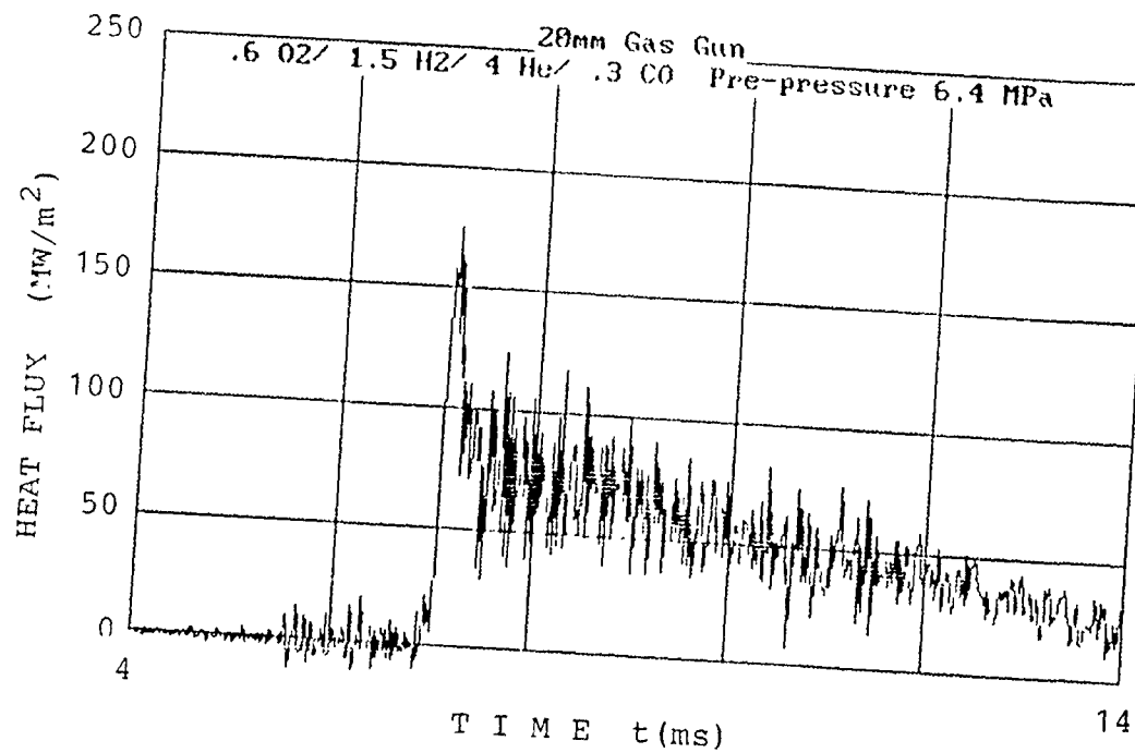
Fig. 57. Heat flux vs time at location M5A (Gas mixture: 0.6 \text{ O}_2 + 1.5 \text{ H}_2 + 4 \text{ He} + 0.3 \text{ CO} ; prepressure: 6.4 MPa)
