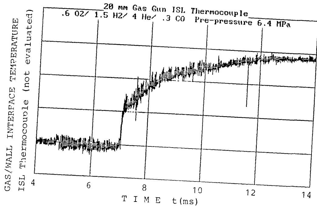
Fig. 56. ISL thermocouple readings at location M5A (not evaluated) (Gas mixture: 0.6 \text{ O}_2 + 1.5 \text{ H}_2 + 4 \text{ He} + 0.3 \text{ CO} ; prepressure: 6.4 MPa)
