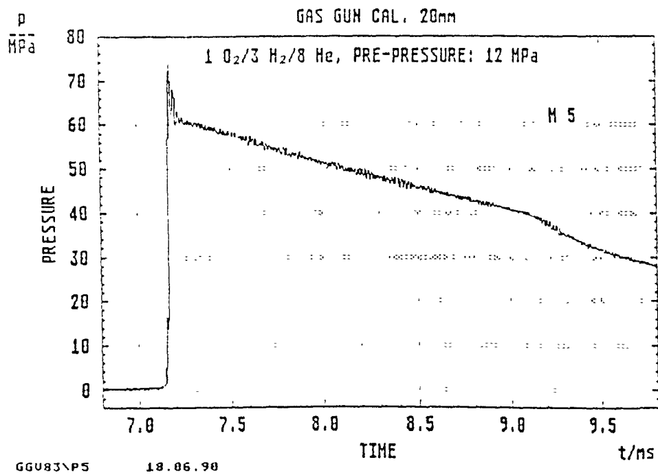
Fig. 31. Velocity at R = 5 mm and pressure at M5 (Gas mixture: O 2 + 3 H 2 + 8 He; prepressure: 12 MPa)
