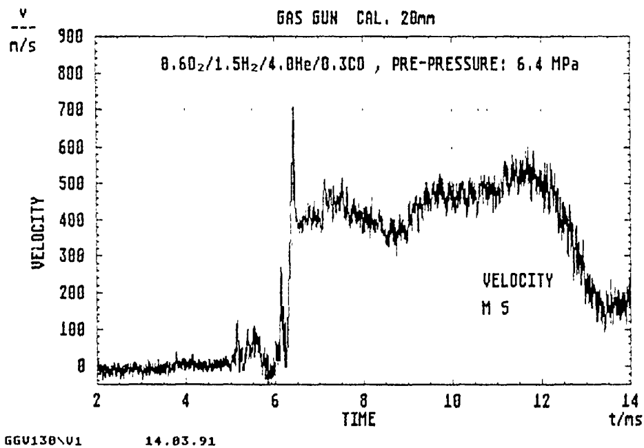
Fig. 61. Velocity vs time at location M5 and R = 8.5 mm (Gas mixture: 0.6 O 2 + 1.5 H 2 + 4 He + 0.3 CO; prepressure: 6.4 MPa)
