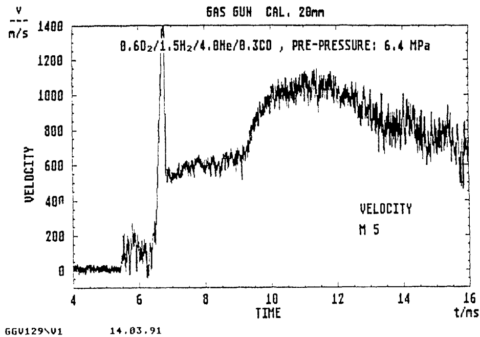
Fig. 60. Velocity vs time at location M5 and R = 7.5 mm (Gas mixture: 0.6 O 2 + 1.5 H 2 + 4 He + 0.3 CO; prepressure: 6.4 MPa)
