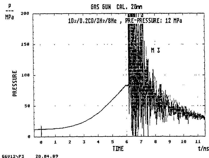
Fig. 12. Pressure vs time at location M3 ( \text{O}_2 + 3 \text{ H}_2 + 8 \text{ He} + 0.2 \text{ CO} )
