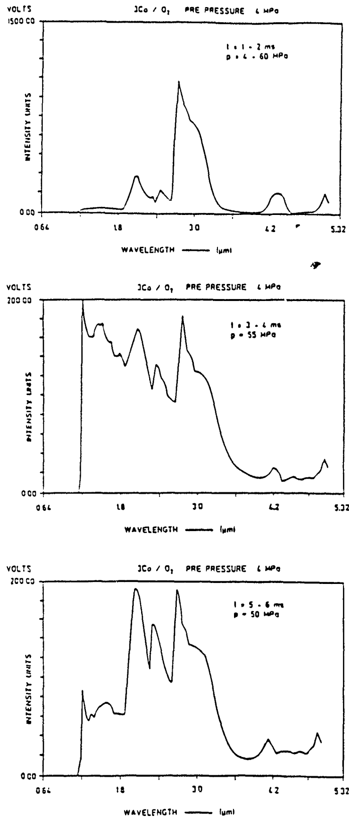
Fig. 16. Series of IR spectra from \text{CO}/\text{O}_2 combustion
