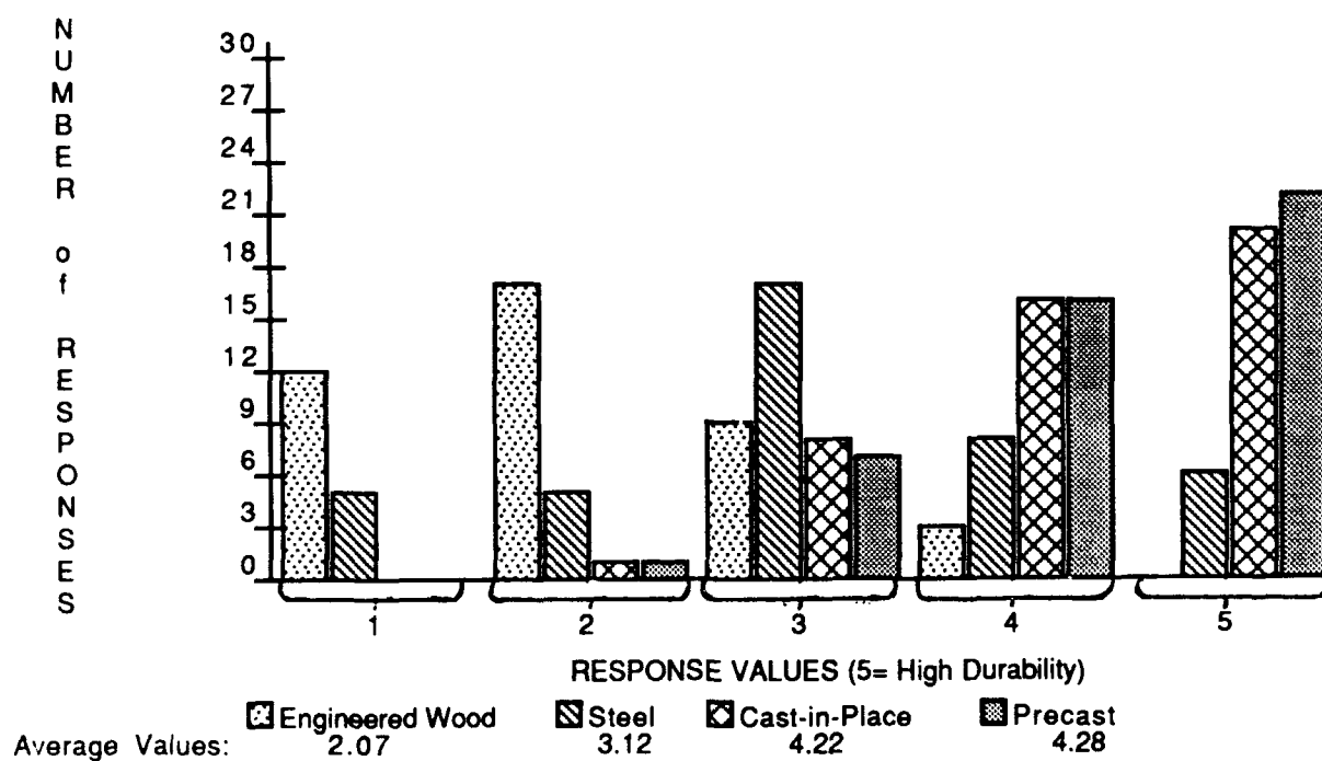
Figure 7. Comparison of Material Durability
