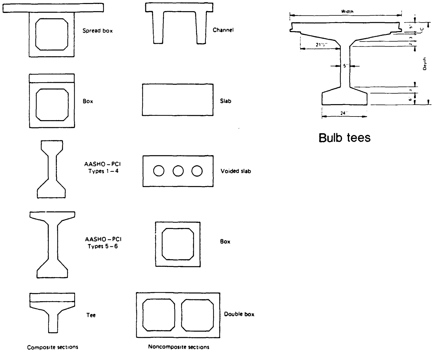
Figure 2. Precast Concrete Element Shapes (Heins and Lawrie, 1984; Prestressed Concrete Institute, 1980)
