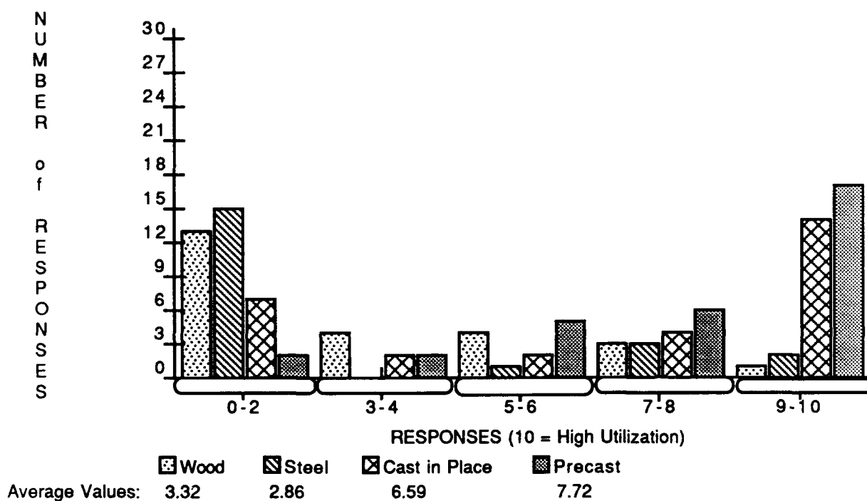
Figure 5. Utilization of Materials in the Bridge Deck
