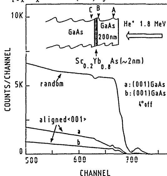
Fig. 3 : RBS/channeling spectra from buried \text{GaAs}/(2\text{nm})\text{Sc}_{0.2}\text{Yb}_{0.8}\text{As}/\text{GaAs} heterostructures for (001) and (001) 4^\circ\text{off} substrates. The two random spectra are quite similar.
