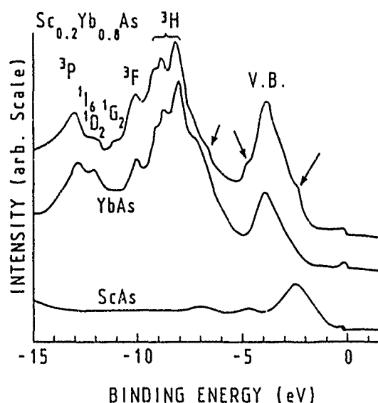
Fig. 2 : UPS spectra taken on \text{Sc}_{0.2}\text{Yb}_{0.8}\text{As} , YbAs and ScAs epitaxial surfaces with \text{HeII}\alpha .
