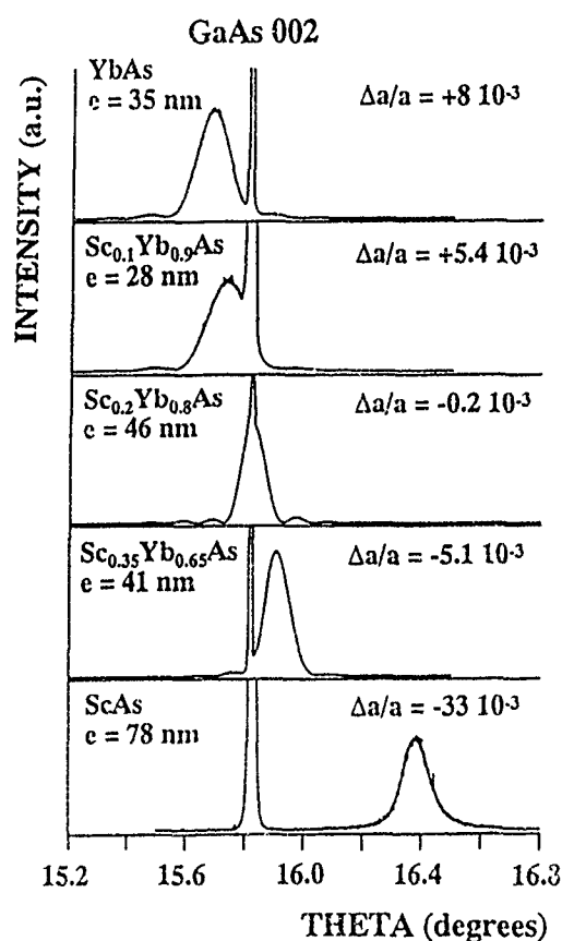
Fig. 1 : X-ray \text{CuK}\alpha_1 patterns of the 002 reflections of various \text{Sc}_{1-x}\text{Yb}_x\text{As}/\text{GaAs}(001) systems.
