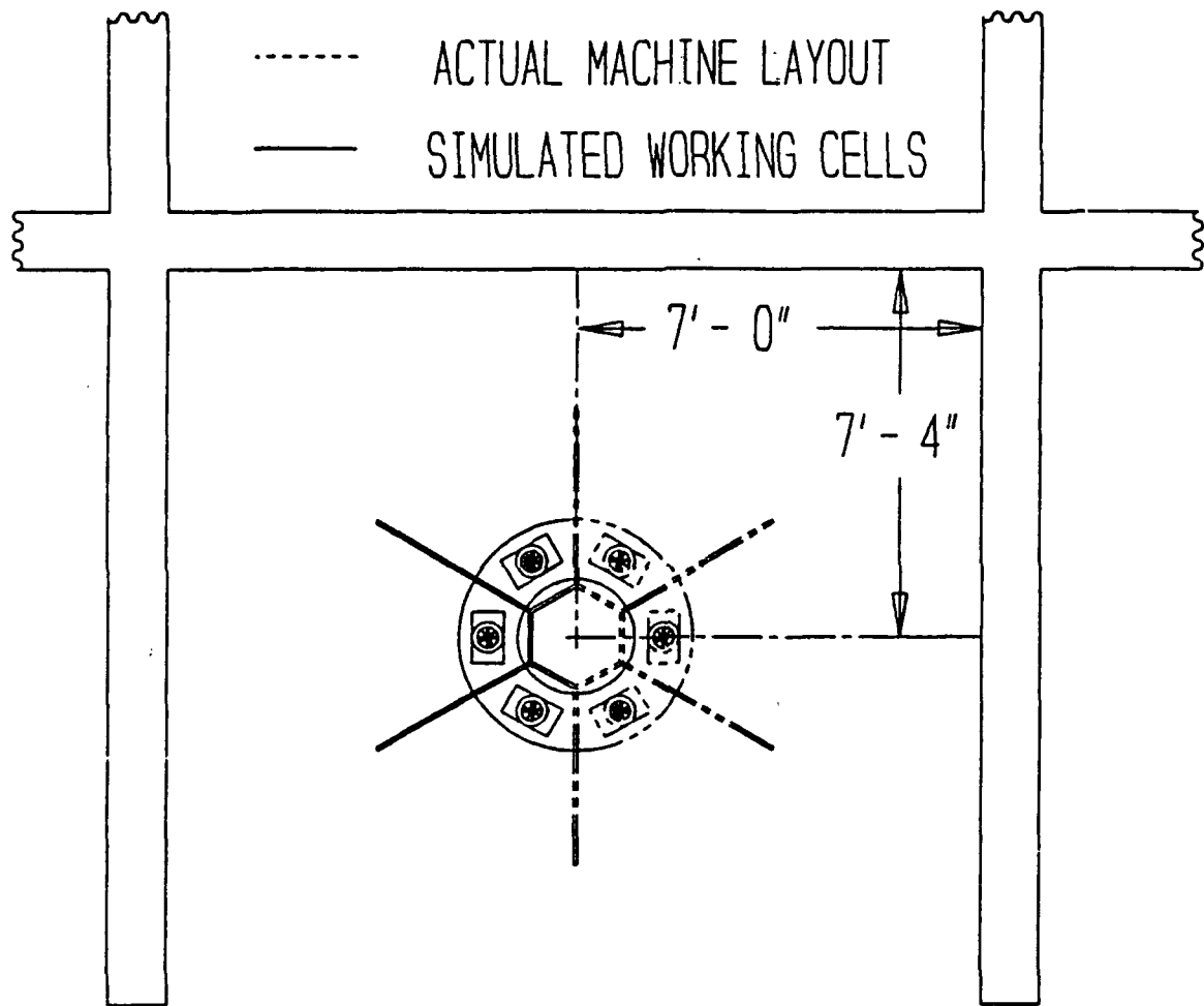
Figure 2 SIMULATED APE 2245 SET UP
