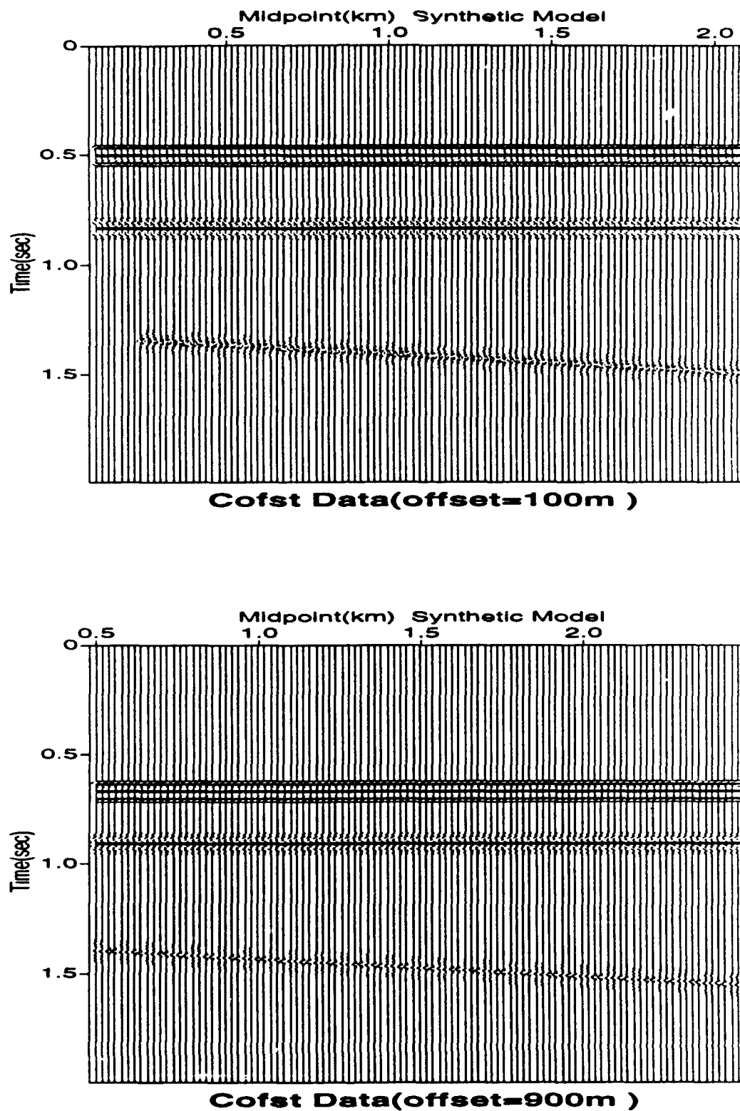
FIG. 4. Input synthetic data of two offsets for the model in Figure 3.
