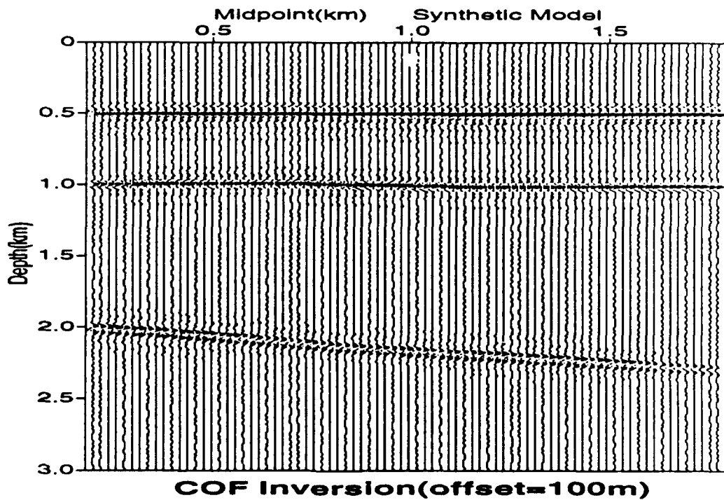
FIG. 5. Inversion outputs. The upper uses the exact model; the lower uses the model obtained from velocity analysis.
