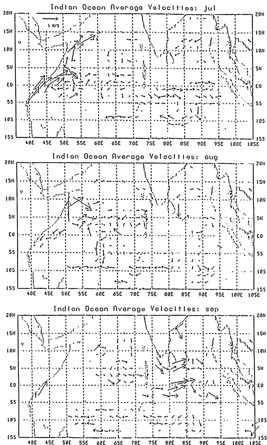
Figure 5.15 Drifting buoy-derived near-surface currents in the Indian Ocean during July, August, and September. (Molinari et al. , 1990).
