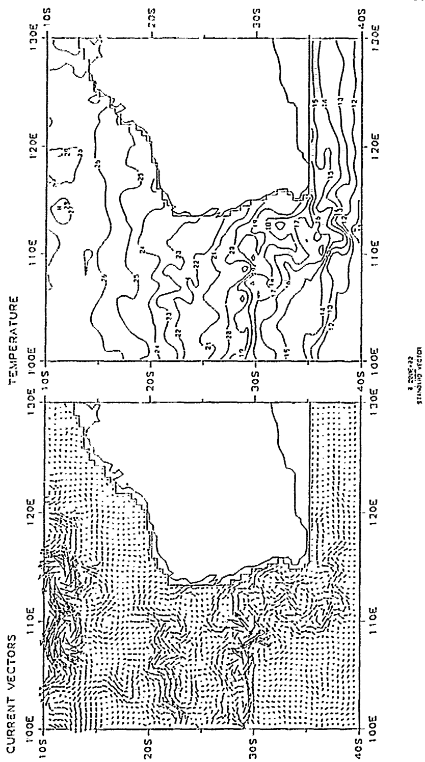
Figure 4.45 Year 4 West Australian current vector and temperature plots at 37.5 m in October.
