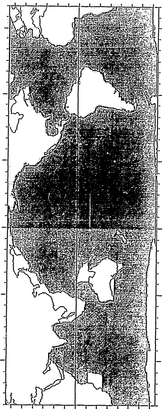
Figure 2.3 The global ocean model domain at 12.5 m. The only islands are Australia/New Guinea, New Zealand, Antarctica. Other islands have been shoaled or attached to continental land masses, and marginal seas have been filled in.
