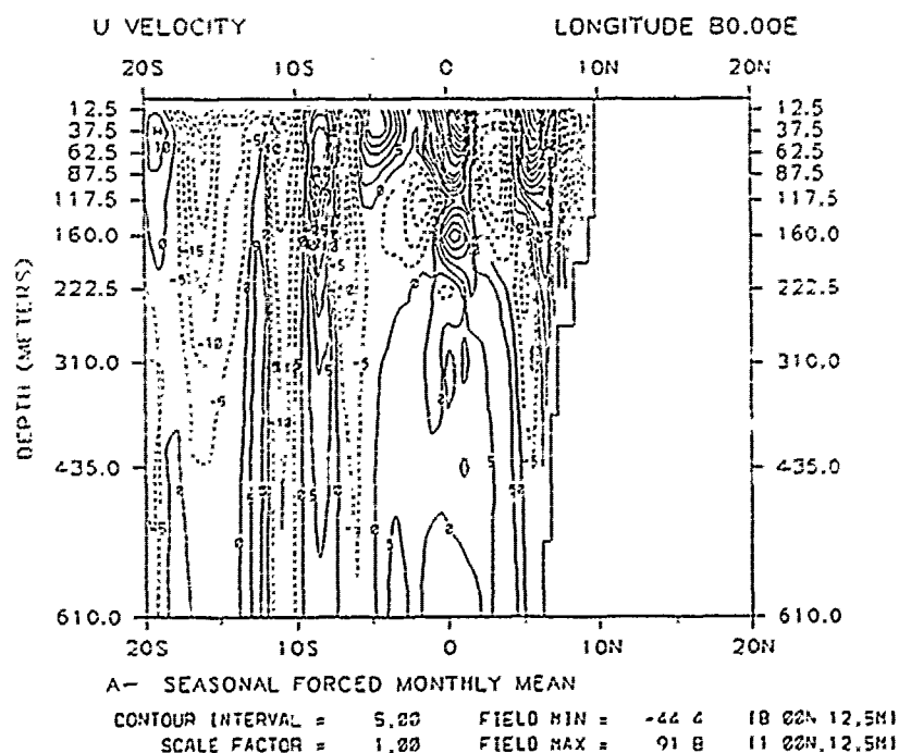
Figure 4.27 Monthly mean zonal currents at 80°E during Year 4. (a) September and (b) October.
