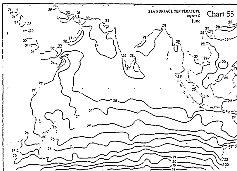
Figure 5.6 Comparison of June T at 12.5 m with climatology. (a) Monthly mean temperature in the model, and (b) Hastenrath and Lamb (1979) sea surface temperature.
