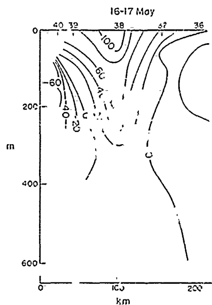
FIG. 11. Alongshore speed in depth range 0-600 m., measured along a section normal to the coast at 5°N (section 0 in Fig. 2) during 16-17 May 1979 (from LEETMAA et al. , 1982).
