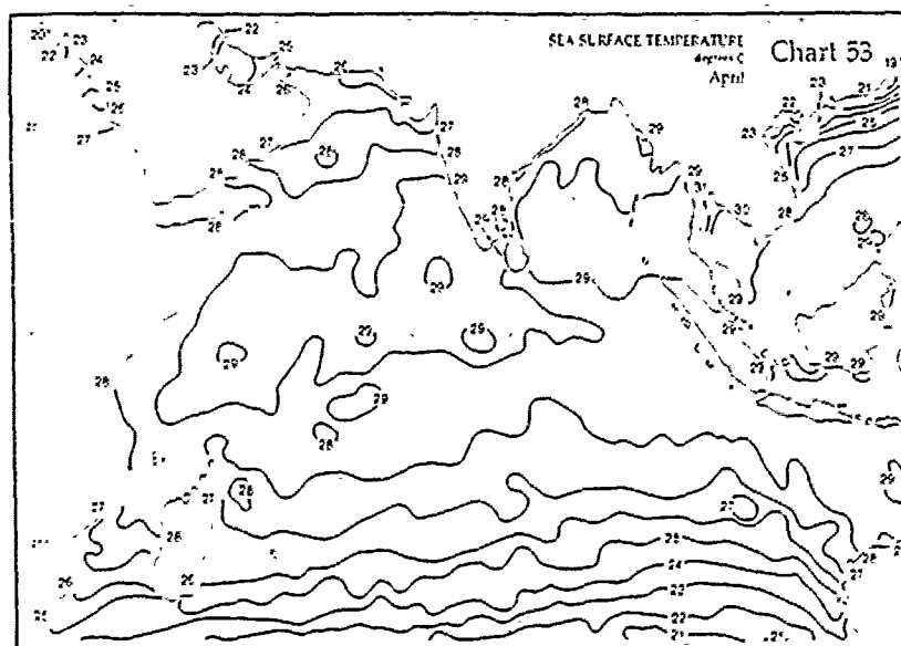
Figure 5.4 Comparison of April T at 12.5 m with climatology. (a) Monthly mean temperature in the model, and (b) Hastenrath and Lamb (1979) sea surface temperature.
