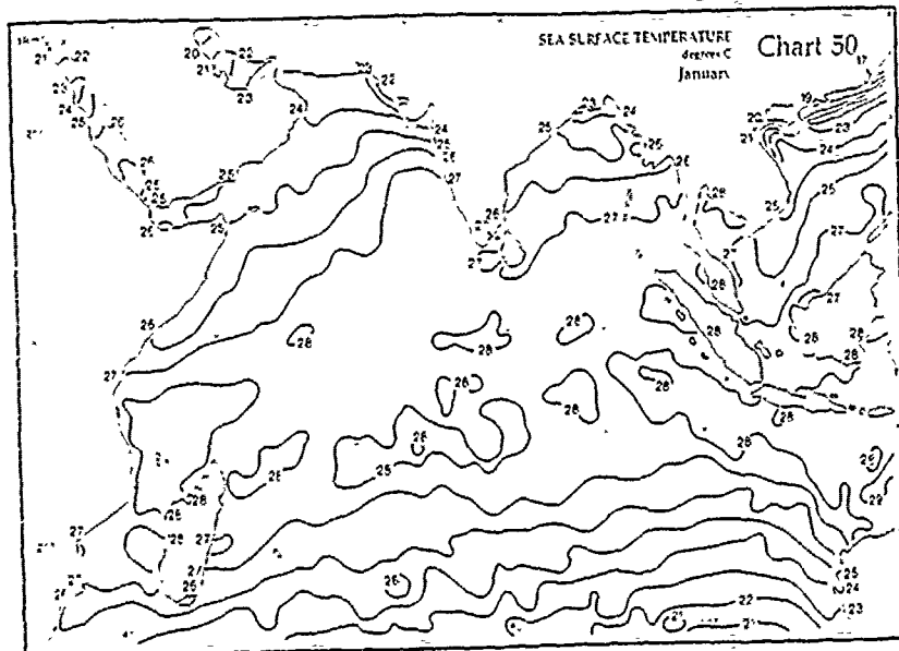
Figure 5.1 Comparison of January T at 12.5 m with climatology. (a) Monthly mean temperature in the model, and (b) Hastenrath and Lamb (1979) sea surface temperature.
