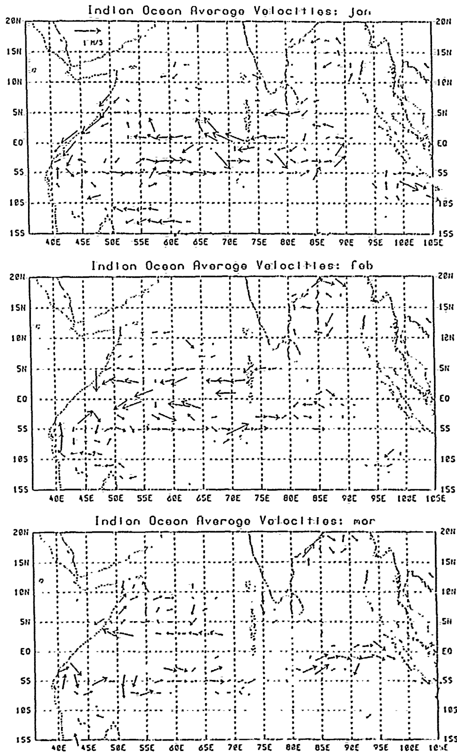
Figure 5.13 Drifting buoy-derived near-surface currents in the Indian Ocean during January, February, and March. (Molinari et al. , 1990).
