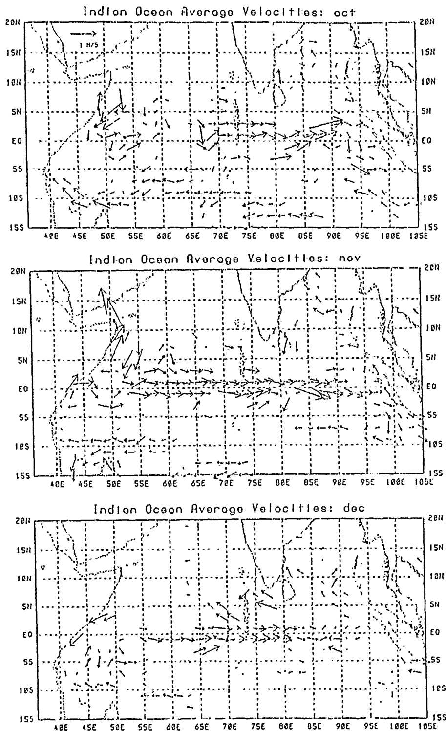
Figure 5.16 Drifting buoy-derived near-surface currents in the Indian Ocean during October, November, and December. (Molinari et al. , 1990).
