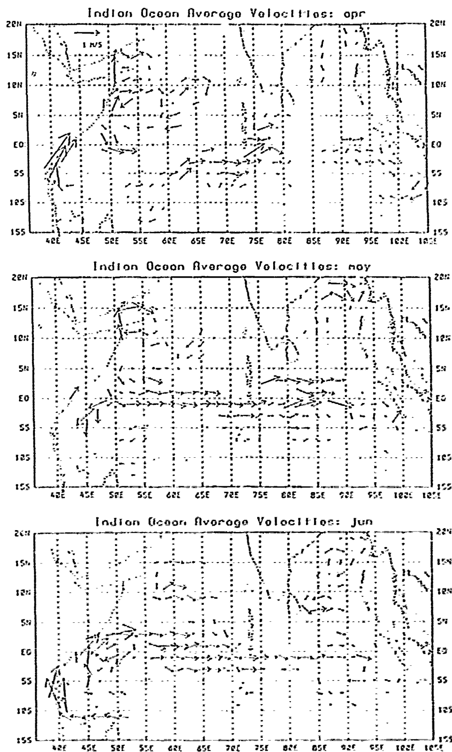
Figure 5.14 Drifting buoy-derived near-surface currents in the Indian Ocean during April, May, and June. (Molinari et al. , 1990).
