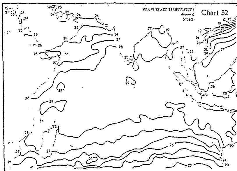
Figure 5.3 Comparison of March T at 12.5 m with climatology. (a) Monthly mean temperature in the model, and (b) Hastenrath and Lamb (1979) sea surface temperature.
