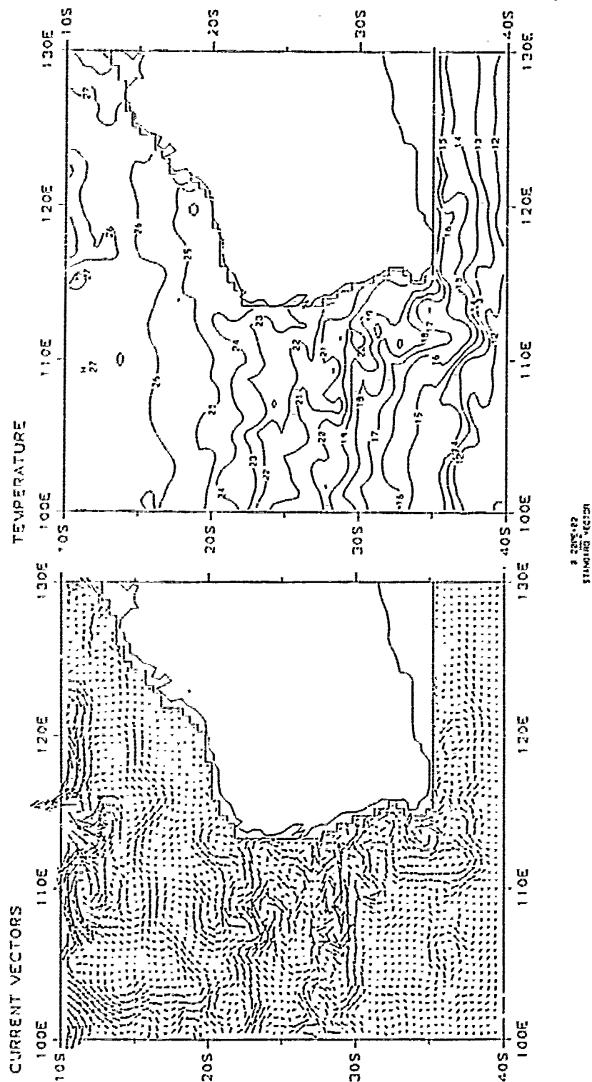
Figure 4.44 Year 4 West Australian current vector and temperature plots at 37.5 m in September.
