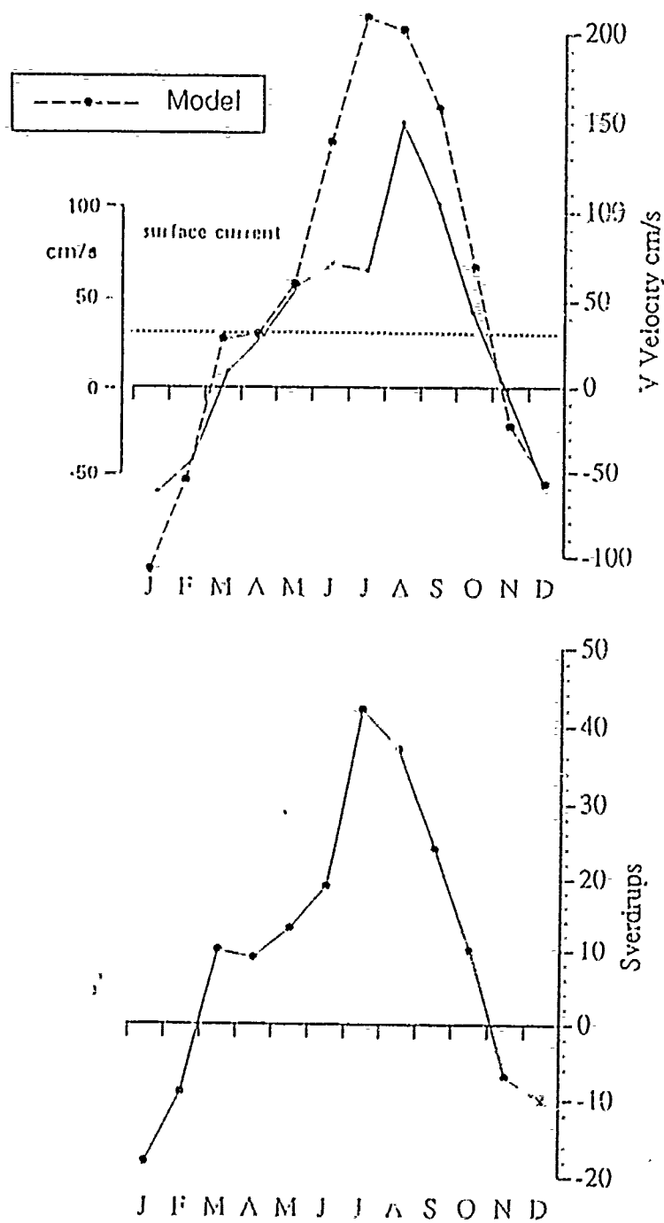
Figure 4.55 Seasonal cycle of Somali Current surface flow at 5°N. (a) Historical alongshore flow (solid line, after Quadfasel and Schott, 1983), and maximum velocity (dashed line) of the top-level (12.5-m) v velocity during Year 4, from sections at 48°E-52°E. (b). Mass transport of the prevailing flow in the 5°N, 48-52°E, 0-610 m plots.
