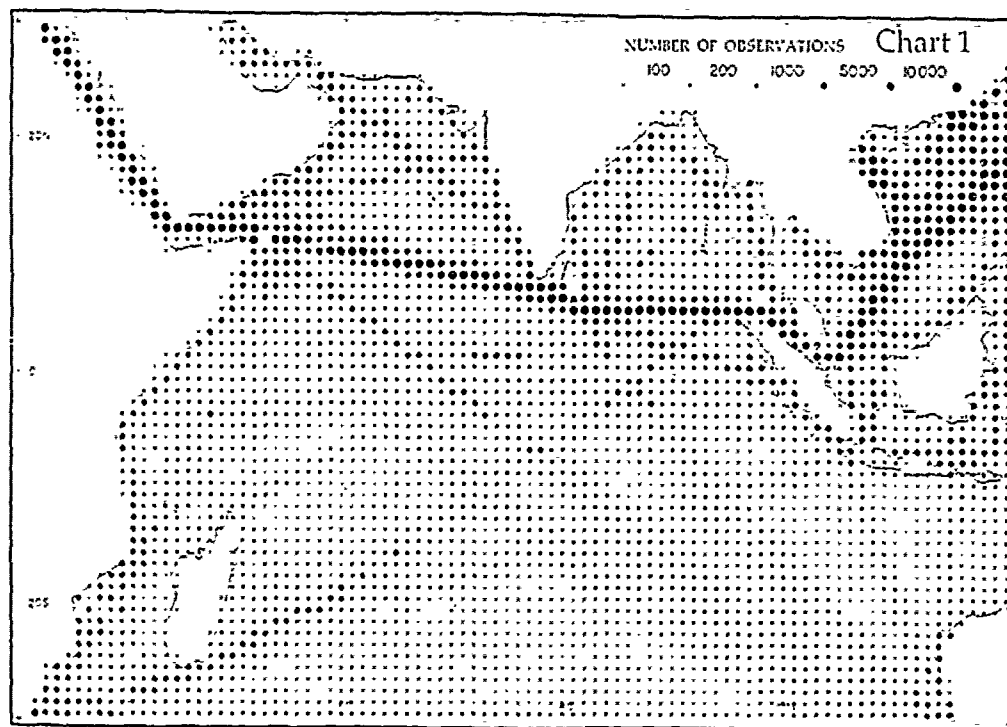
Figure 1.2 Density and distribution of Indian Ocean observations. (a) Surface and subsurface observations from Levitus (1982) (b) Surface observations from Hastenrath and Lamb (1979).
