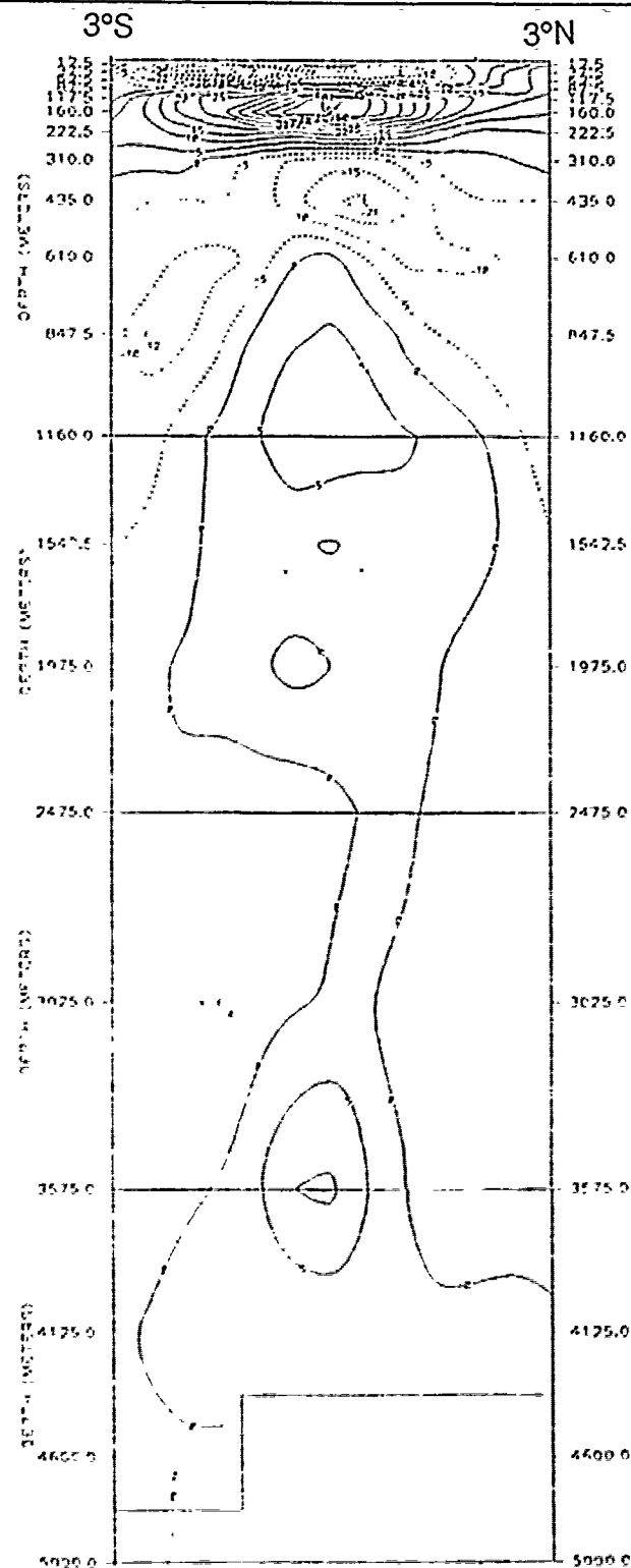
Figure 4.32 Deep current structure in the equatorial Indian Ocean. This plot of zonal velocity ( \text{cm s}^{-1} ) at 85^\circ\text{E} on 19 March of Year 4 illustrates the complex deep current structure in the equatorial region.
