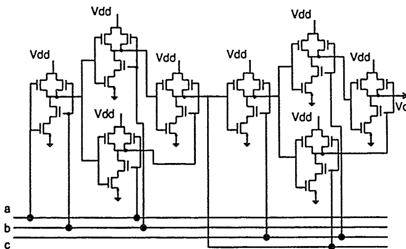
Figure 68. Circuit implementation of the full adder.
