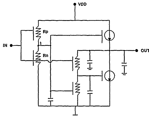
Figure 73. TODO model for the circuit shown in Figure 70.
