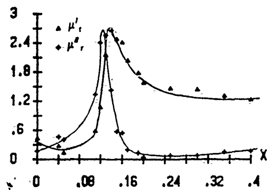
Fig. 9: Dependence of \mu_i on Co content
