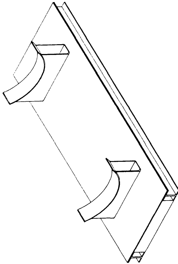
Figure 8. Muffler Mount.
