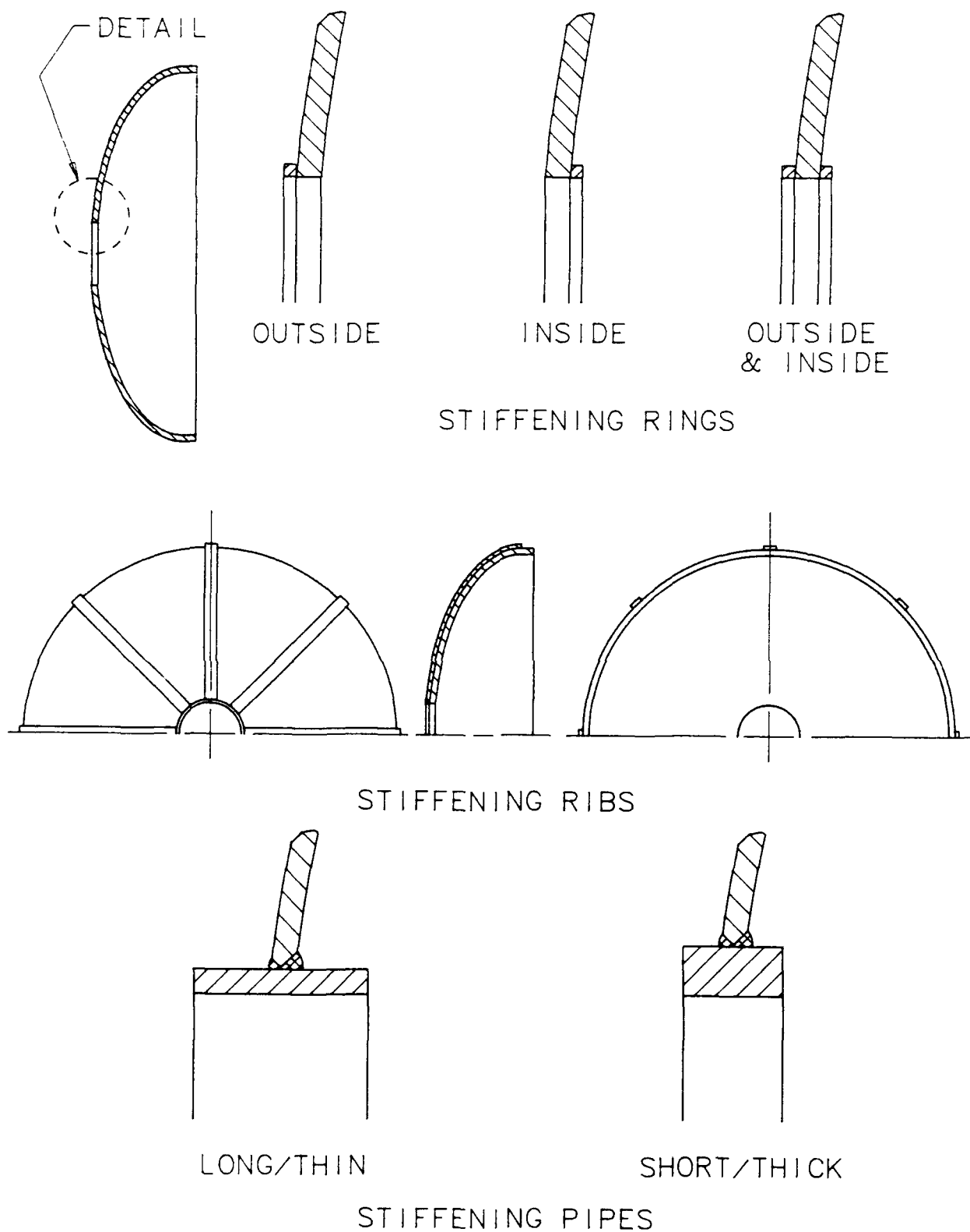
Figure 3. Hole Stiffeners.
