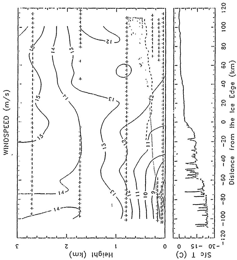
Figure 10. Cross section of wind speed, perpendicular to the ice edge.
