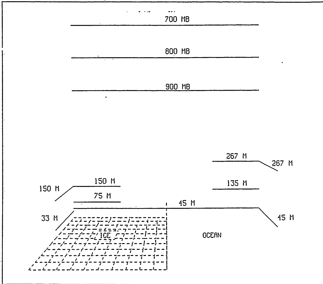
Figure 3. Flight pattern schematic for CEAREX flight
