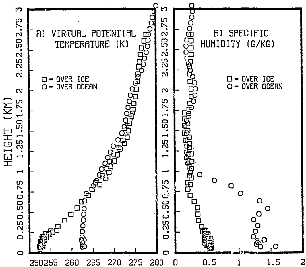
Figure 4. Composite profiles of a) virtual potential temperature and b) specific humidity
