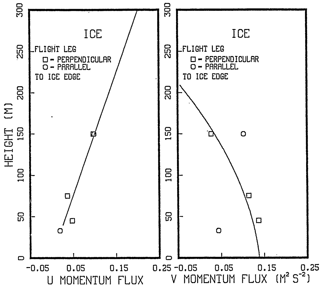
Figure 18. Vertical turbulent momentum flux over the ice
