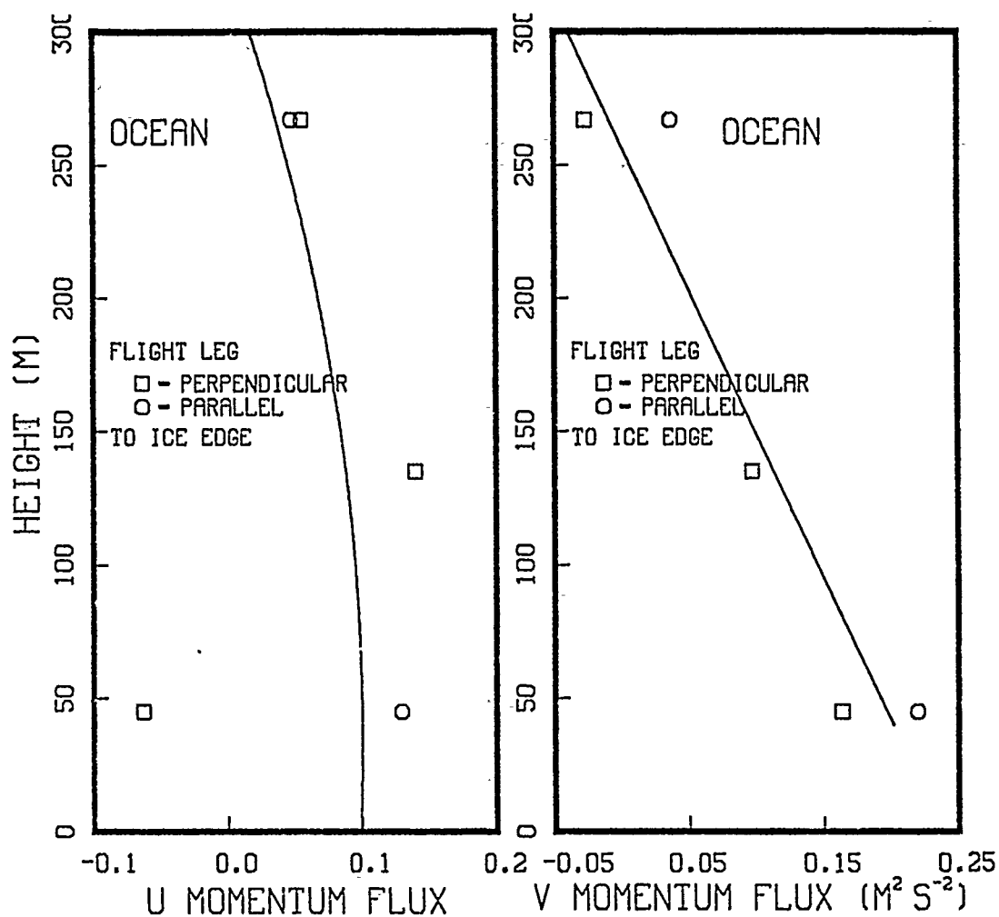
Figure 19. Vertical turbulent momentum flux over the ocean
