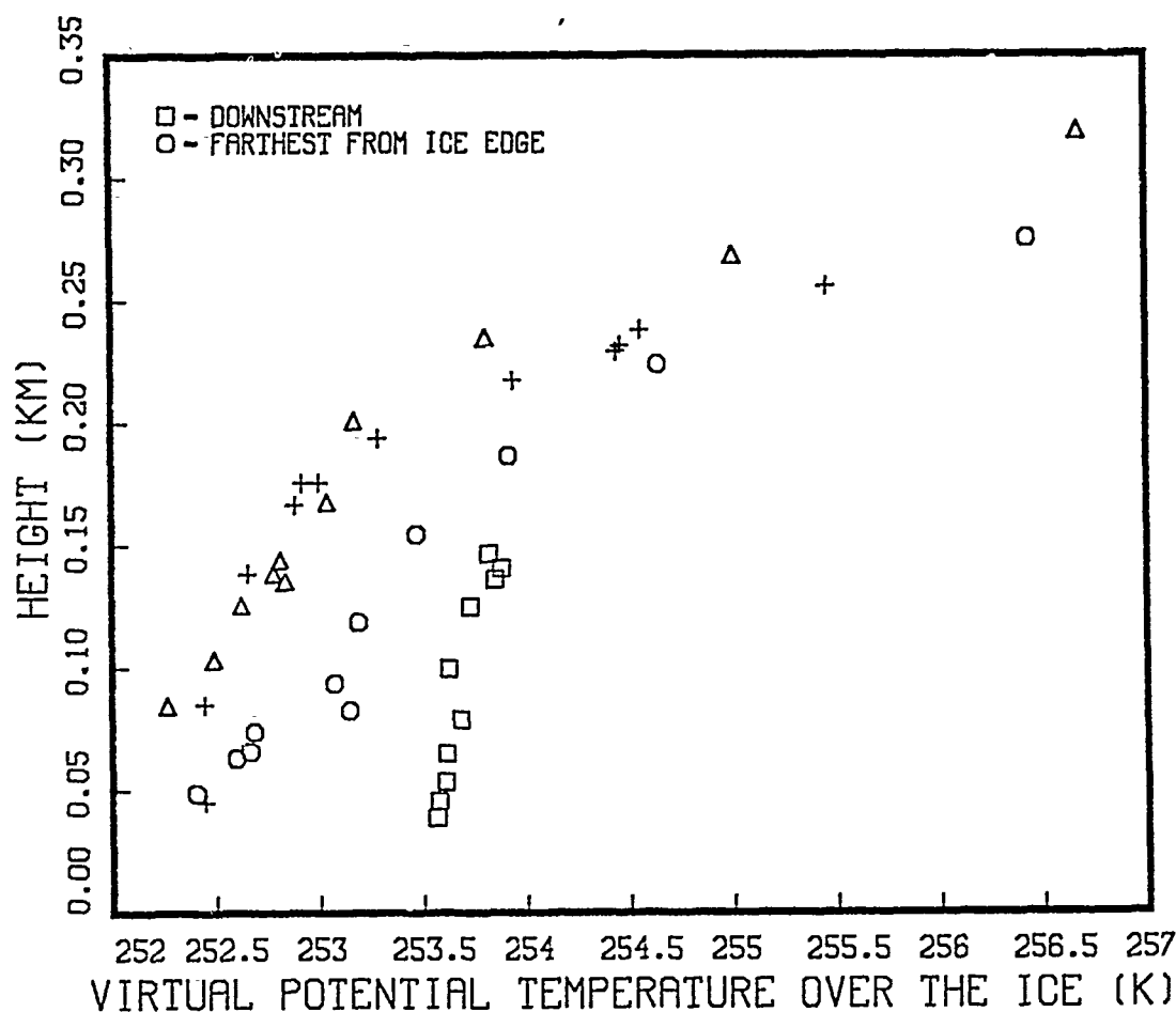
Figure 5. Profiles of virtual potential temperature over ice
