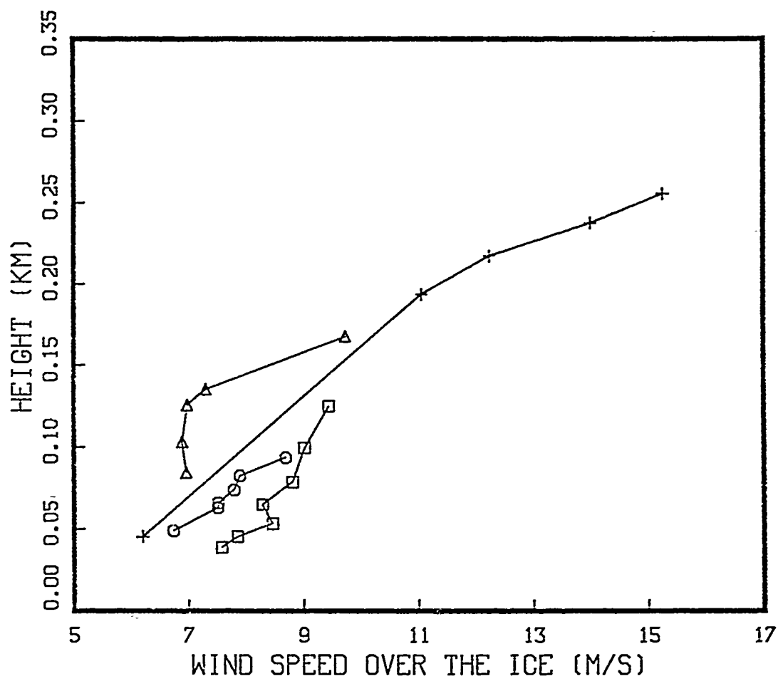
Figure 7. Profiles of wind speed over ice
