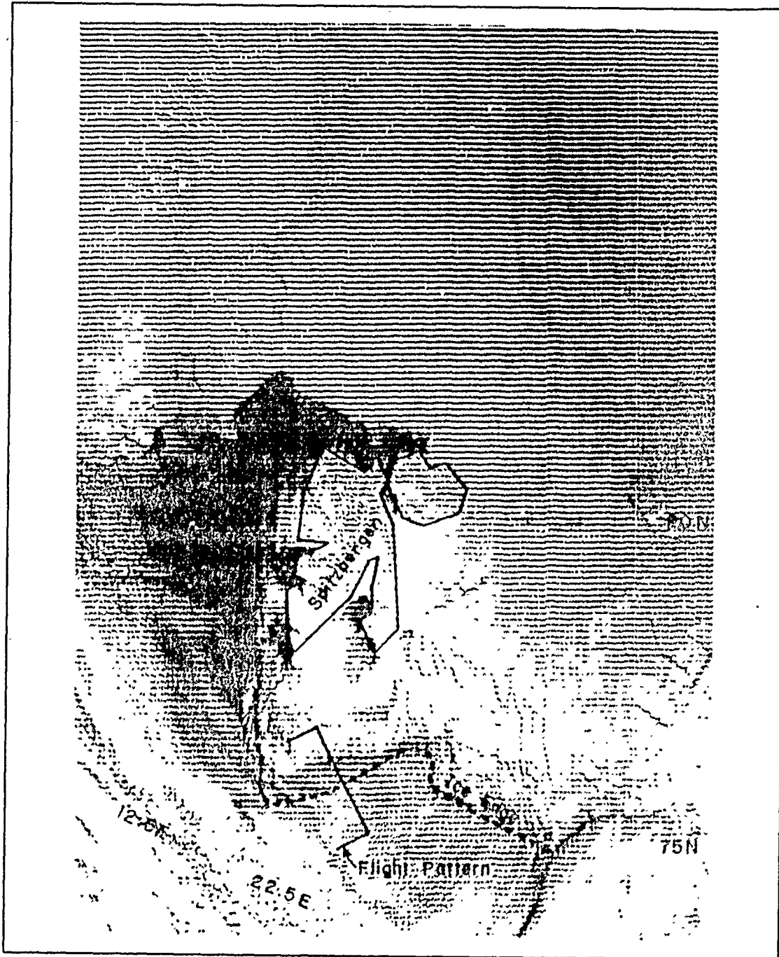
Figure 2. NOAA-10 IR imagery of 1038 UTC 24 March 1989
