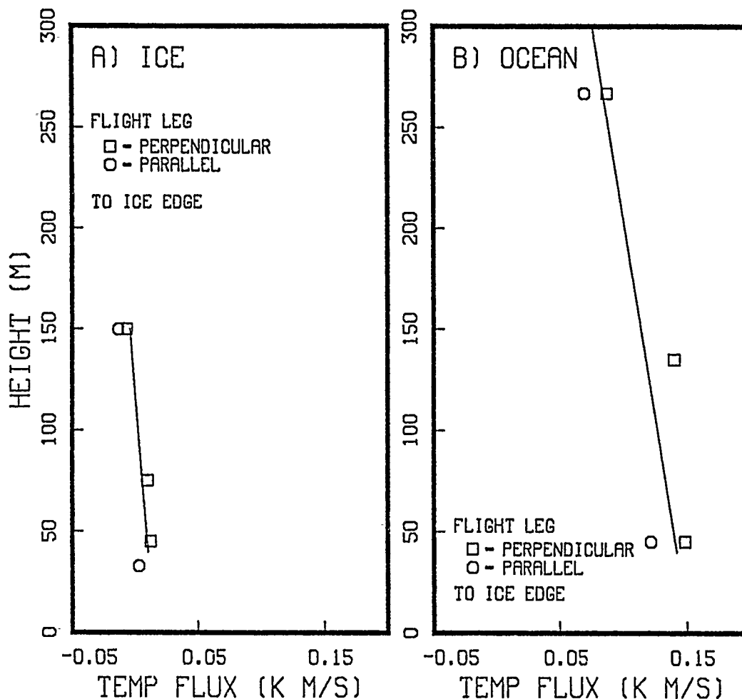
Figure 16. Vertical turbulent heat flux
