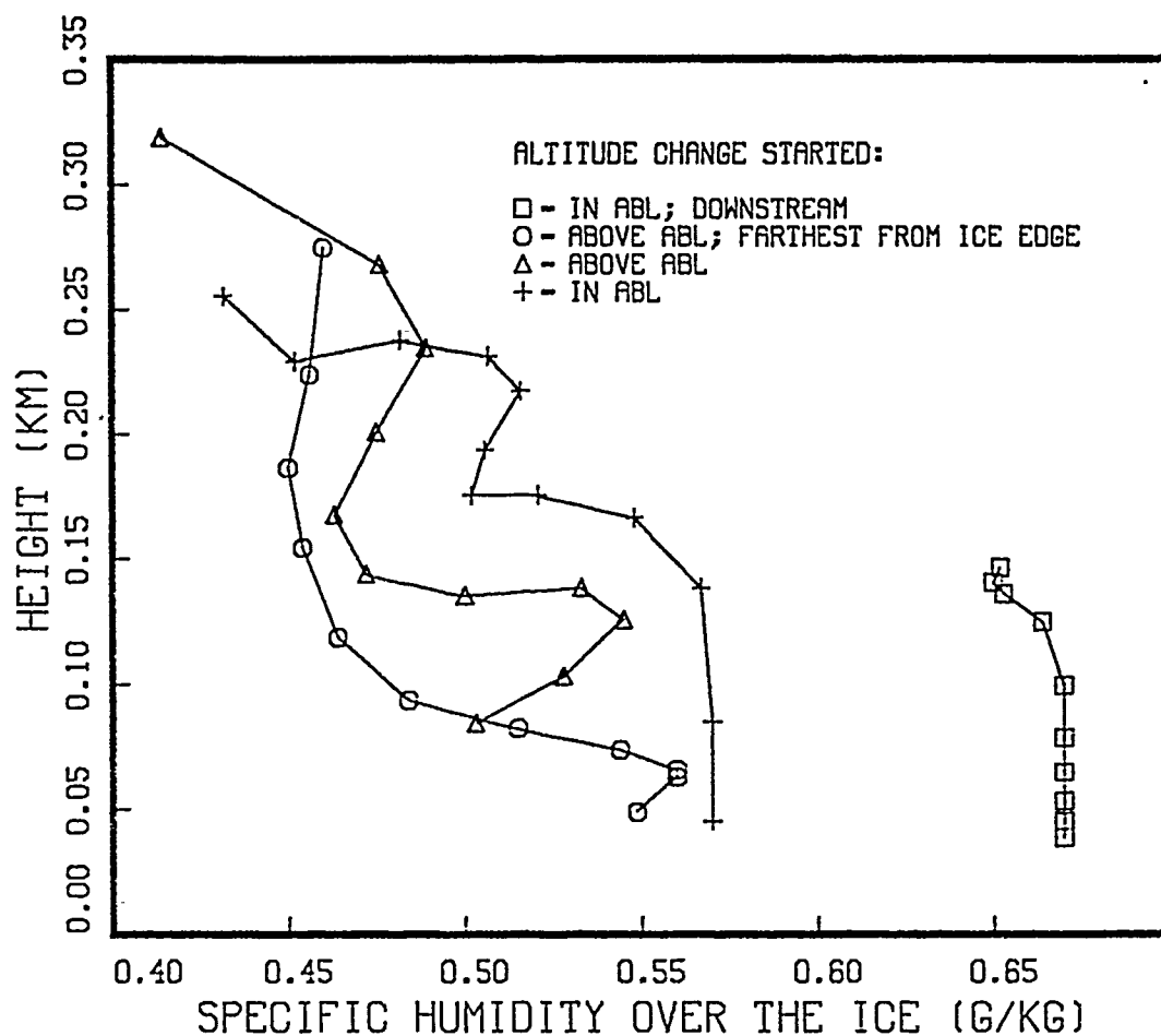
Figure 6. Profiles of specific humidity over ice
