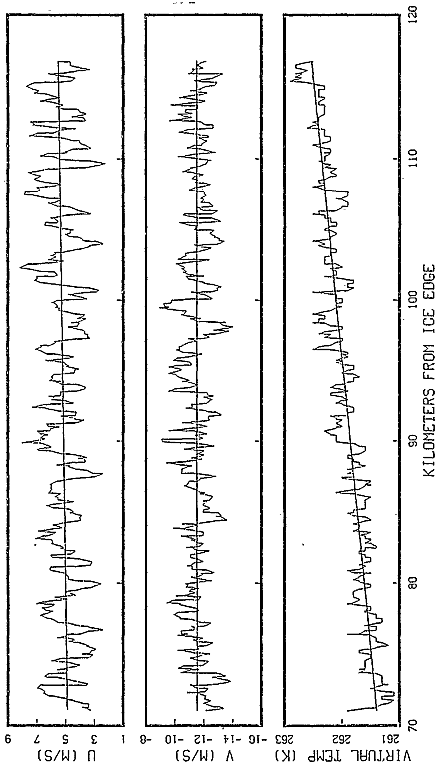
Figure 12. u, v and virtual temperature spatial series: from the 45 meter flight leg over ocean.
