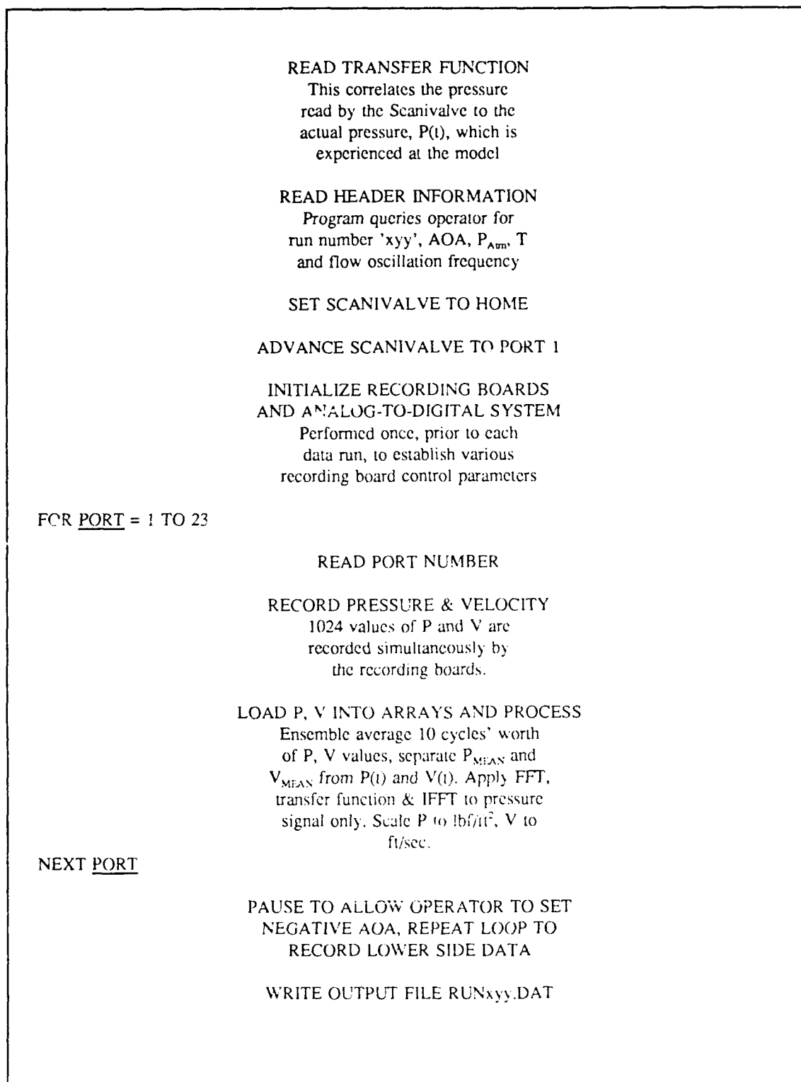
Figure 10. Data Acquisition Program Flow Chart.
