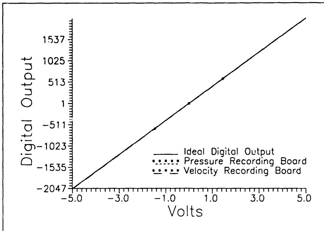
Figure 9. Data Acquisition Boards Calibration Results.
