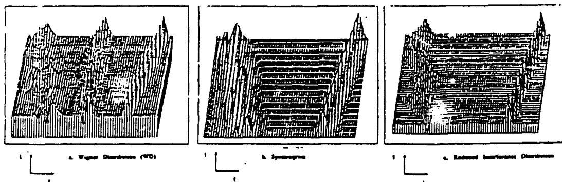
Figure 2. t-f distributions for a chirp plus FM signal: a. WD, b. spectrogram, c. RID
