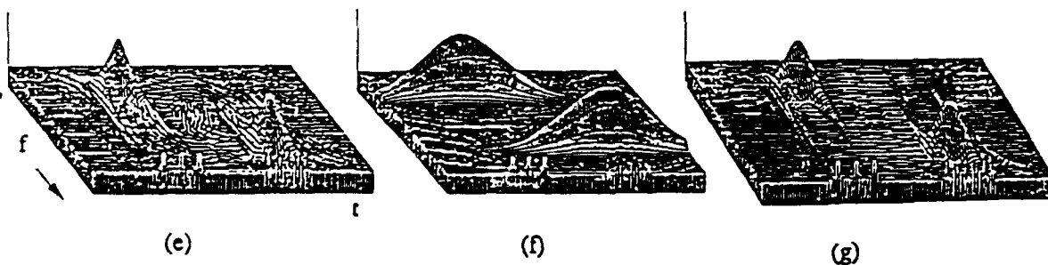
Figure 1e.-1g. t-f distributions for two sinusoids : e. WD, f. spectrogram, g. RID
