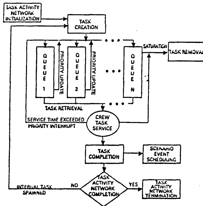
FIGURE 2. CTMEM CREW TASK PROCESSING MODEL STRUCTURE.
