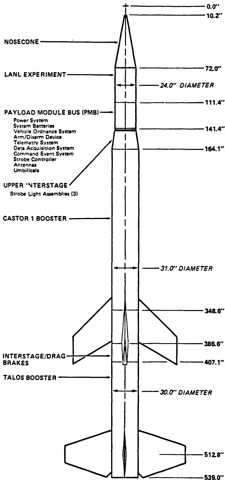
FIGURE 1-3 ZEST FLIGHT VEHICLE
