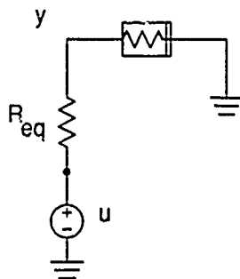
Figure 6: Thevenin equivalent circuit for one-dimensional nonlinear smoothing and segmentation network with step input.
