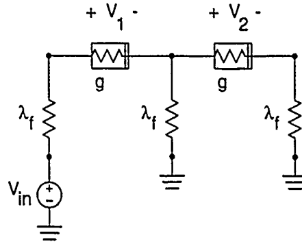
Figure 17: Three pixel example circuit. For the result shown in Figure 18, V_{in} = 2.5 \text{ V} , \lambda_s = 0.19 , \lambda_h = 1.0 \times 10^{-4} , \beta = 40 , \lambda_f = (1 - t)\lambda_{large} + \lambda_{small} , \lambda_{large} = 0.1 , \lambda_{small} = 1.0 \times 10^{-12} , and t was varied from 0 to 1.
