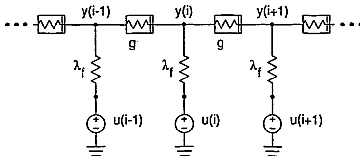
Figure 2: Resistor-With-Fuse (RWF) network topology.
