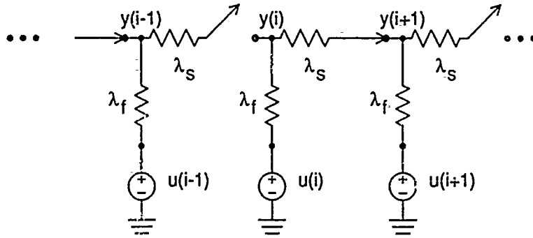
Figure 1: A simple smoothing network with switches. The vertical and horizontal resistors have conductances \lambda_f and \lambda_s , respectively.
