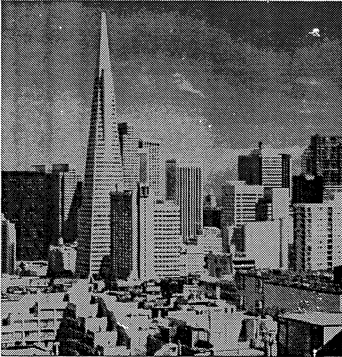
Figure 16: (a) Output produced by \lambda_f -continuation network. Here, the parameter values are \lambda_s = 1 \times 10^{-3} , \lambda_h = 2 \times 10^{-5} , \beta = 5 \times 10^4 , and \lambda_f = 1 , \lambda_f = 5 \times 10^{-4} , and \lambda_f = 1 \times 10^{-6} for Figures 16a, 16b, and 16c, respectively.
