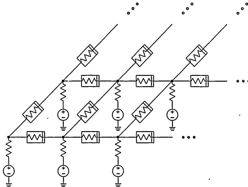
Figure 9: Two-Dimensional network topology.
