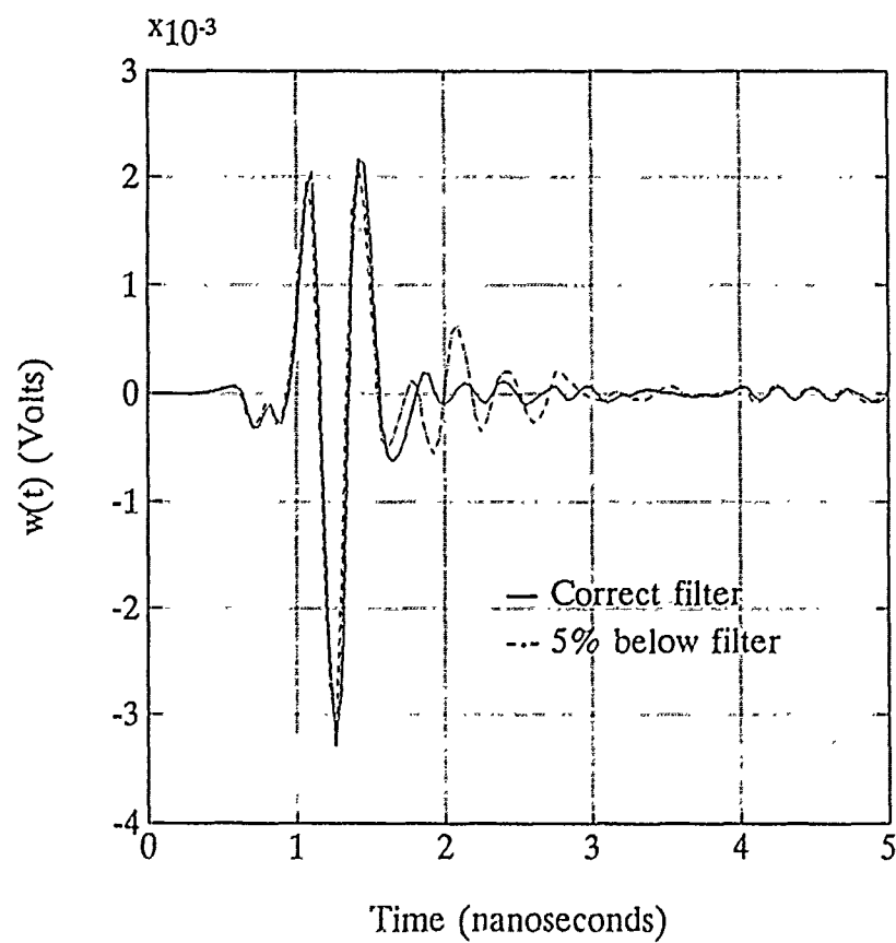
Figure 32. Measured thin-wire filter output, 30°
