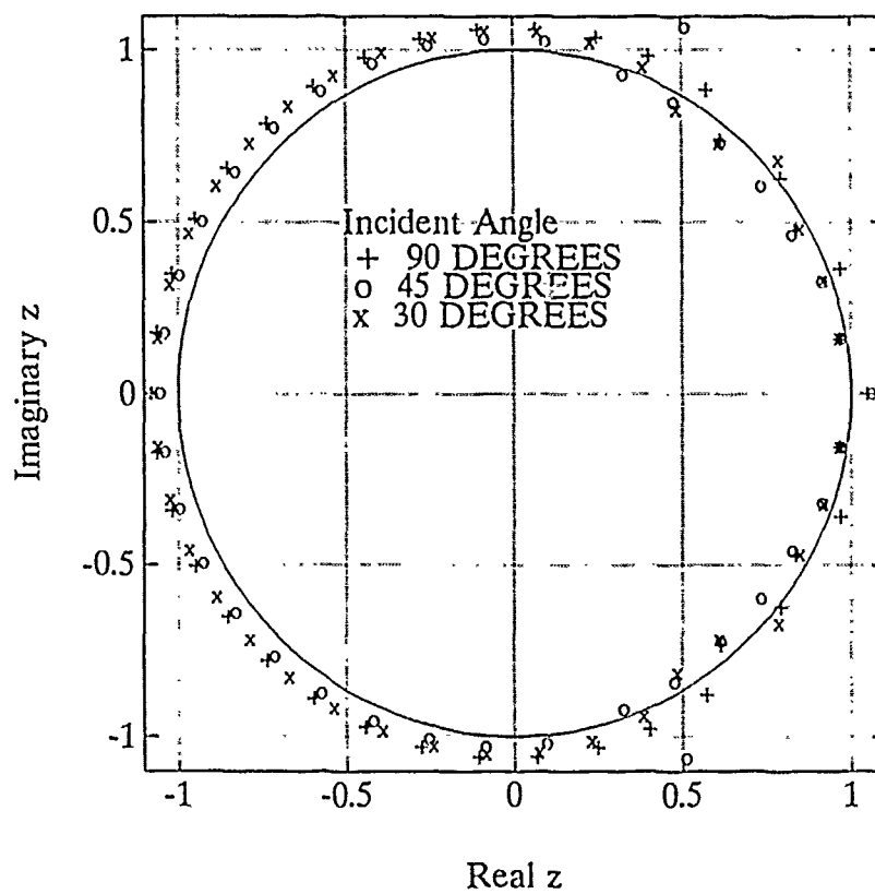
Figure 18. Extracted poles, measured thin-wire data [Ref. 6]
