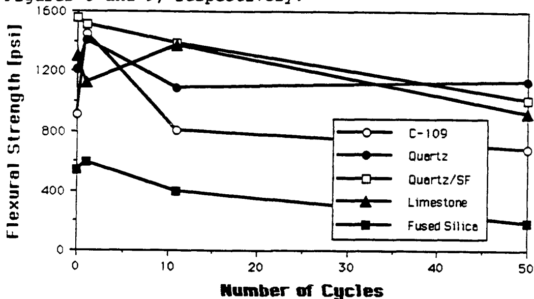
Figure 8. Flexural Strength Development with Heat Cycling
