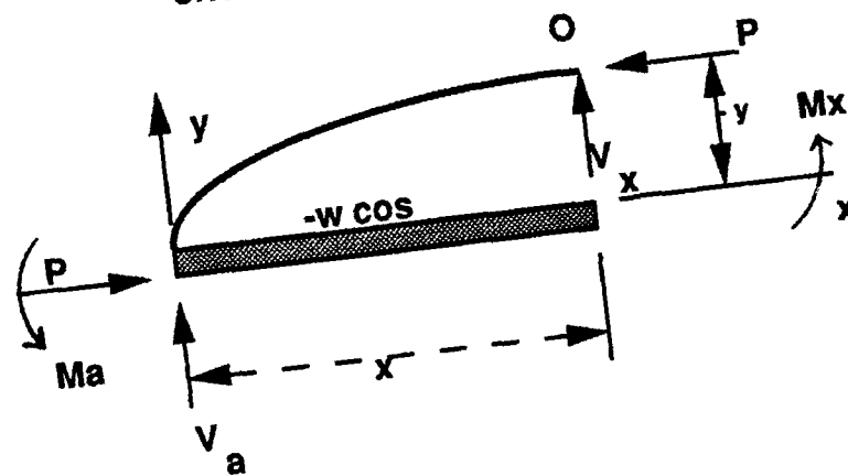
(b) free-body diagram
