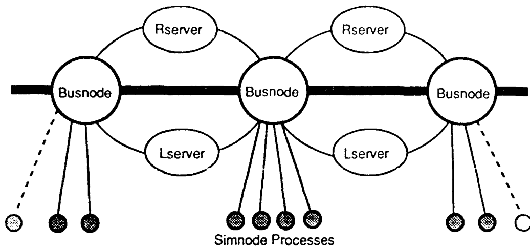
Figure 3. Simulation Model for Bus Topology Networks
