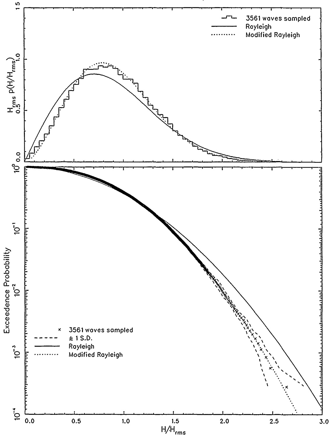
Figure 9. Probability and exceedence curves from a broad spectrum
