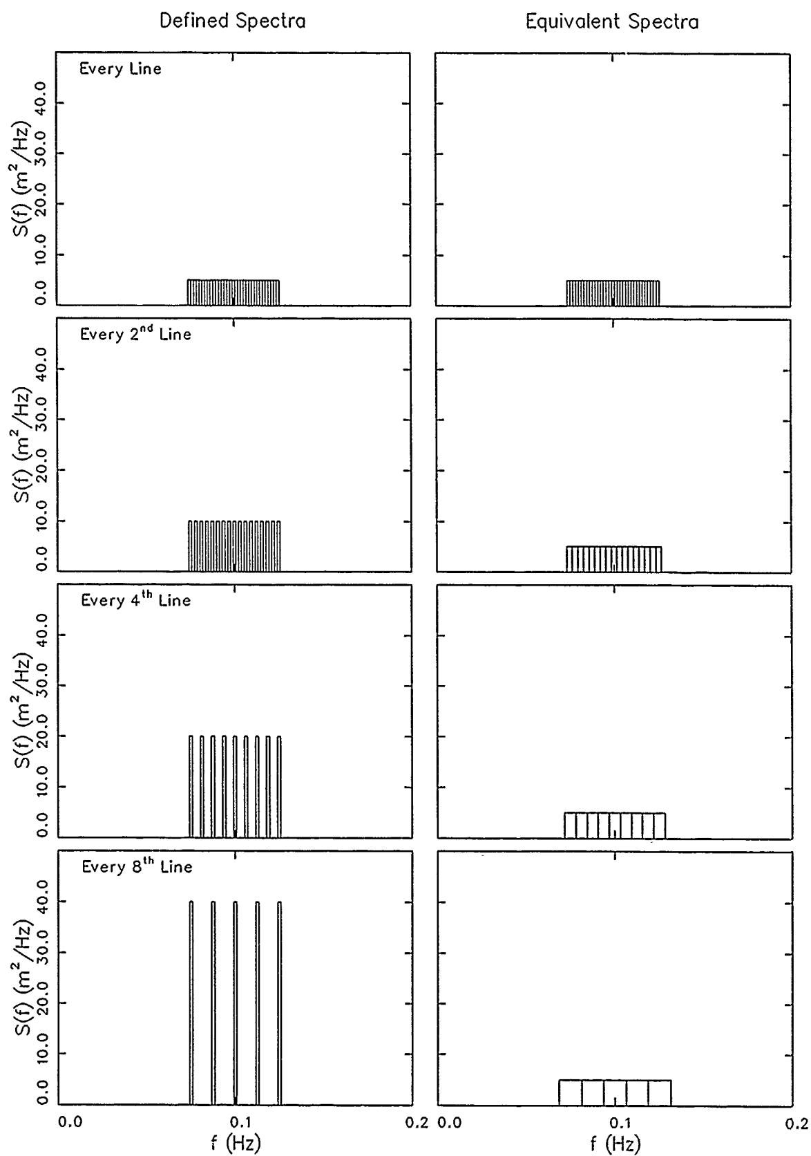
Figure 2. Examples of spectral line decimation
