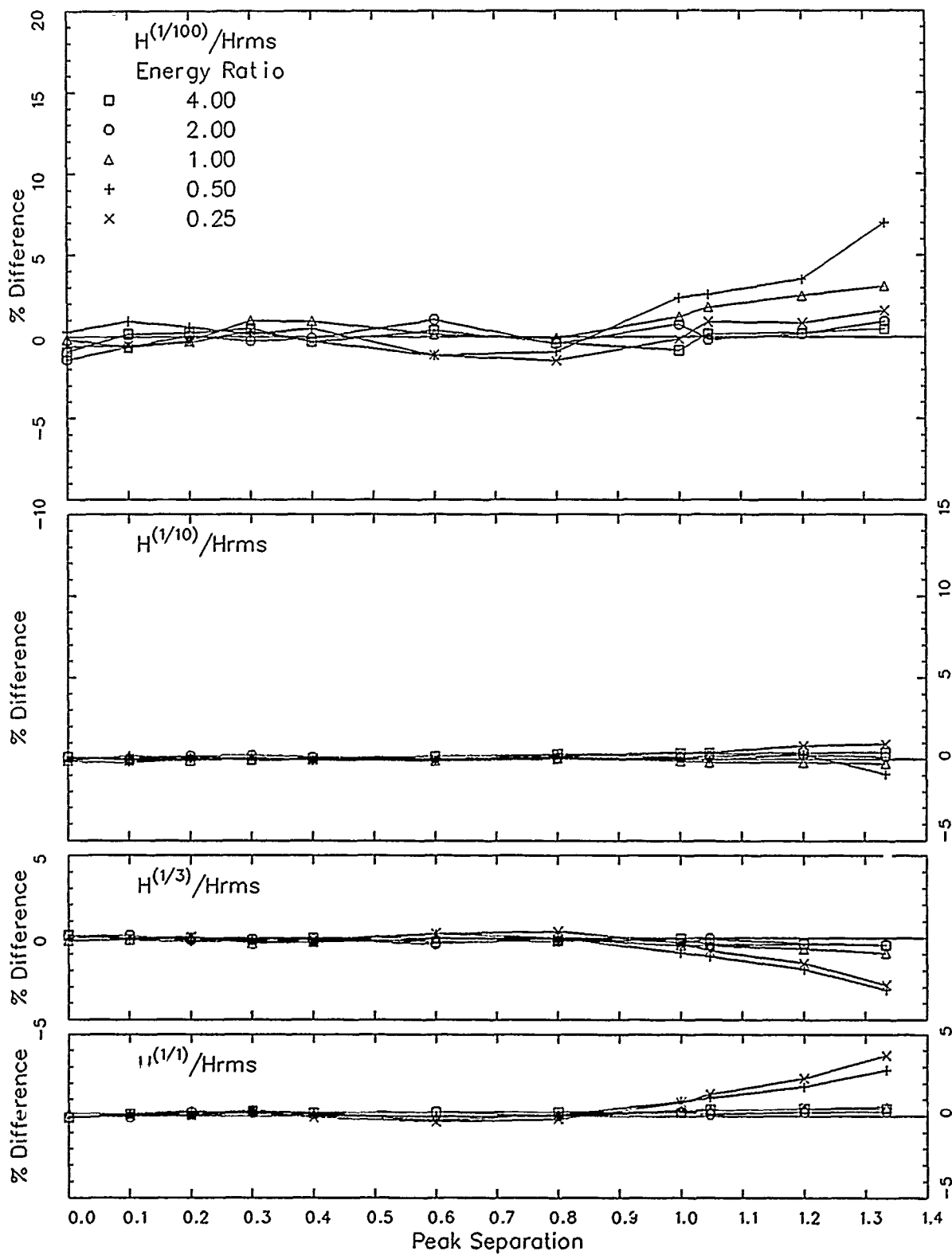
Figure 11. Wave height averages from bimodal spectra compared with Modified Rayleigh wave height averages
