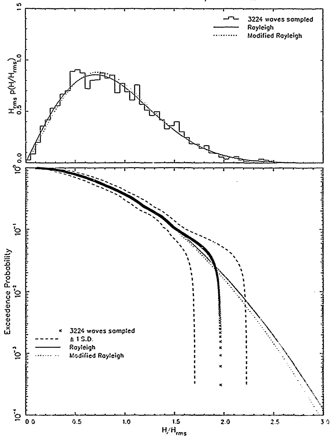
Figure 7. Probability and exceedence curves for 10 wave trains
