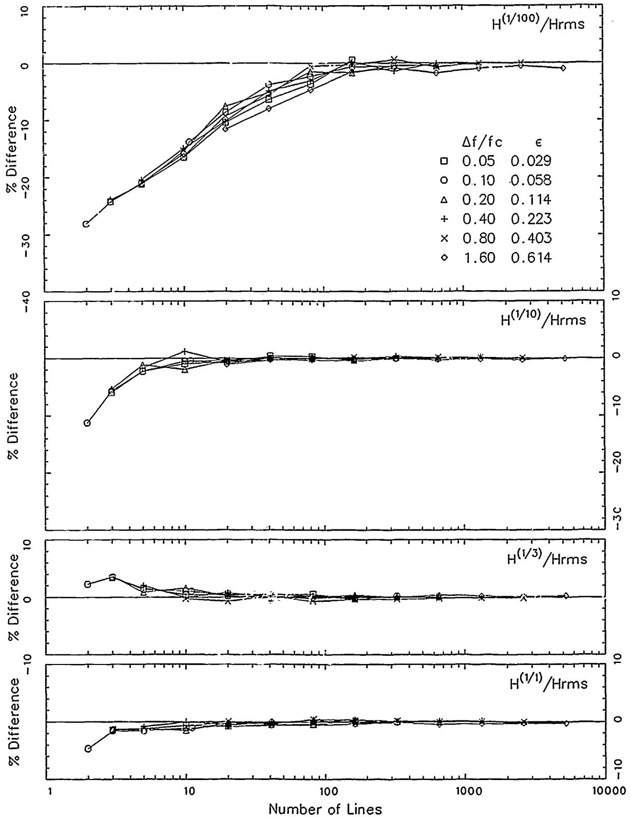
Figure 4. Synthetic wave height averages compared with Modified Rayleigh averages
