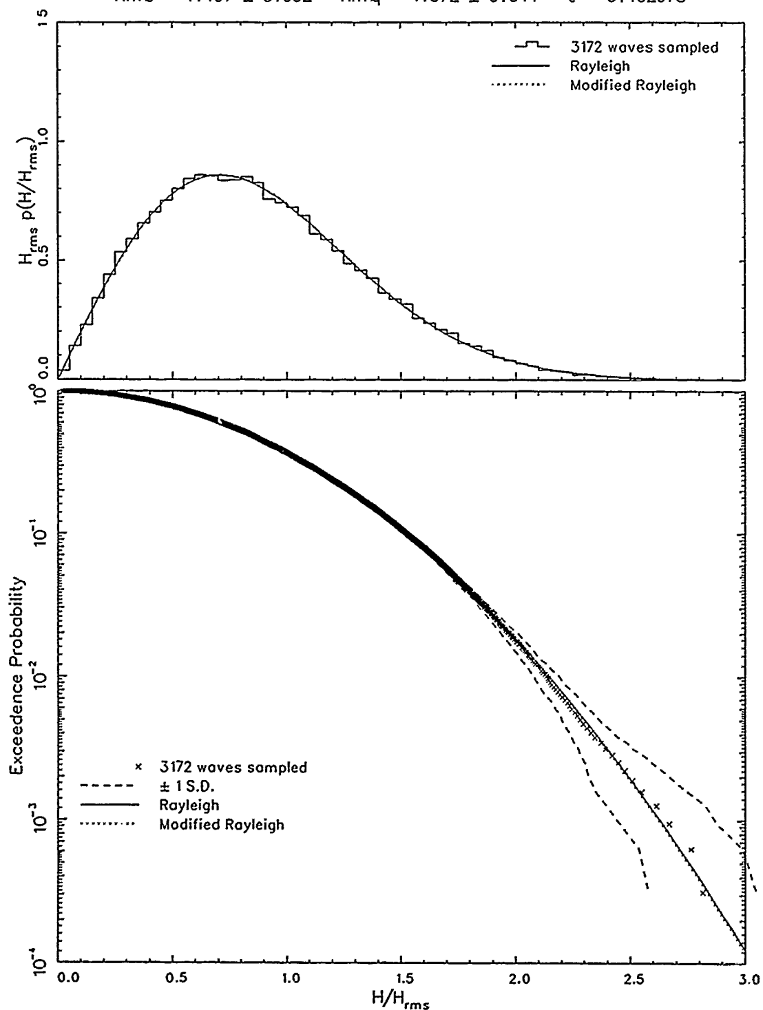
Figure 12. Probability and exceedence curves from bimodal spectra with small modal separation
