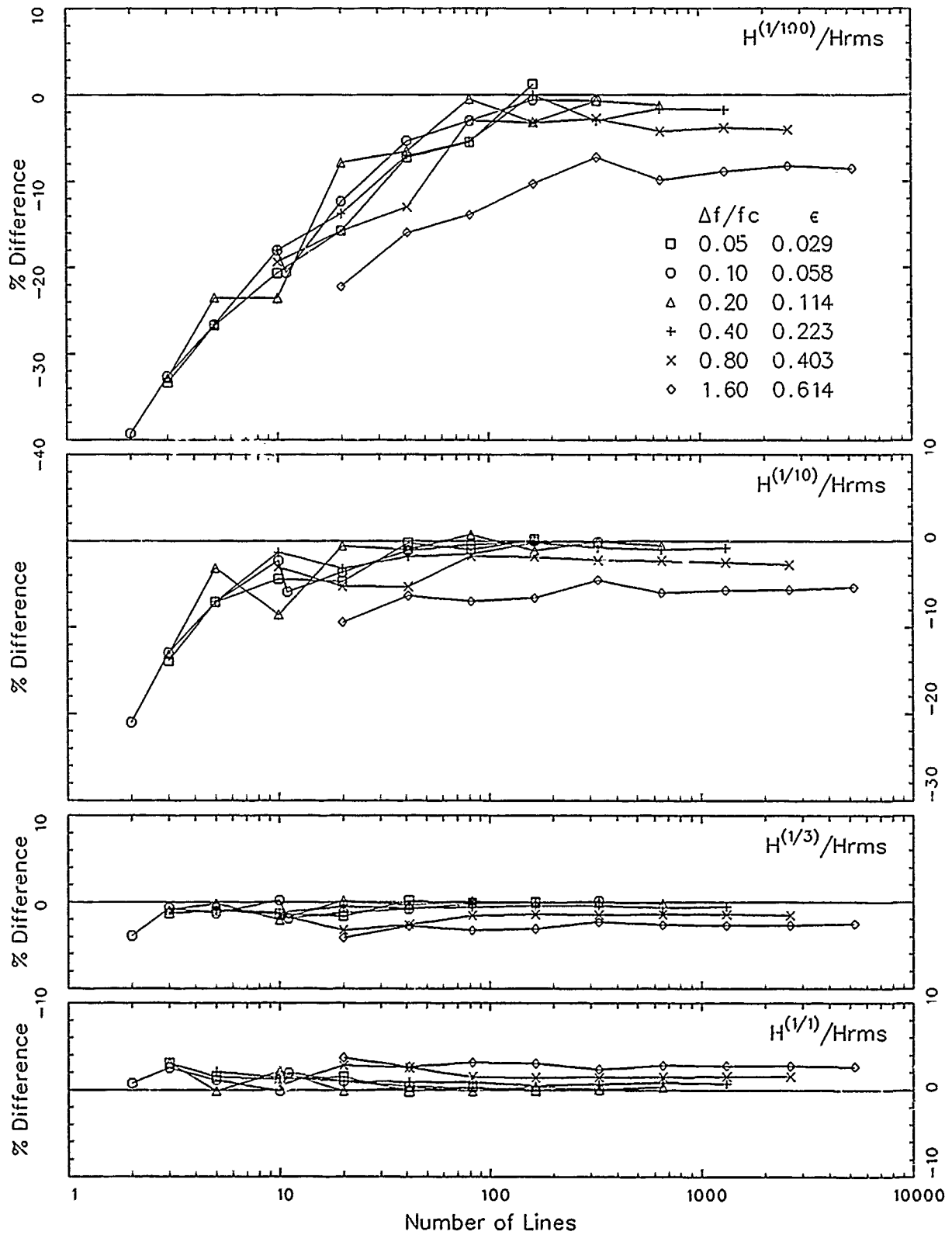
Figure 3. Synthetic wave height averages compared with Rayleigh averages
