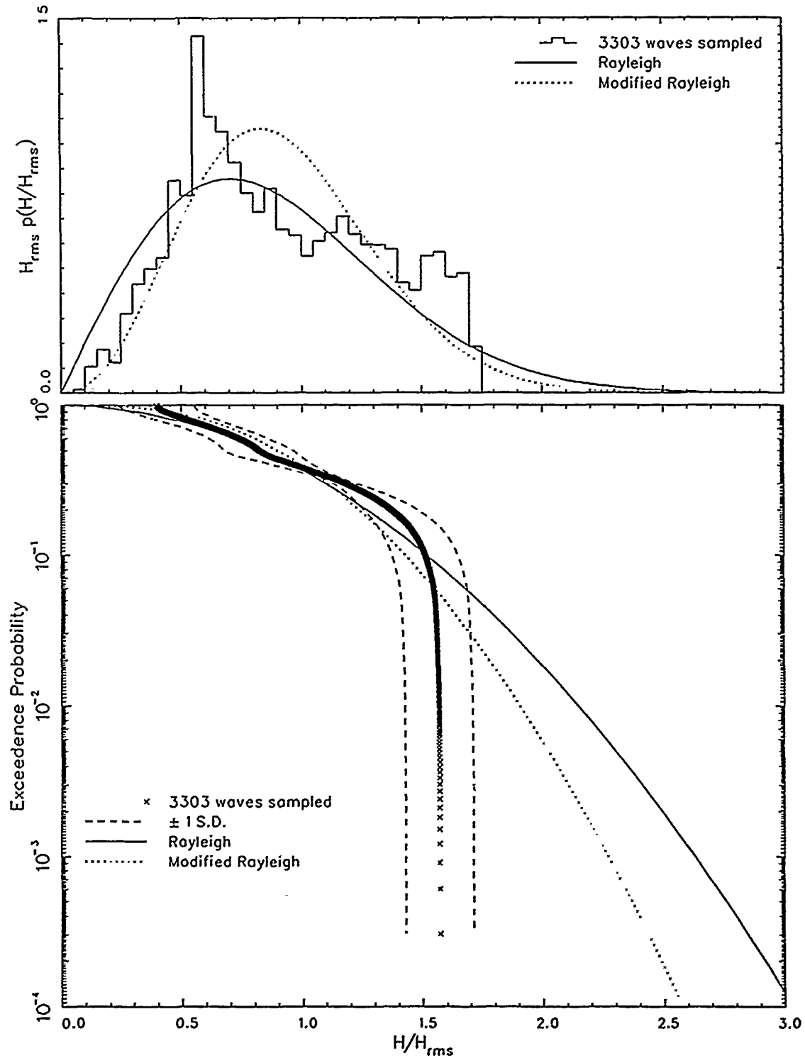
Figure 6. Probability and exceedence curves for three wave trains
