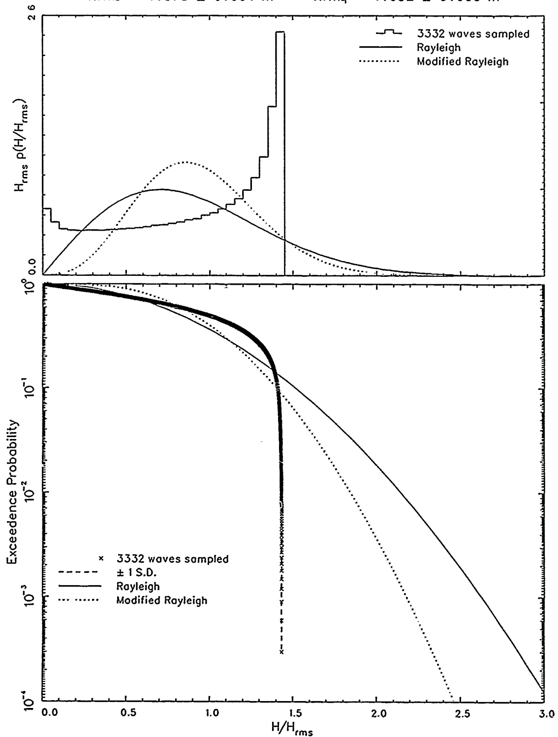
Figure 5. Probability and exceedence curves for two wave trains
