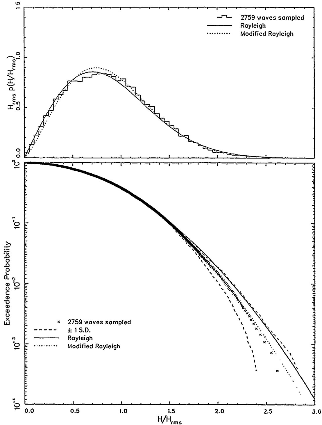
Figure 13. Probability and exceedance curves for bimodal spectra with intermediate modal separation
