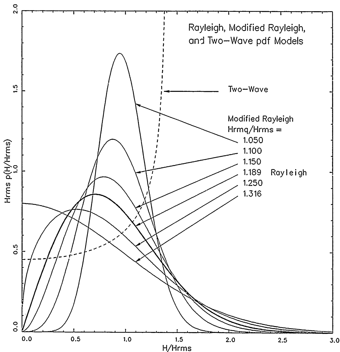
Figure 1. Examples of model curves
