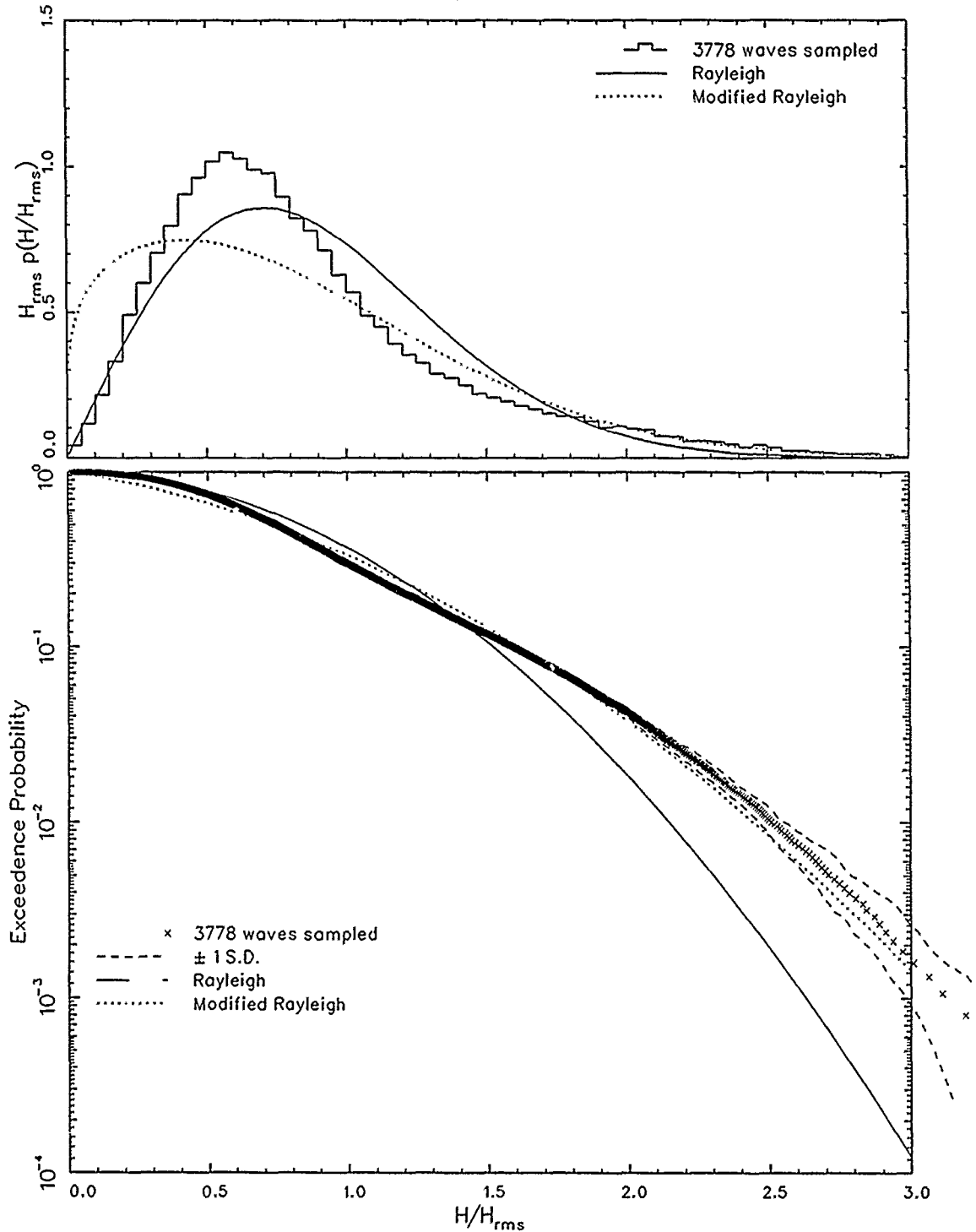
Figure 15. Probability and exceedence curves from bimodal spectra with large modal separation and small energy ratio
