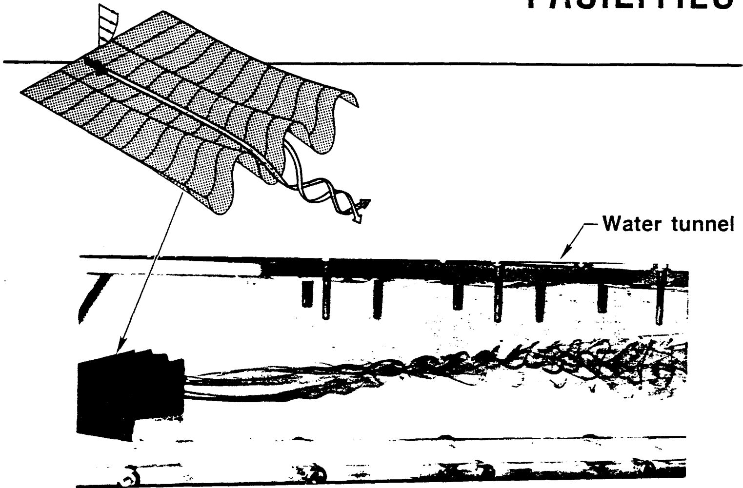
FIGURE 6 : Mixer Lobe Testing
