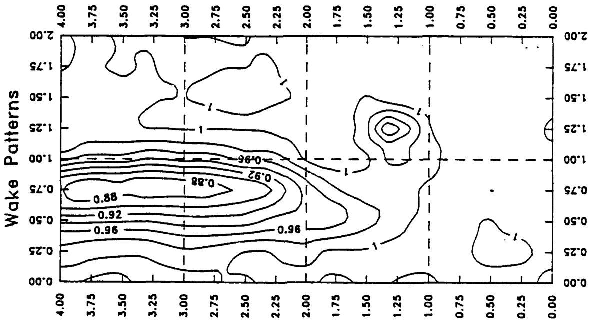
Triangular TE Wing L=1C
