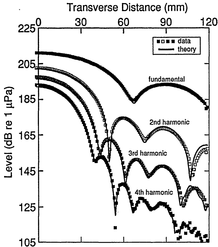
FIGURE 2.4 Beam Patterns of First Four Harmonics in Strong Source Experiment. Fundamental Frequency Is 1 MHz, Piston Radius Is 12 mm, Range Is 894 mm (about 3 Rayleigh Distances). Theoretical Curves Represent Bergen KZK Curves (Ref. 2).
