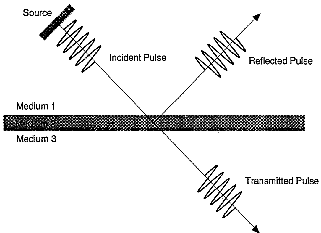
FIGURE 2.7 Three-fluid Problem.
