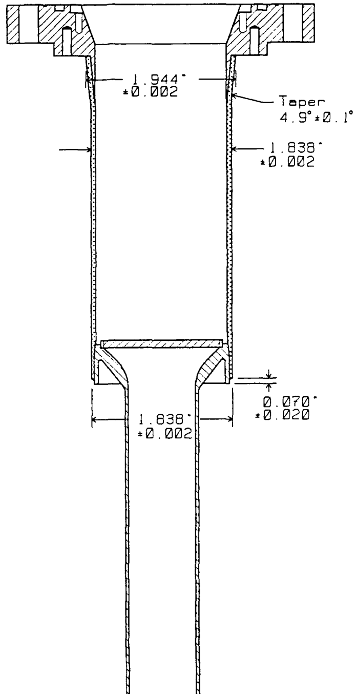
Figure D-24. FRP Outer Diameter
