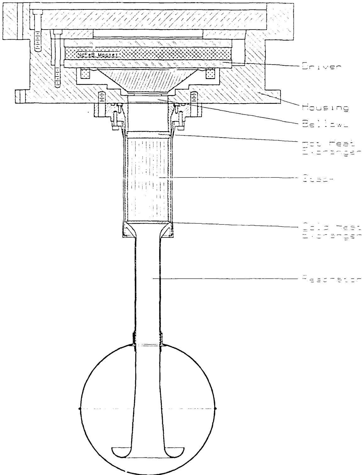
Figure 1-3. Acoustical Subsystems
