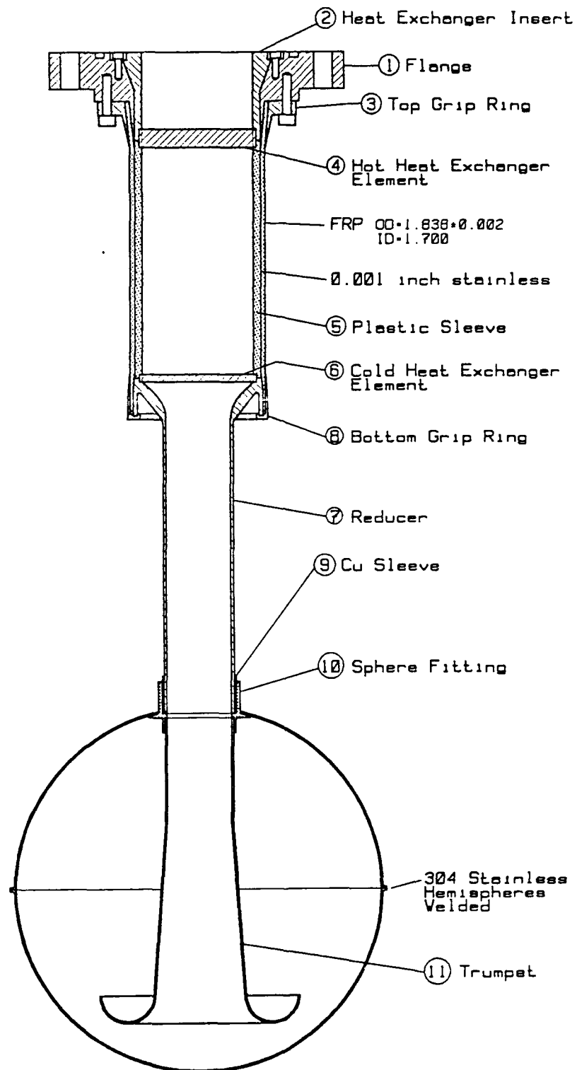
Figure III-2. STAR Resonator
