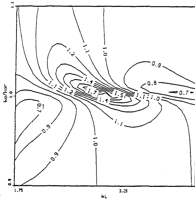
Figure 3-6c,d. Three Dimensional and Contour Plots of G_R as a Function of k_a and k_{l0} for N=8 , Conical Configuration, 1 atm.
