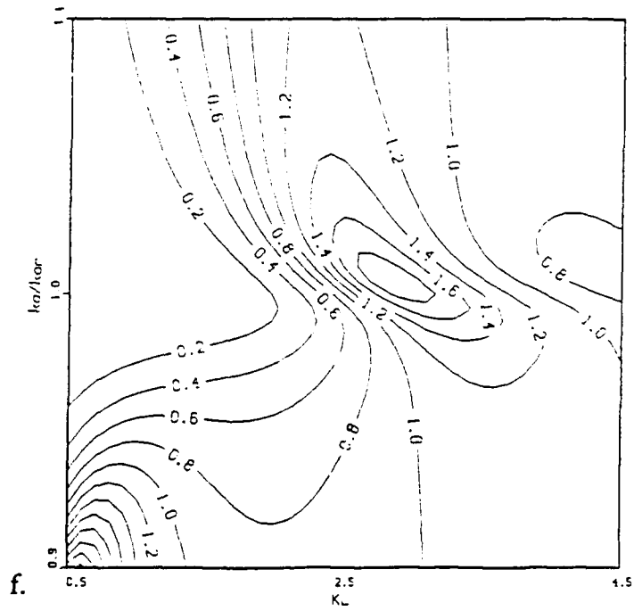
Figure 3-2e,f. Three Dimensional and Contour Plots of G_R as a Function of ka and kL for N=15 , Planar Configuration, 1 atm.
