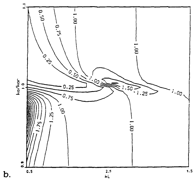
Figure 3-2a,b. Three Dimensional and Contour Plots of G_R as a Function of ka and kl_{10} for N=4 , Planar Configuration, 1 atm.
