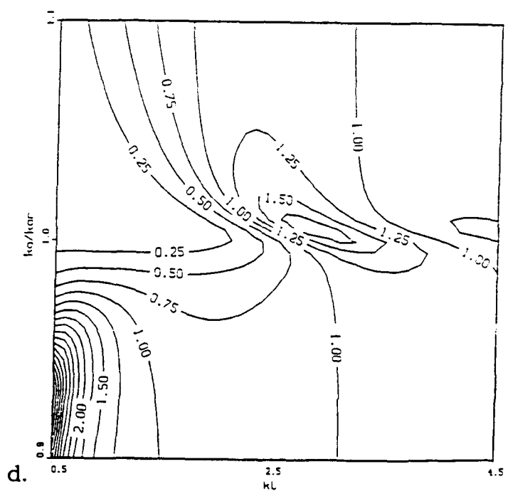
Figure 3-2c,d. Three Dimensional and Contour Plots of G_R as a Function of ka and kl_{n0} for N=8 , Planar Configuration, 1 atm.
