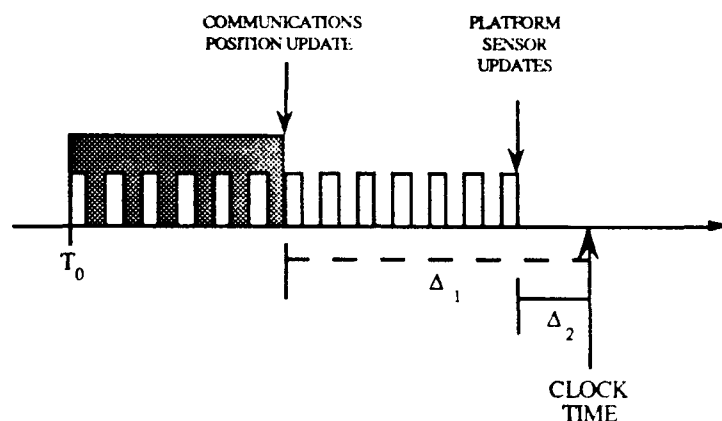
Figure 9. Timing Considerations
