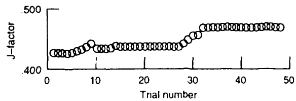
Figure 3.—J-factor as a function of optimizer trial number, using subroutine JFACTOR.
