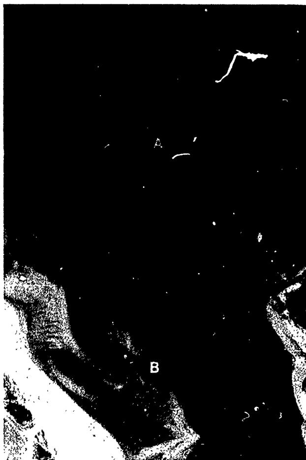
Figure 37. Oblique aerial photograph taken at low tide showing well-developed ebb-oriented sandwaves on outer flanks of main ebb channel. Regard (A) in photograph. Note also the well-developed flood-oriented sandwaves in the updrift marginal flood channel. Regard (B) in photograph.
