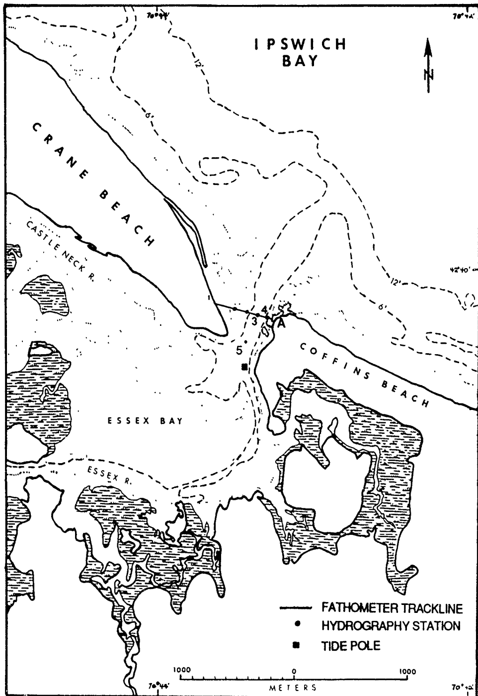
Figure 26. Location of hydrography stations 1-5 utilized to determine inlet hydraulic parameters. Cross section A-A' is shown in Figure 27.
