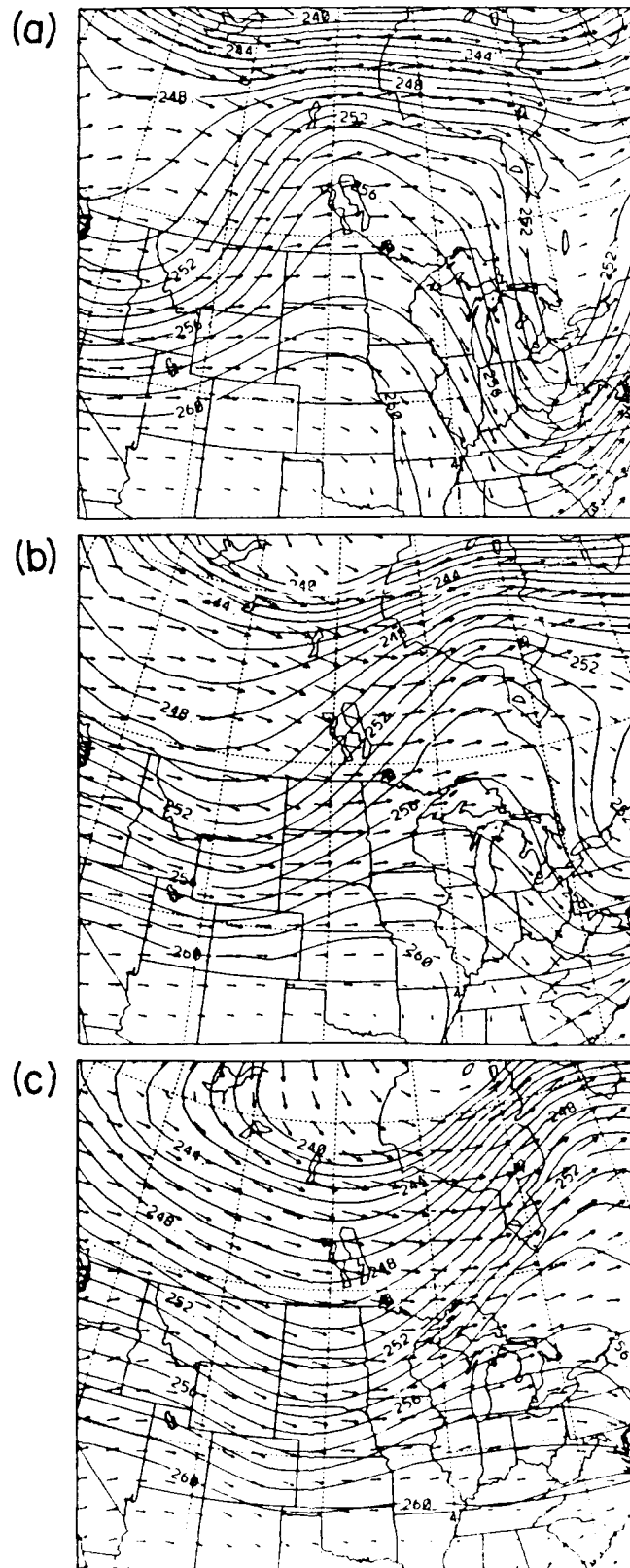
Figure 5.4: 900 mb temperature (K) and winds (m/s) at (a) 0000 UTC, (b) 1200 UTC, (c) 2400 UTC.
