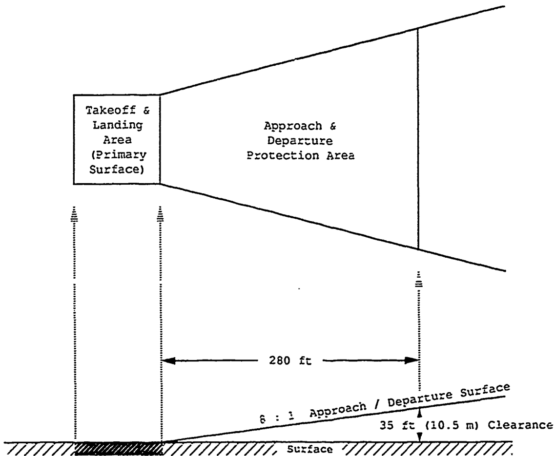
FIGURE 8 VISUAL APPROACH AND DEPARTURE PROTECTION AREA
