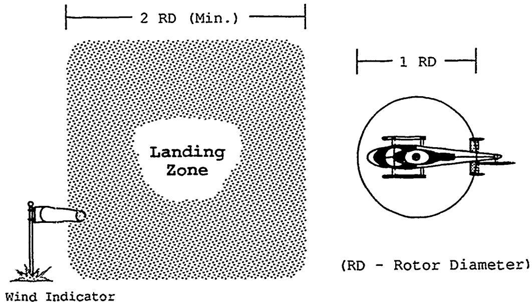
FIGURE 7 MINIMUM LANDING ZONE REQUIREMENTS
