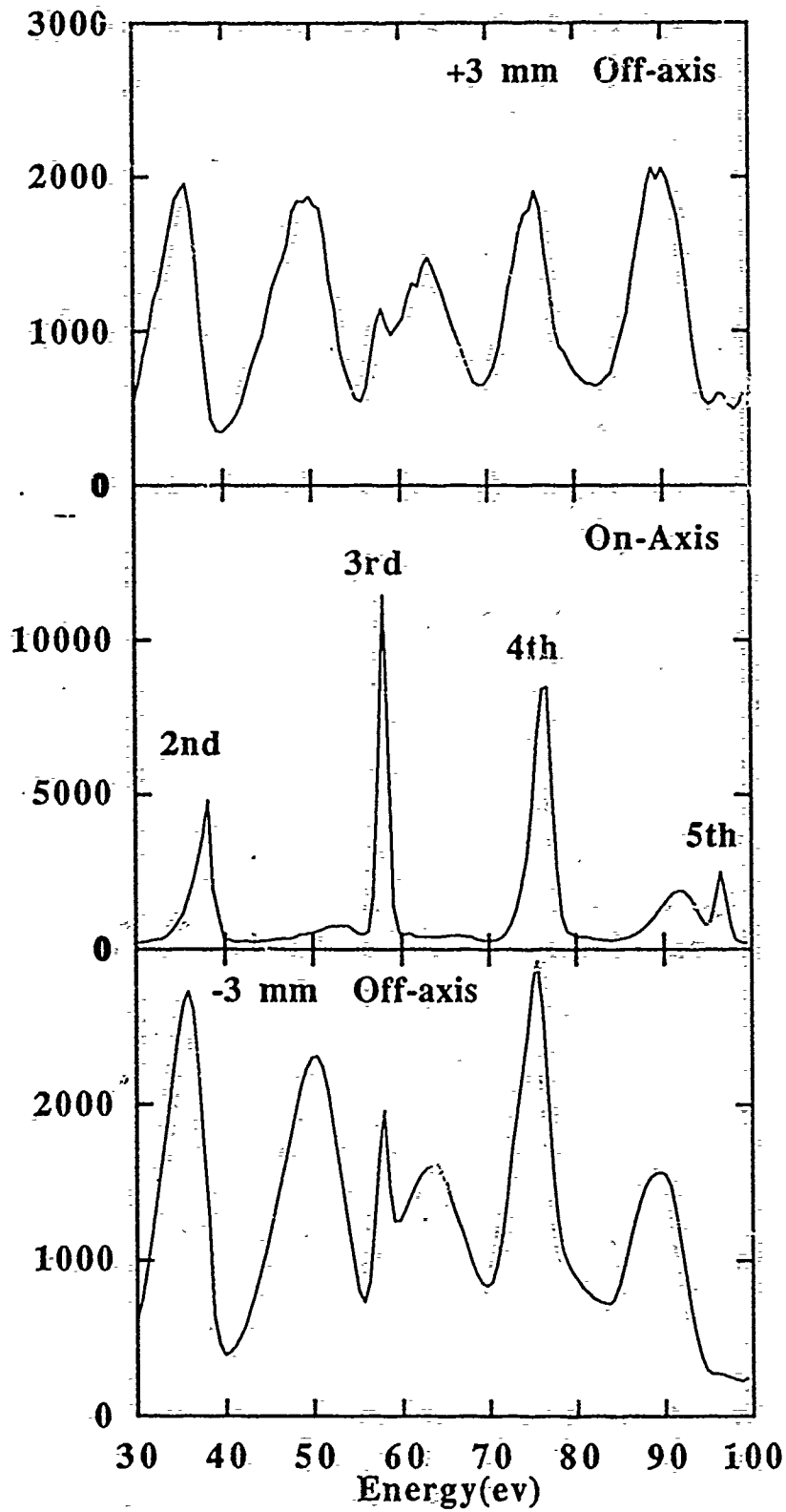
U5 Undulator Spectra, Horizontal Scan 1 mm Pinhole
