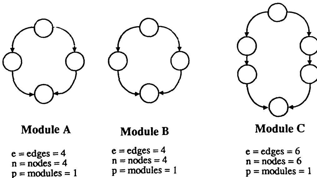
FIGURE 3.3-5. THREE MODULES
