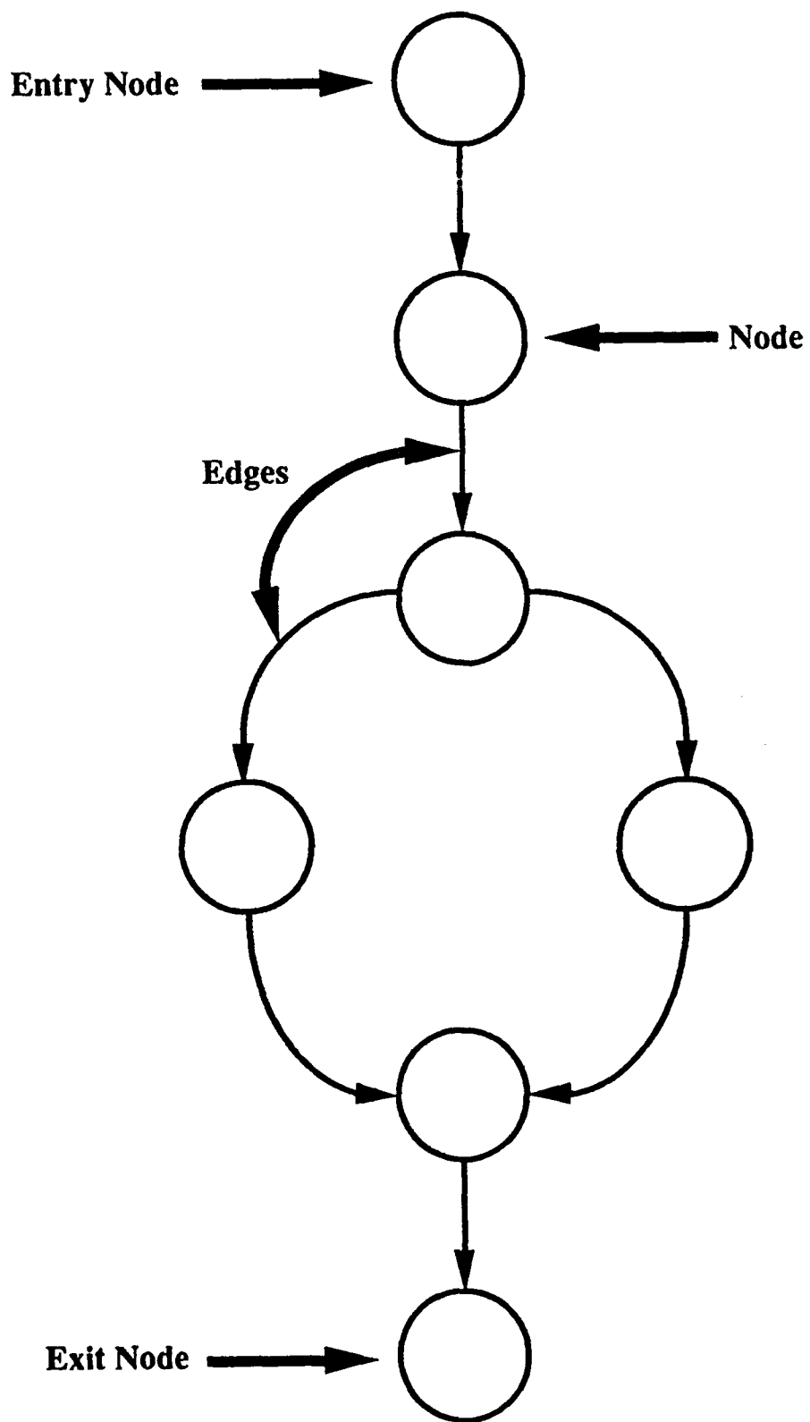
FIGURE 3.3-1. A PROGRAM CONTROL GRAPH AND ITS ELEMENTS
