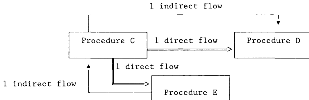
FIGURE 3.7-2. EXAMPLE OF INDIRECT LOCAL INFORMATION FLOW
