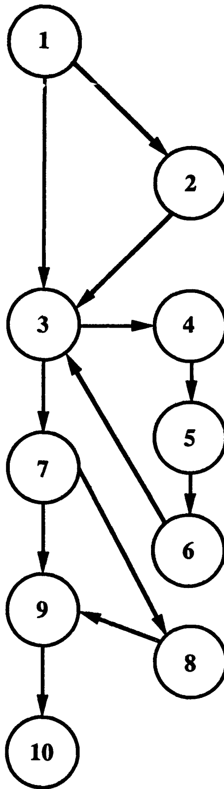
FIGURE 3.3-3. A PROGRAM CONTROL GRAPH OF FORTRAN CODE
