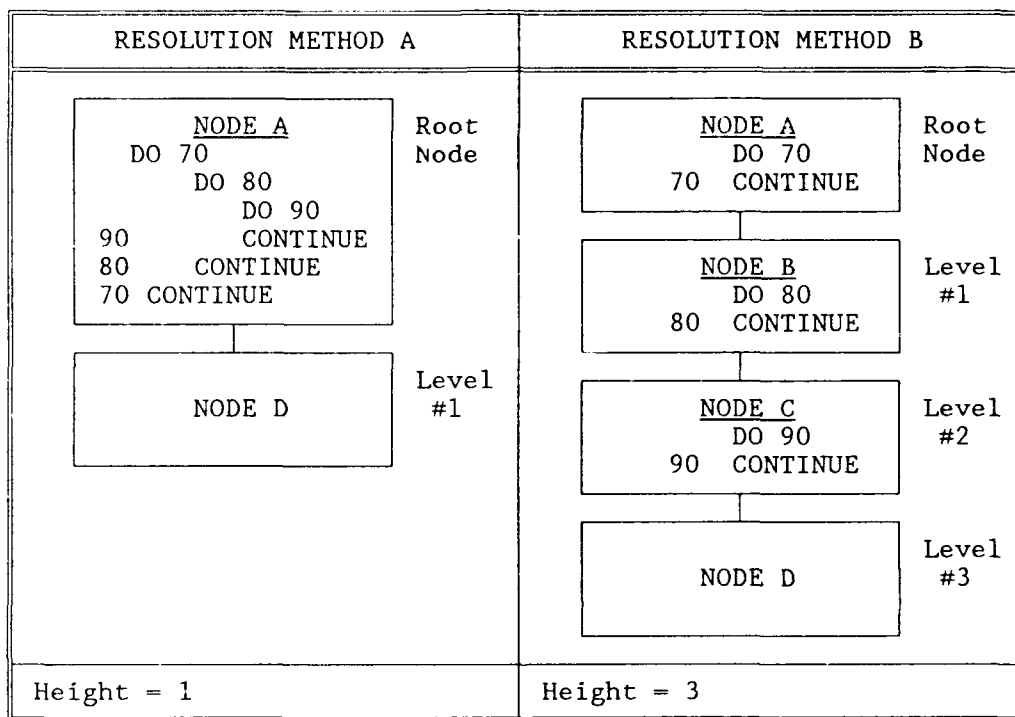
FIGURE 3.6-2. TWO INTERPRETATIONS OF RESOLVING NESTED DO LOOPS
