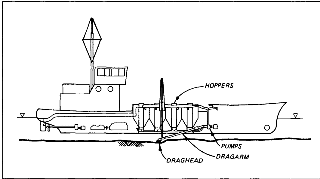
Figure 7. Hopper dredge (from McLellan et al. 1989)
