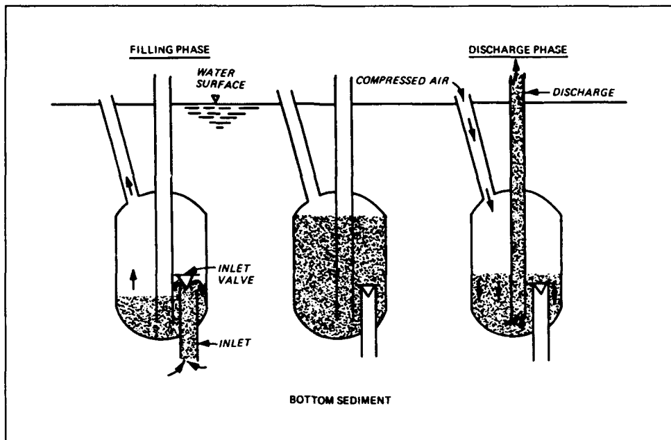
Figure 10. Pneumatic pump operation (from Herbich and Brahme 1991)
