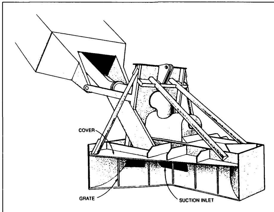
Figure 4. Matchbox dredgehead
