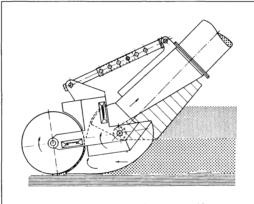
Figure 9. IHC Roller Silt draghead (from Van Dooremalen et al. 1983)
