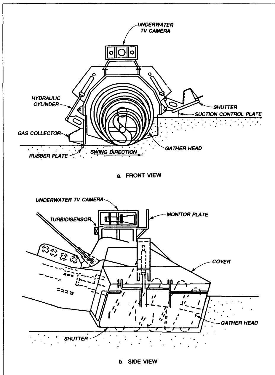
Figure 5. Refresher dredgehead (from Raymond 1984)
