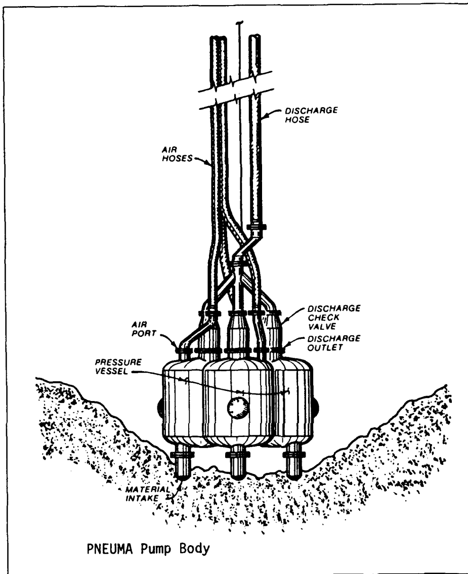
Figure 11. Pneuma dredgehead (from Herbich and Brahme 1991)
