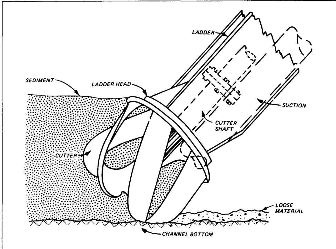
Figure 2. Conventional cutterhead (modified from Huston and Huston 1976)
