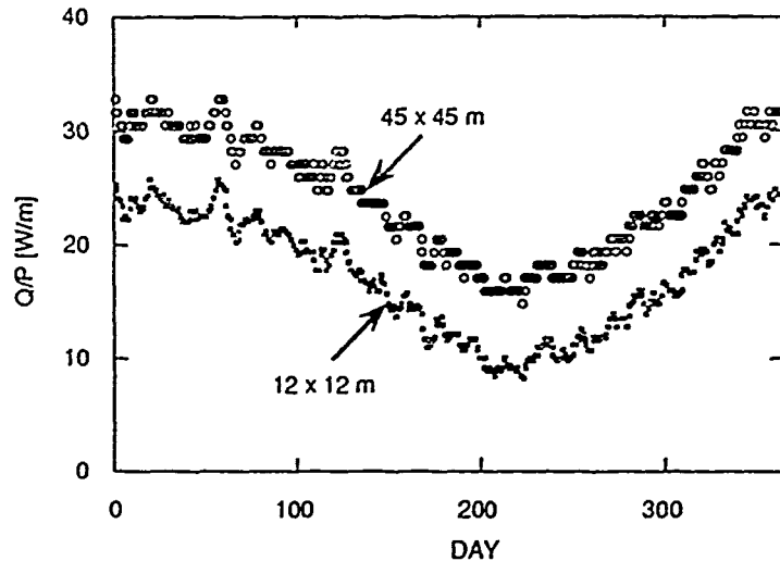
Figure 2. Daily-averaged heat loss per unit perimeter length for large and small slabs, Medford, OR.
