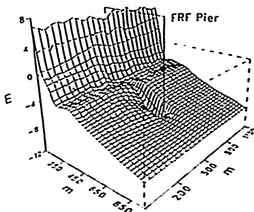
Figure 22. Permanent trough under the FRF pier, 27 February 89
