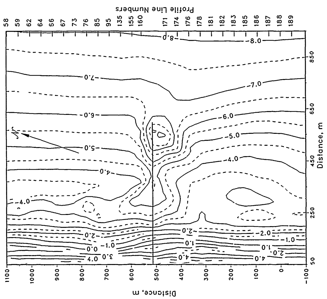
Figure A7. FRF Bathymetry 15 June 89 (depths relative to NGVD)
