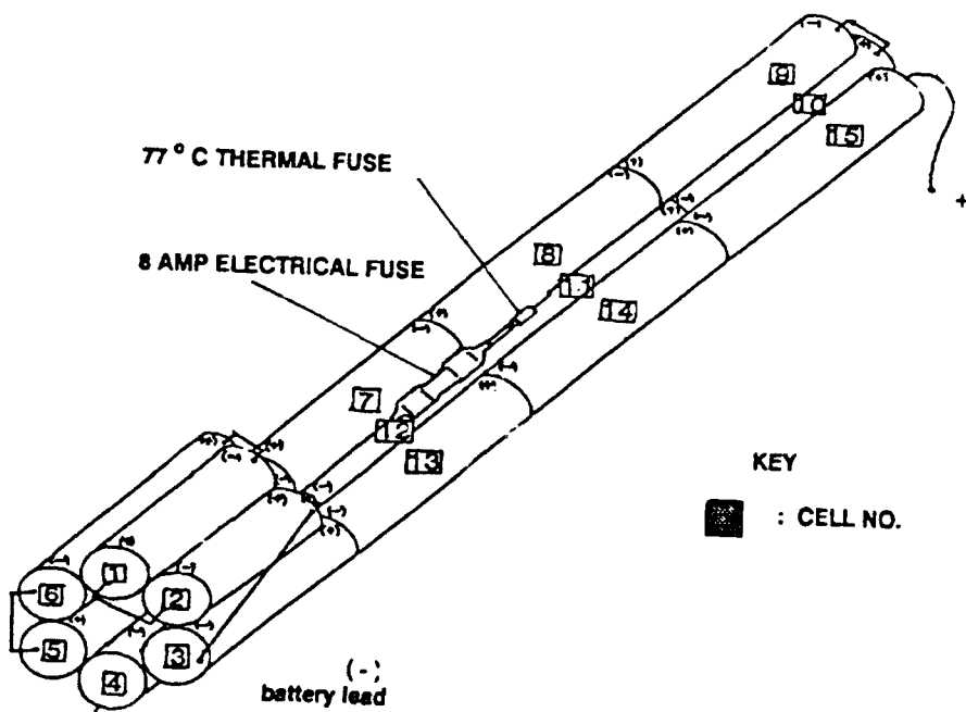
FIGURE 2-3. BATTERY PACK CONFIGURATION, FUSE PLACEMENT
