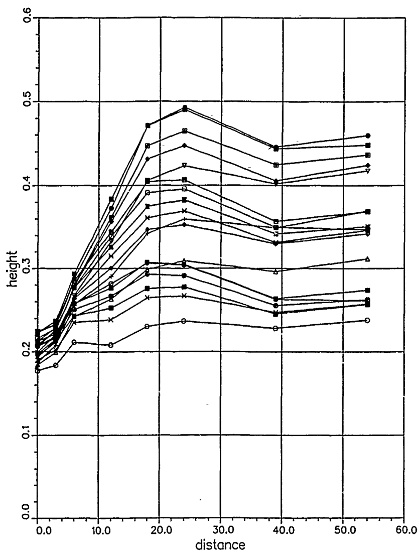
Figure 6. Energy-based wave height computed from the averaged spectra (each line represents a different test)
