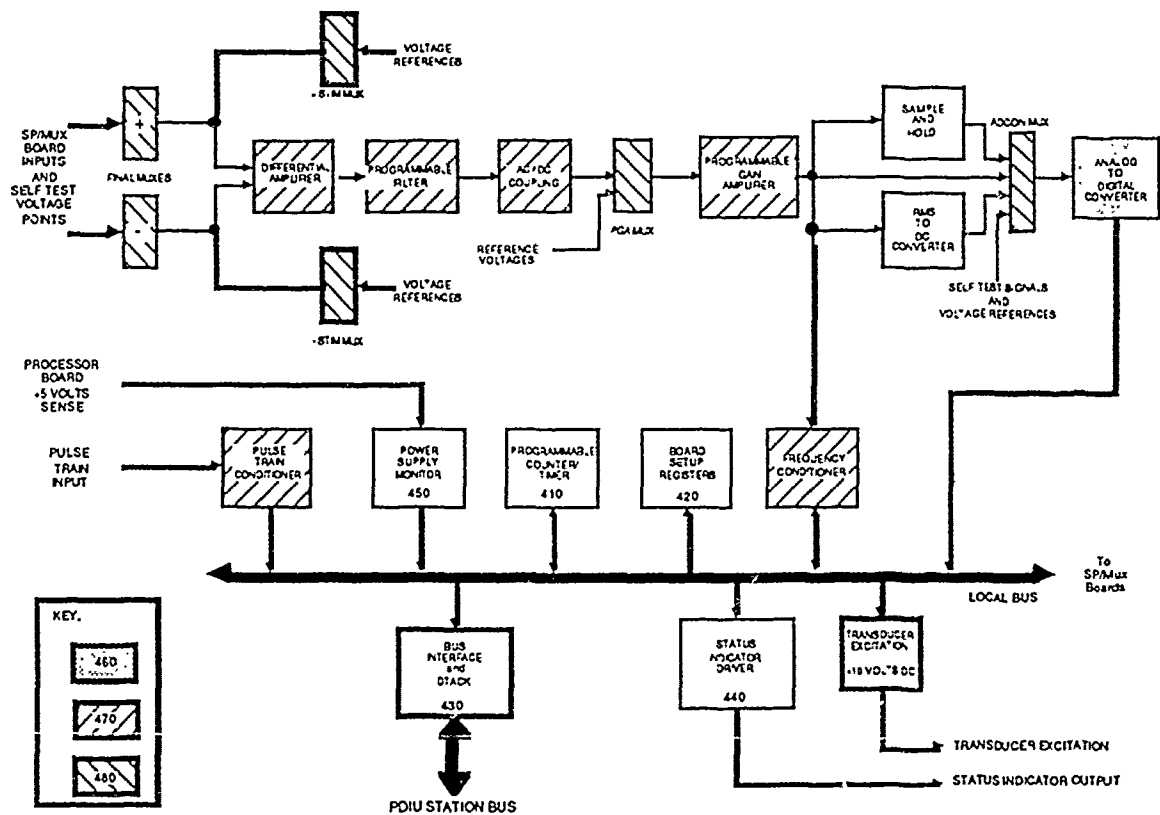
Figure 4. PDIU I/O Board Configuration
