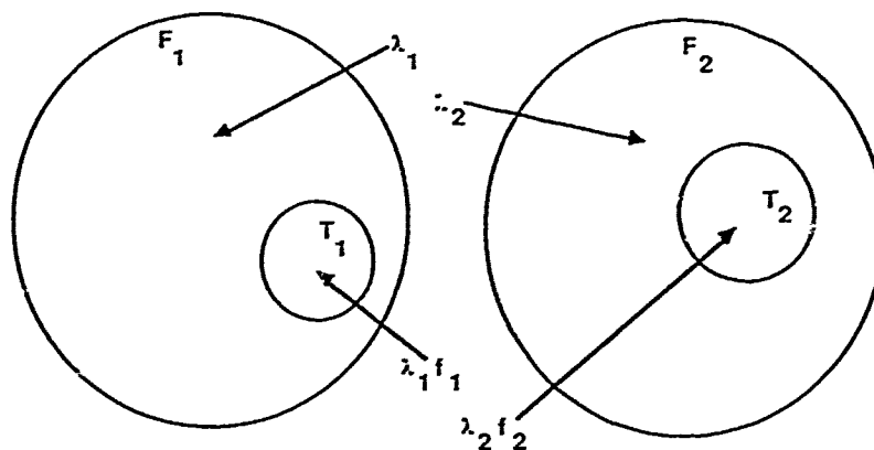
Figure 8-4. Fault Coverage of Tests 1 and 2
