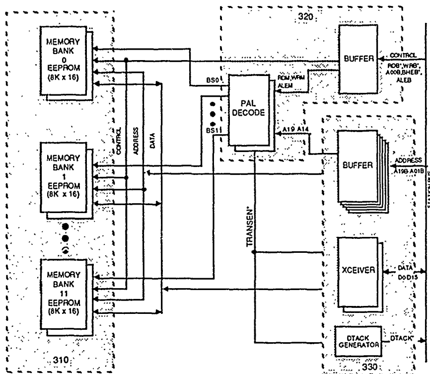
Figure 3. PDIU Memory Board Configuration
