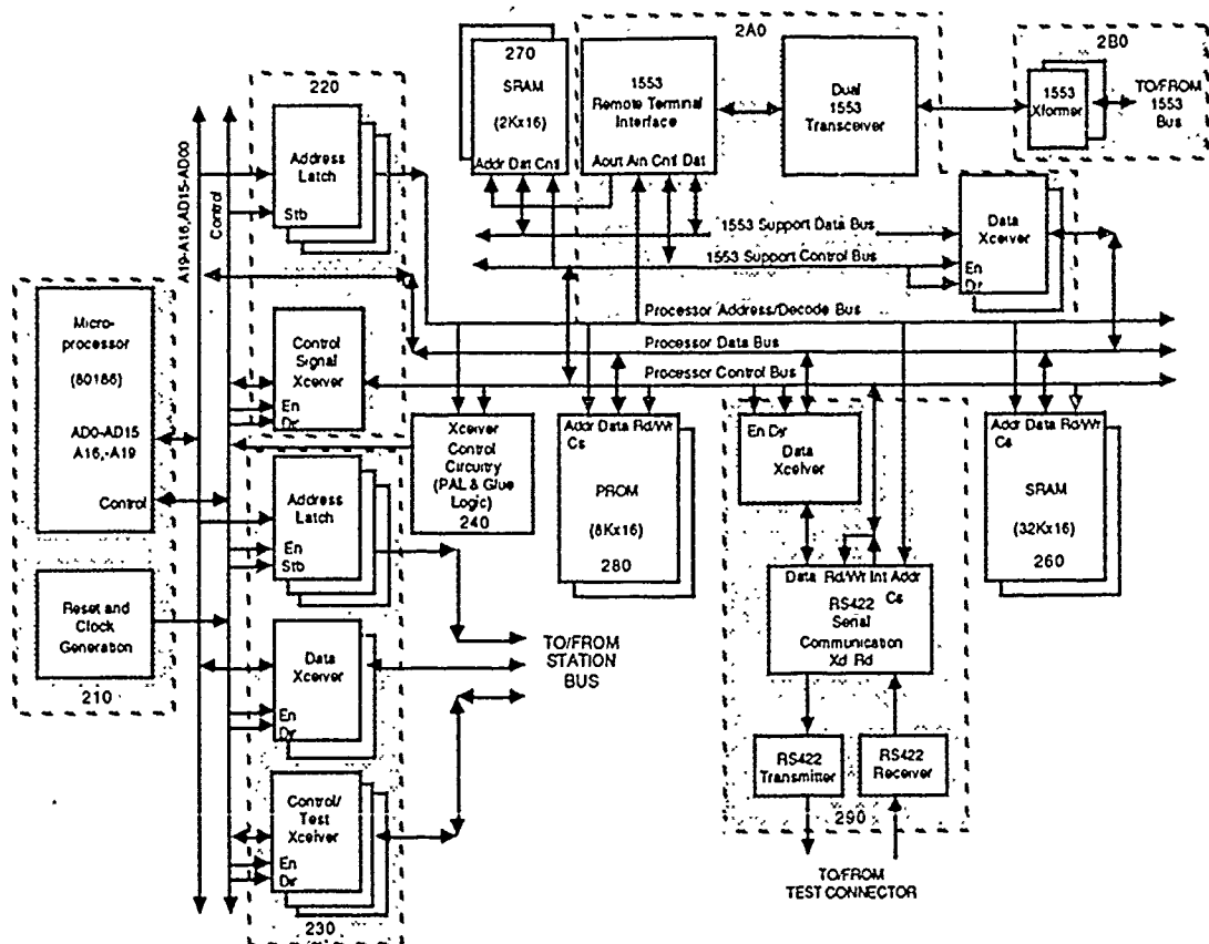
Figure 2. PDIU Processor Board Configuration
