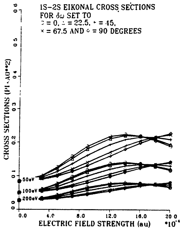
Fig. 2. Cross section vs laser field strength, for third order Floquet dressed hydrogen atoms, in laser assisted e^- + \text{H}(1\text{S}) collisions, using a multichannel Eikonal treatment. (a) 1S-2S and (b) 1S-2P 0 cross sections. Cross sections are compared over a range of phases and impact energies.
