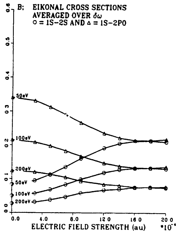
Fig. 3 1S-2S and 1S-2P 0 cross sections vs laser field strength, for third order Floquet dressed hydrogen atoms, in laser assisted e^- + \text{H}(1\text{S}) collisions, using (a) Born-wave and (b) multichannel Eikonal treatments. The cross sections are averaged over \delta\omega in the range 0^\circ to 90^\circ and compared over a range of impact energies.
