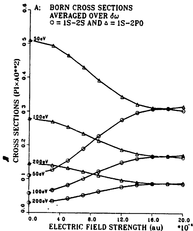
Fig. 3 1S-2S and 1S-2P 0 cross sections vs laser field strength, for third order Floquet dressed hydrogen atoms, in laser assisted e^- + \text{H}(1\text{S}) collisions, using (a) Born-wave and (b) multichannel Eikonal treatments. The cross sections are averaged over \delta\omega in the range 0^\circ to 90^\circ and compared over a range of impact energies.
