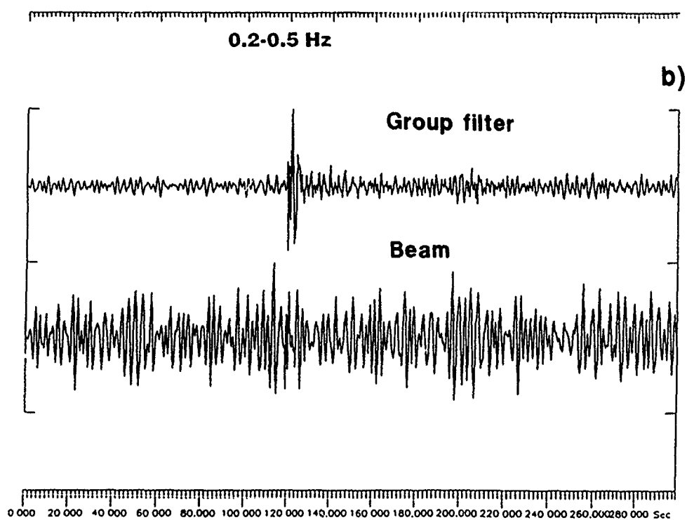
Fig. 7.7.10. Example of nuclear explosion record filtered by beam and AOGF in: a) broad frequency band and b) low frequency band.
