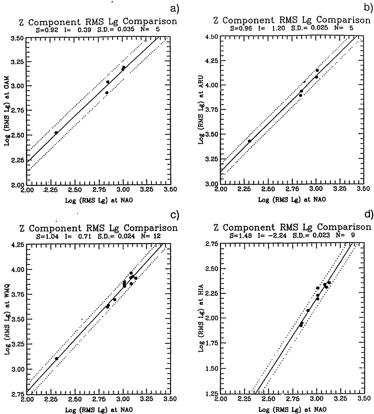
Fig. 7.1.2. Examples of observed correlations between RMS Lg at NORSAR and selected stations in the USSR and China. Note the excellent consistency in all of the plots.
