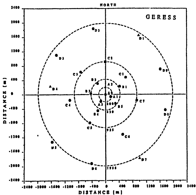
Fig. 7.2.1. Geographical location and geometry of the GERESS array in Germany (after Harjes, 1990).
