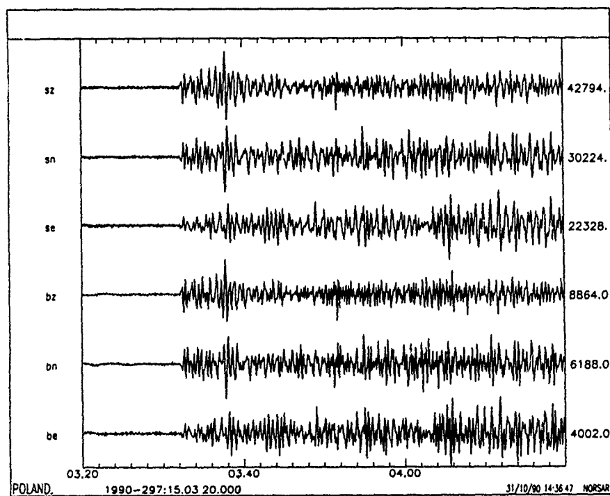
Fig. 7.6.3. Short period (sz, sn, se) and broad band (bz, hn, be) 3-component recording at Ksiaz of the 24 October 1990 nuclear explosion at Novaya Zemlya. The upper frame shows 20 minutes of data, whereas the lower frame covers a one-minute interval around the P onset.
