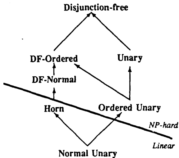
Figure 7.2: The complexity of goal-directed reasoning in the restricted default theories considered by Kautz and Selman.
