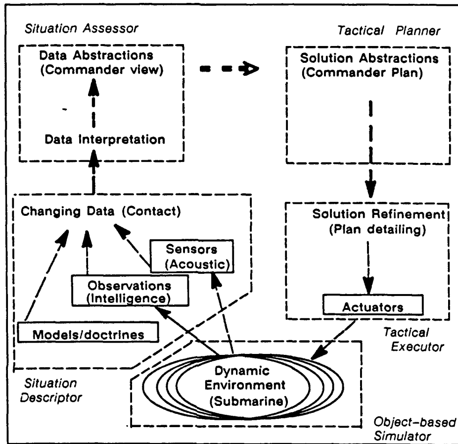
Figure 1.5: The Dynamic Classification Problem
