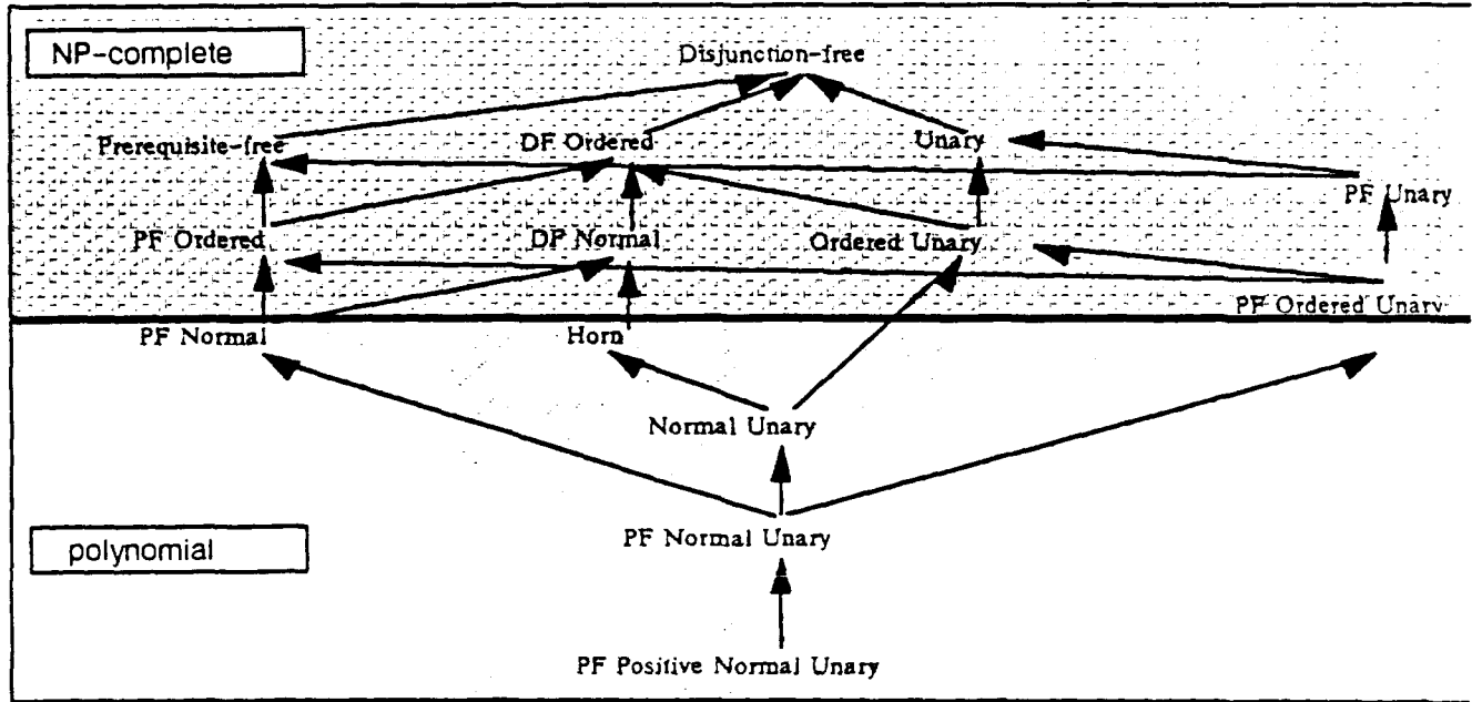
Figure 8.5: The complexity of membership problems with single literal theories.
