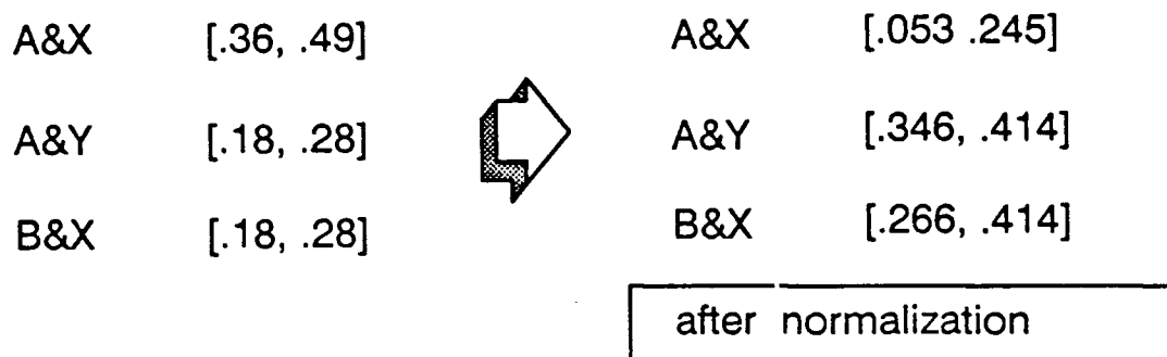
Figure 1.10: Computation of New Bounds (Normalized)
