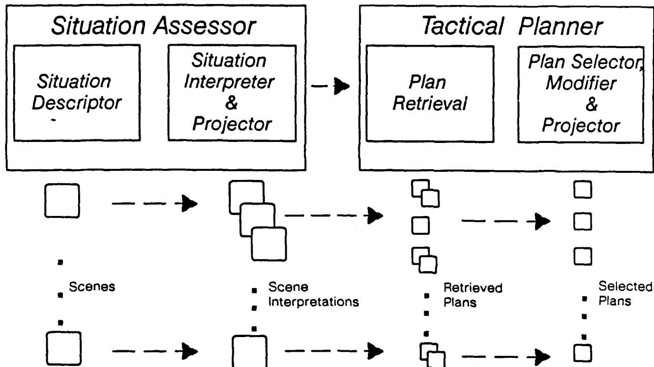
Figure 1.6: Ambiguity and Uncertainty in SA and TP
