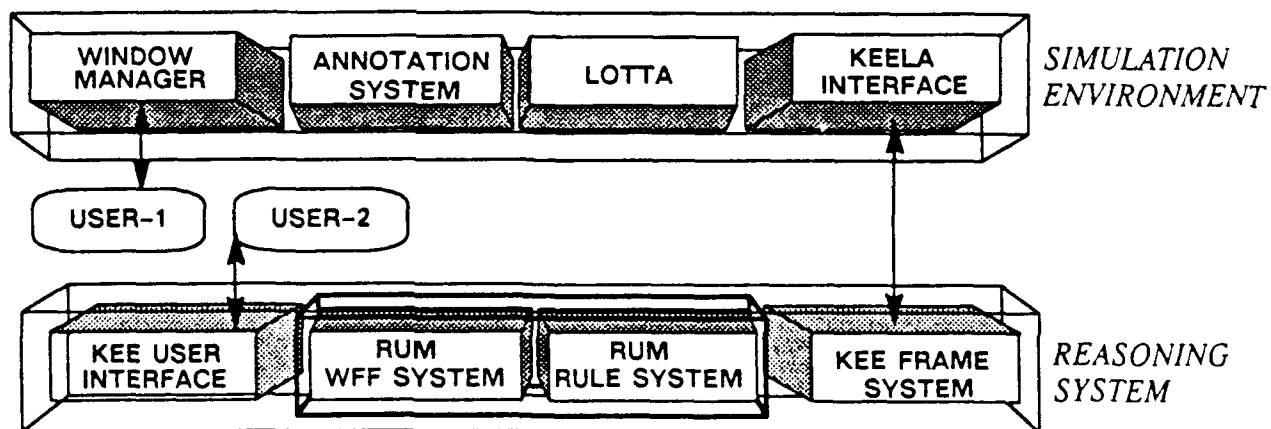
Figure 3.2: The Test-bed Architecture
