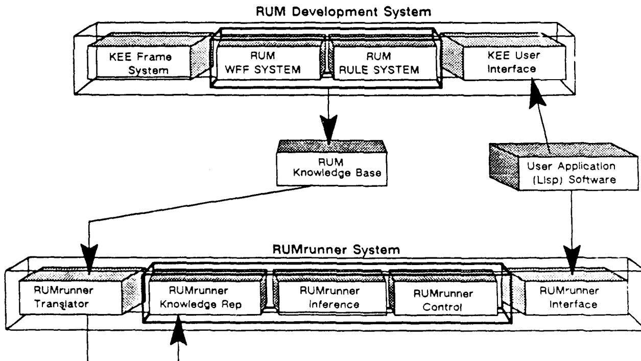
Figure 3.5: Transitioning from Development to Deployment
