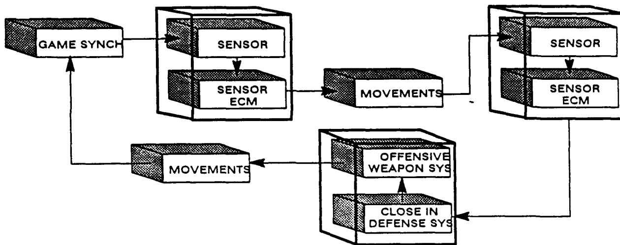
Figure 3.3: Simulation Cycle in LOTTA
