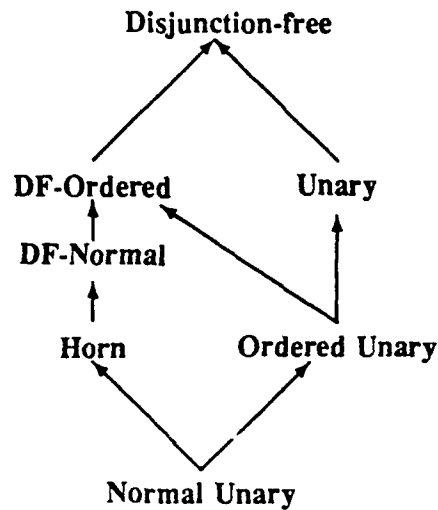
Figure 8.1: Kautz and Selman's hierarchy of default theories.
