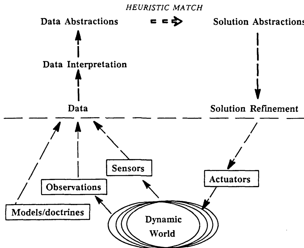
Figure 3.1: The Dynamic Classification Problem
