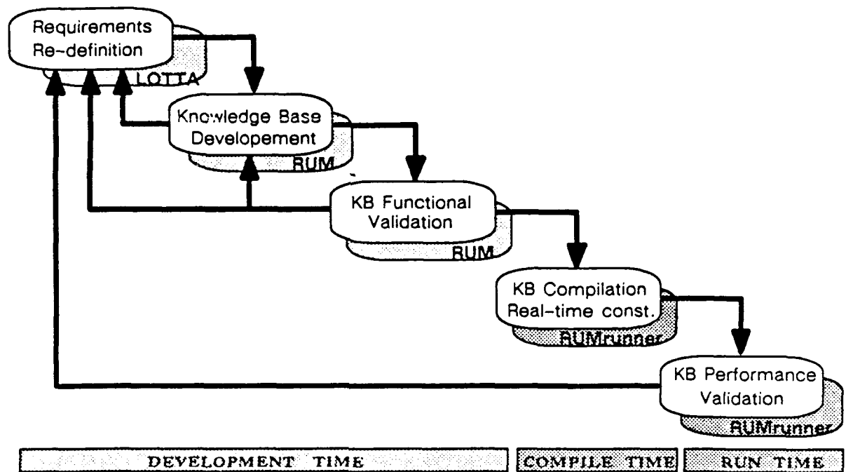
Figure 1.2: Software Engineering with RUM and RUMrunner
