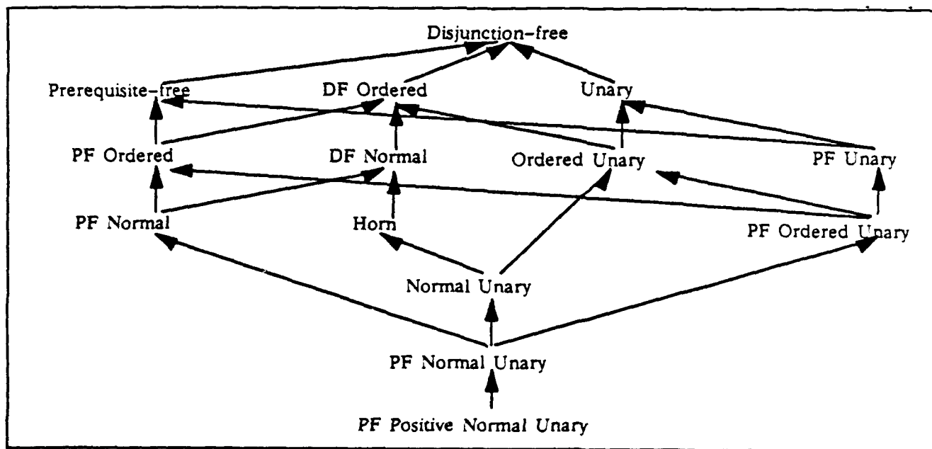
Figure 8.2: An expanded hierarchy of default rules.
