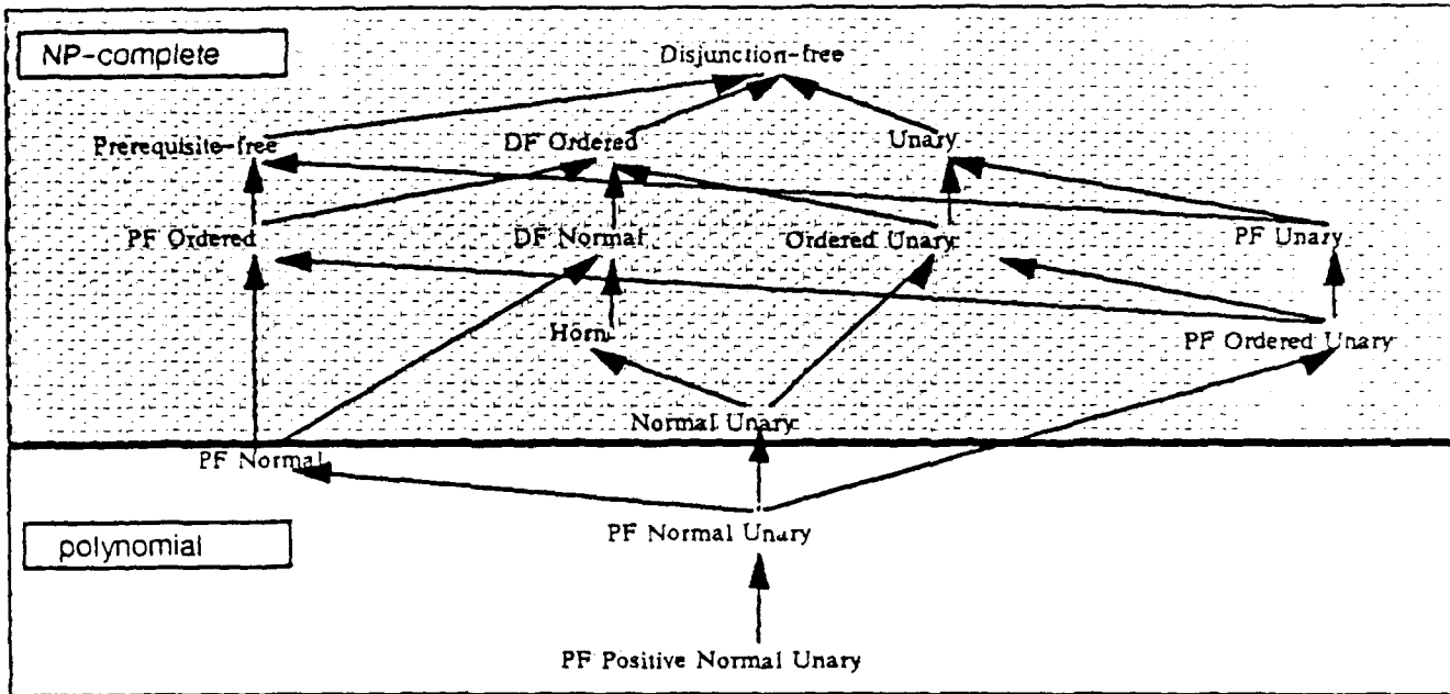
Figure 8.4: The complexity of membership problems with 2-literal theories.
