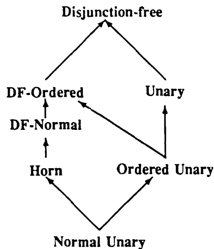
Figure 7.1: Kautz and Selman's hierarchy of restricted default theories.
