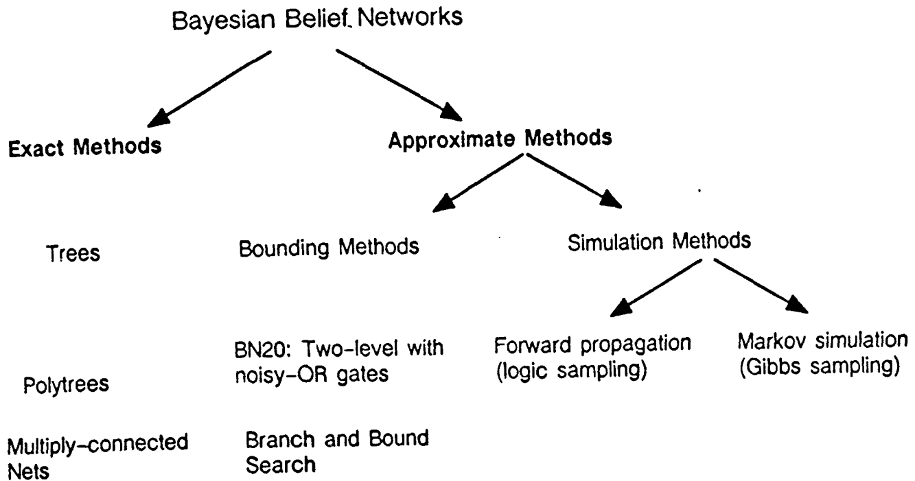
Figure 1.1: Taxonomy of Inference Mechanisms for Bayesian Belief Networks
