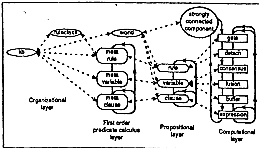
Figure 9.1: PRIMO's three levels of abstraction.
