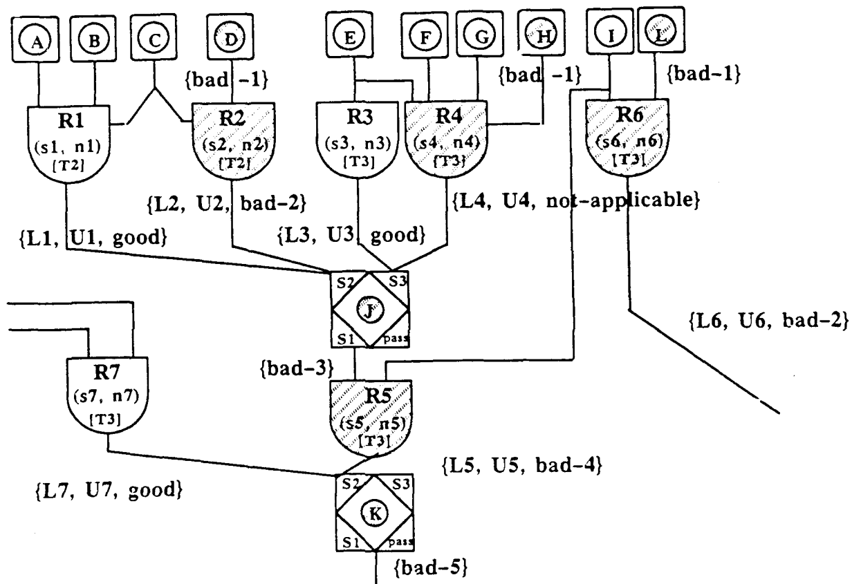
Figure 2.3: Portion of an Acyclic Deductive Graph
