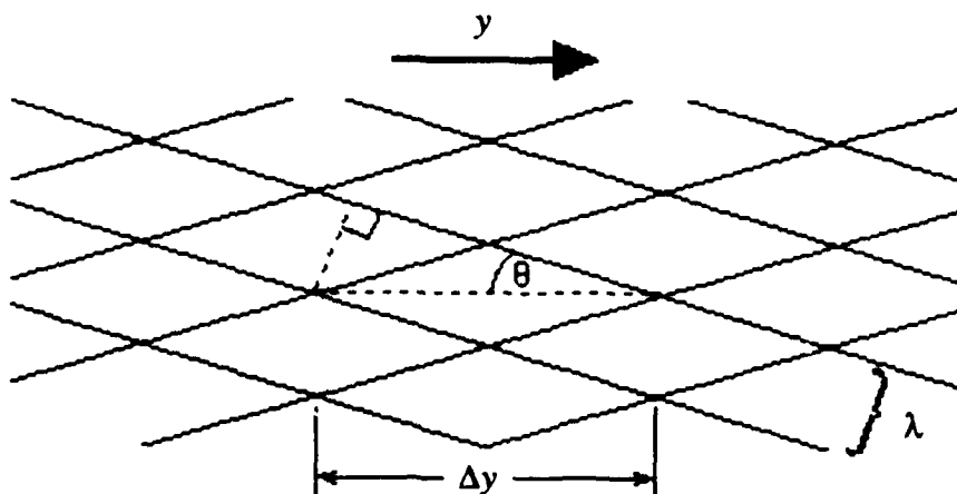
Figure 4.5. Separation of Fringes.
