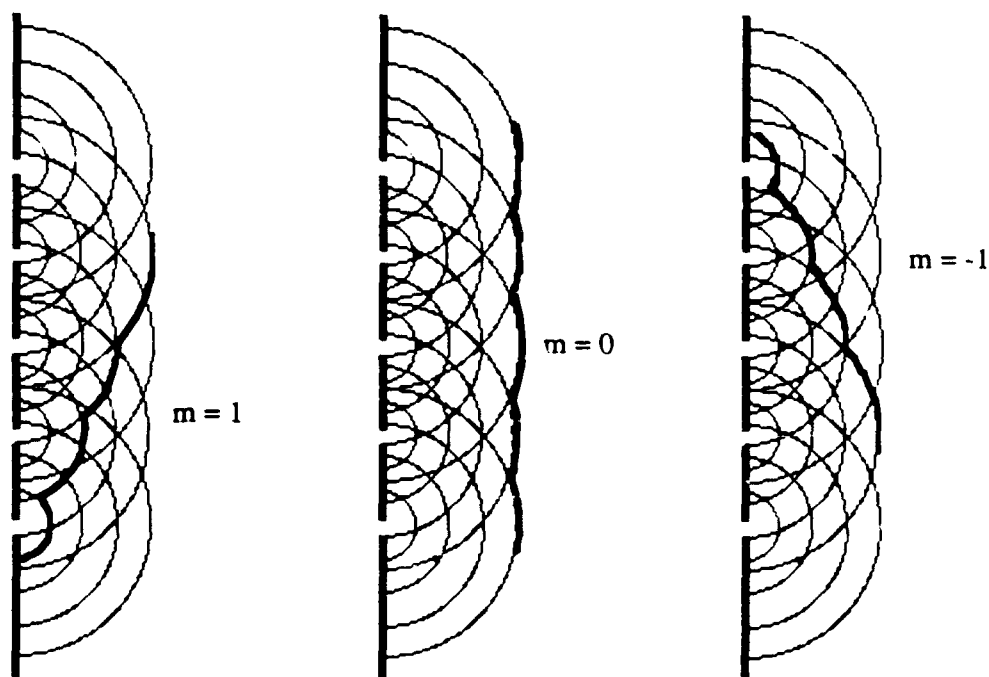
Figure 3.1. Diffraction from Multiple Slits.
