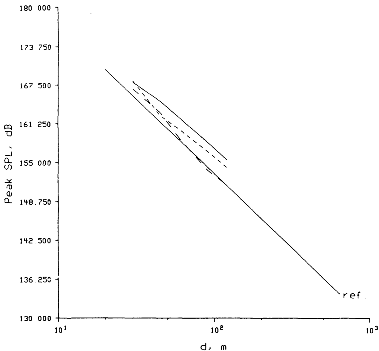
Figure 11.21. 162 dB initial peak pressure SPL versus range for porous surface propagation. The 0 m receiver height is given by the solid line, the 1 m height by the short dashed line, and the 5 m height by the long dashed line. The solid line ending with the label "ref." shows a decay of r^{-1.2} for reference.
