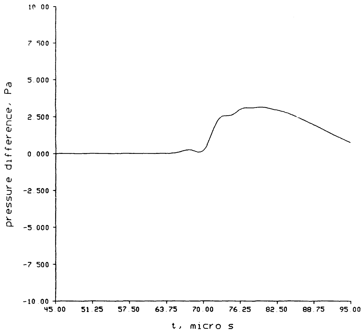
Figure 8.5. Acoustic pressure difference in Pa between cases one and four.
