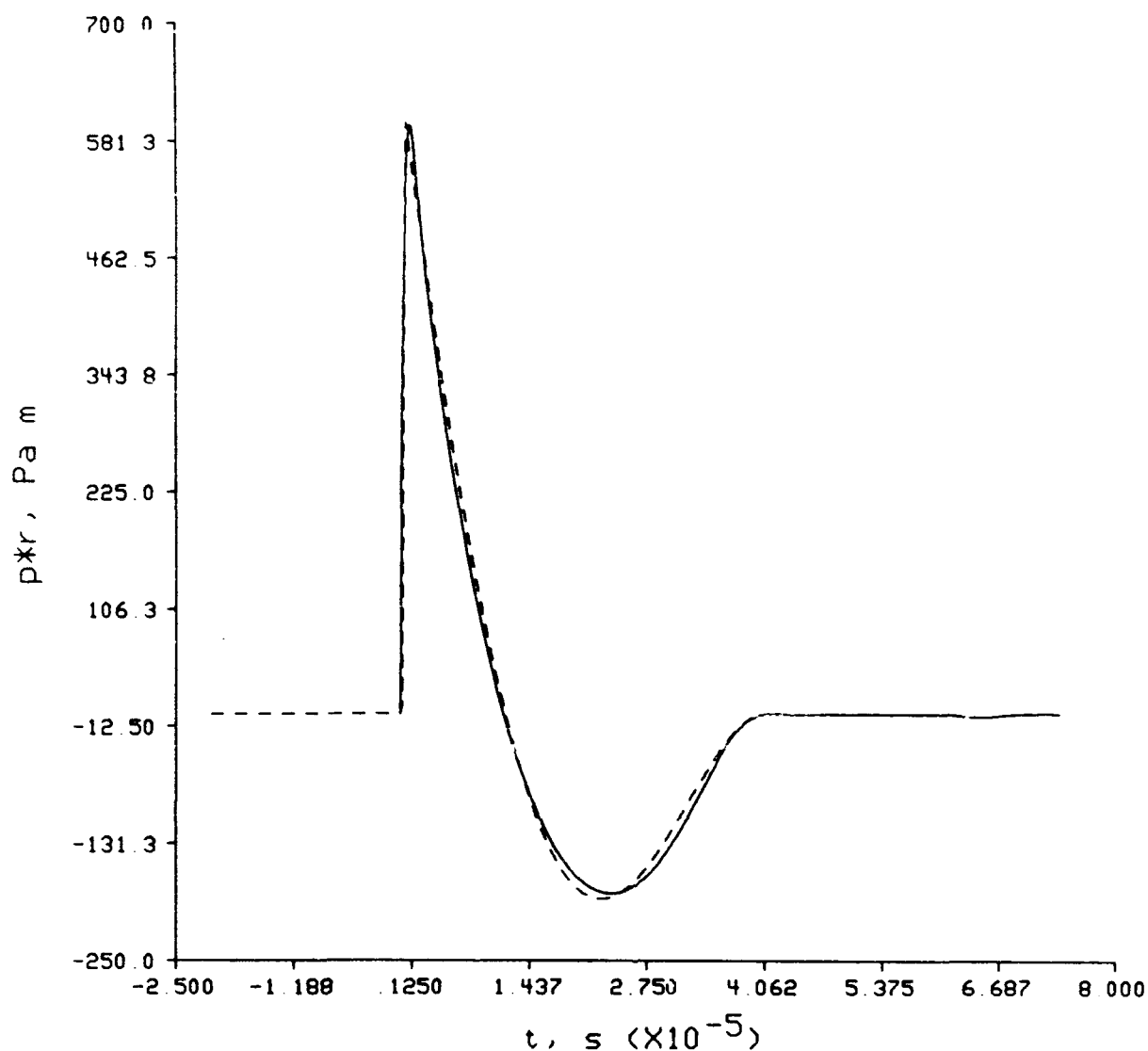
Figure 10.1. A free field spherical spark pulse propagating in air. The solid lines are the finite difference results, and the dashed lines are from the Pestorius algorithm. Time is given relative to a wave traveling at 343 m/s. Initial conditions at d = 0.03 m.
