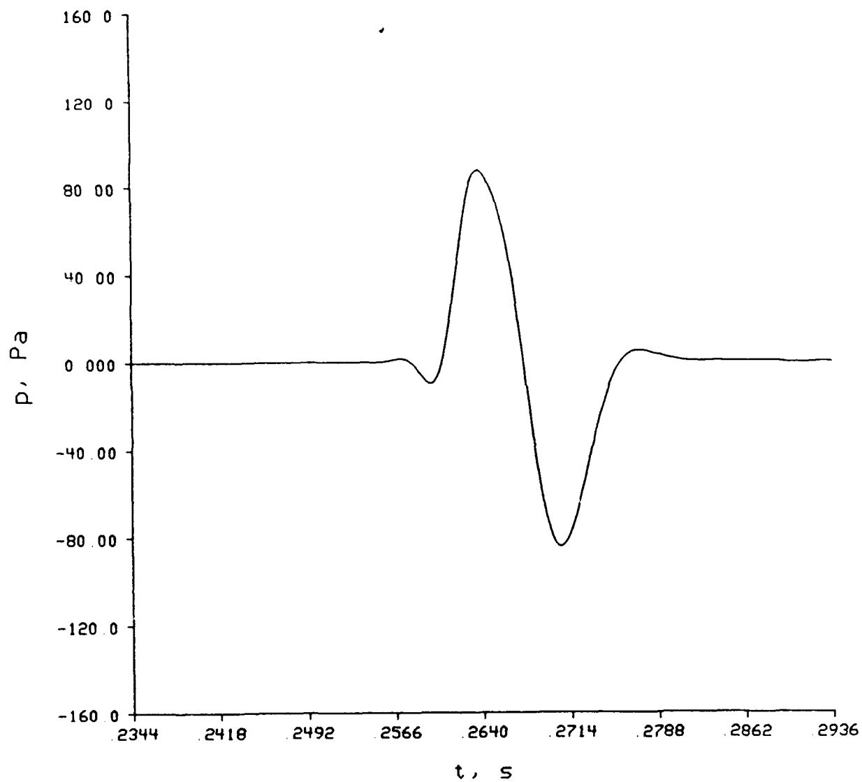
Figure 11.24. Pressure versus time at the 120 m range and the 5 m receiver height for a 150 dB initial peak blast propagating over the porous surface.
