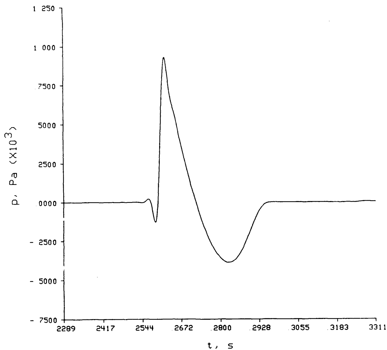
Figure 11.17. Pressure versus time at the 120 m range and the 5 m receiver height for a 162 dB initial peak blast propagating over the hard surface.
