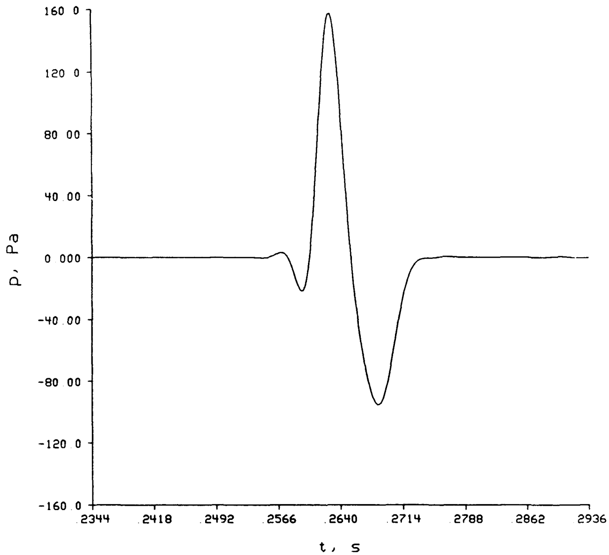
Figure 11.14. Pressure versus time at the 120 m range and the 0 m receiver height for a 150 dB initial peak blast propagating over the hard surface.
