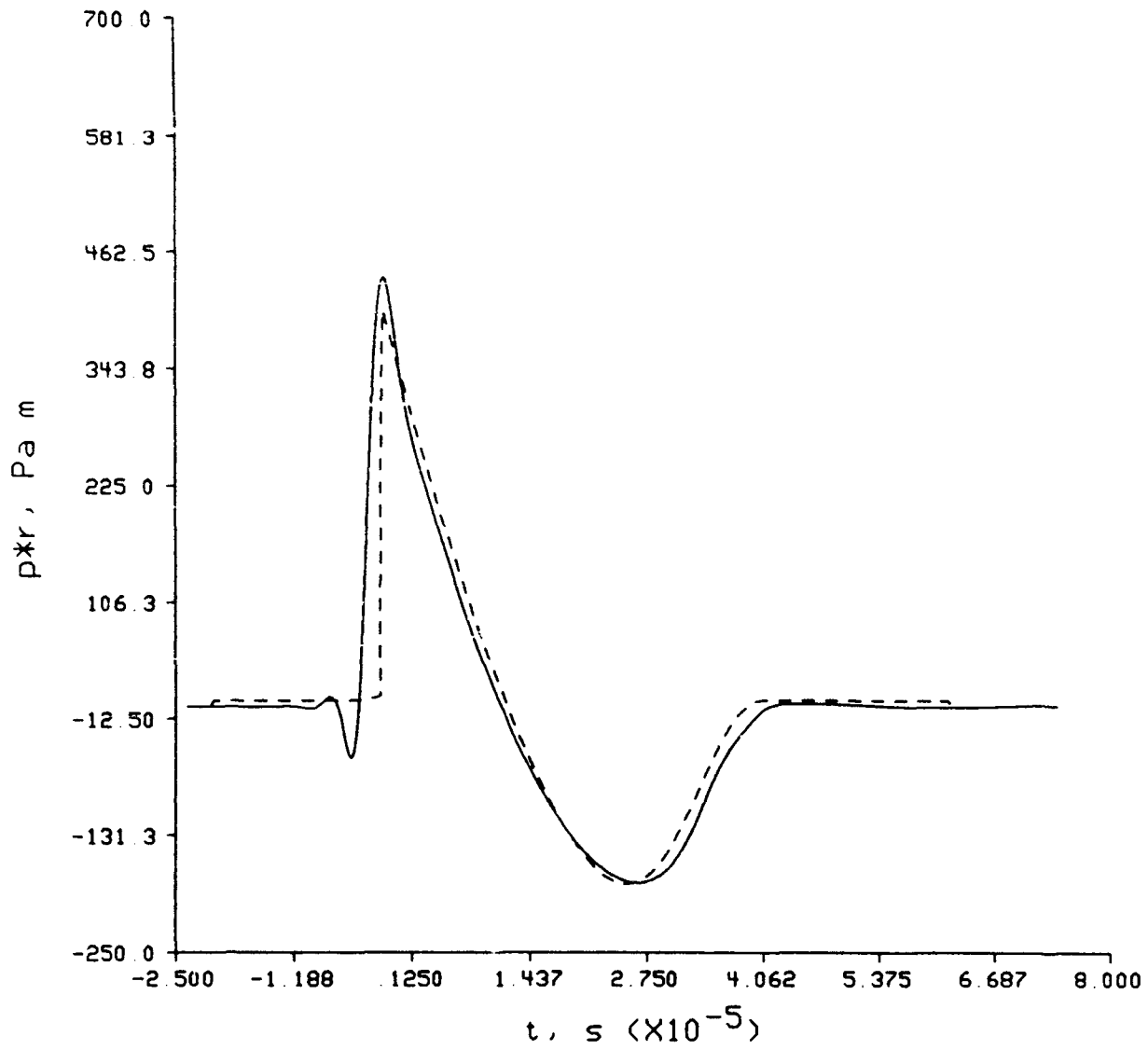
Figure 10.2. Same as Figure 10.1 at d = 0.05744 m.
