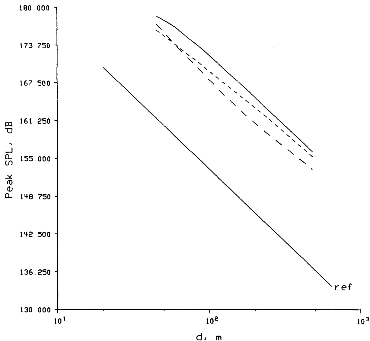
Figure 11.22. 174 dB initial peak pressure SPL versus range for porous surface propagation. The 0 m receiver height is given by the solid line, the 1 m height by the short dashed line, and the 5 m height by the long dashed line. The solid line ending with the label "ref." shows a decay of r^{-1.2} for reference.
