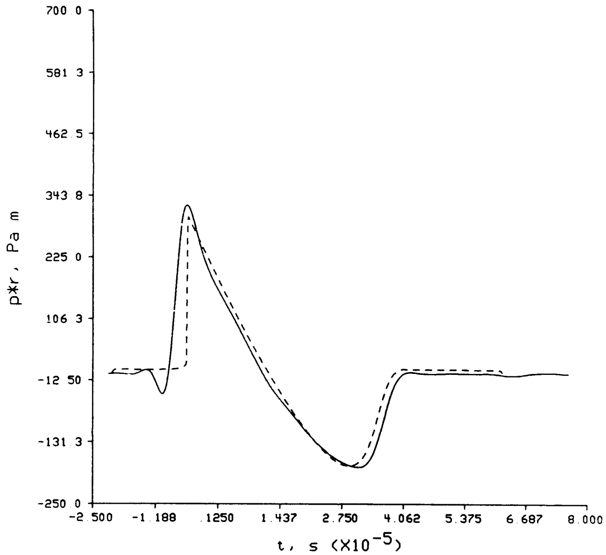
Figure 10.5. Same as Figure 10.1 at d = 0.13976 m.
