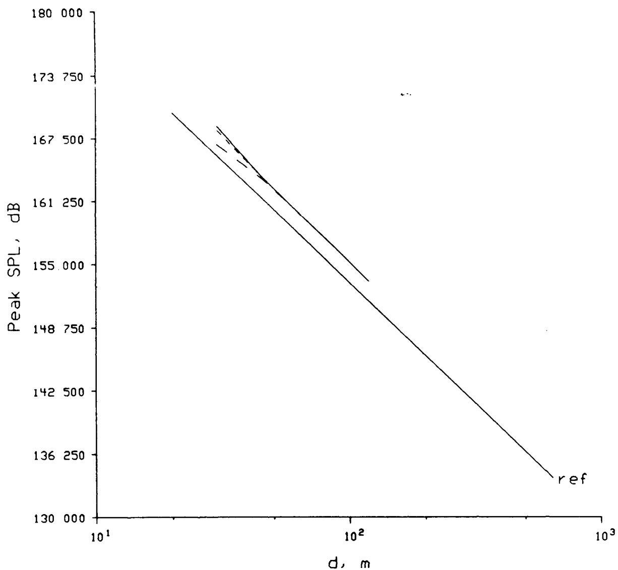
Figure 11.12. 162 dB initial peak pressure SPL versus range for hard surface propagation. The 0 m receiver height is given by the solid line, the 1 m height by the short dashed line, and the 5 m height by the long dashed line. The solid line ending with the label "ref." shows a decay of r^{-1.2} for reference.
