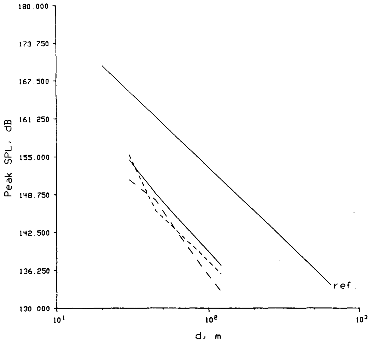
Figure 11.20. 150 dB initial peak pressure SPL versus range for porous surface propagation. The 0 m receiver height is given by the solid line, the 1 m height by the short dashed line, and the 5 m height by the long dashed line. The solid line ending with the label "ref." shows a decay of r^{-1.2} for reference.
