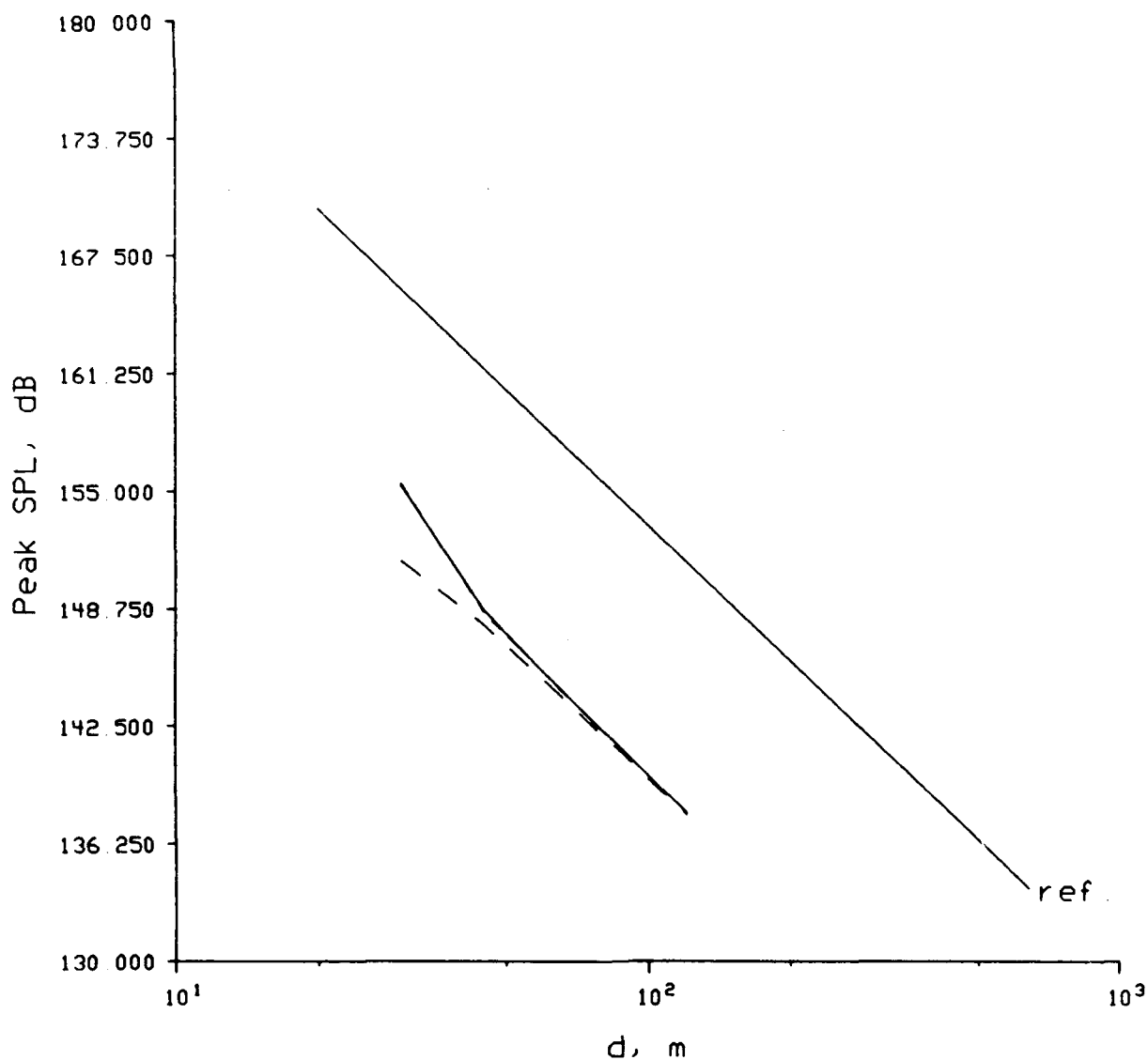
Figure 11.11. 150 dB initial peak pressure SPL versus range for hard surface propagation. The 0 m receiver height is given by the solid line, the 1 m height by the short dashed line, and the 5 m height by the long dashed line. The solid line ending with the label "ref." shows a decay of r^{-1.2} for reference.
