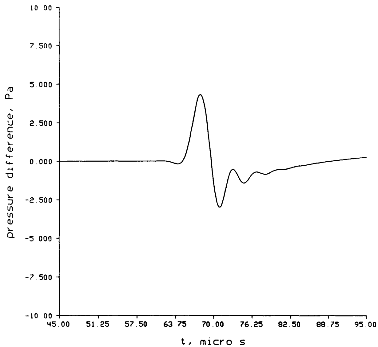
Figure 8.6. Acoustic pressure difference in Pa between cases two and four.
