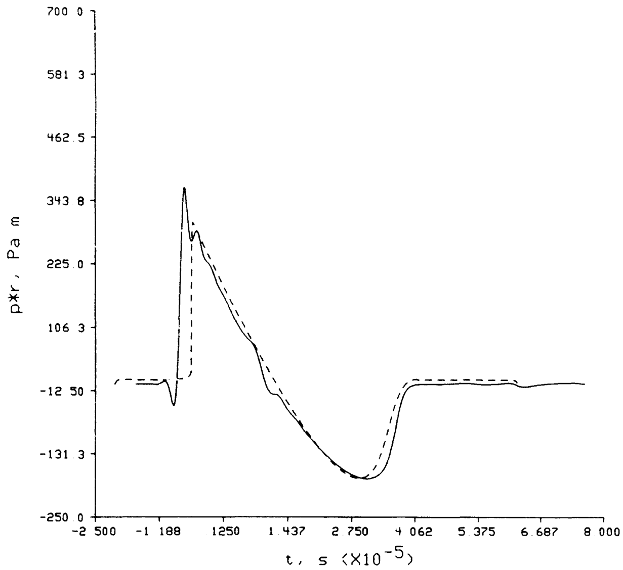
Figure 10.6. Same as Figure 10.1 at d = 0.13976 \text{ m} , with no artificial viscosity.
