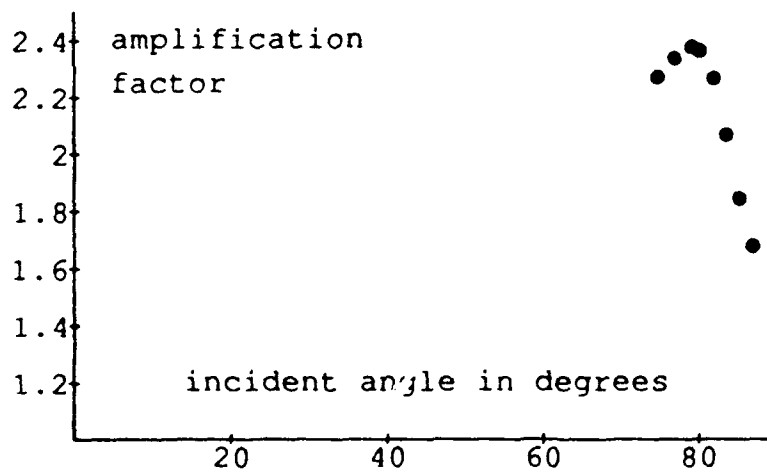
Figure 10.12. Same as Figure 10.9 except the peak pressure is 2.5 kPa, 162 dB.
