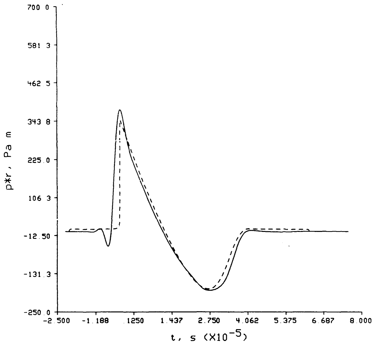
Figure 10.3. Same as Figure 10.1 at d = 0.08488 \text{ m} .
