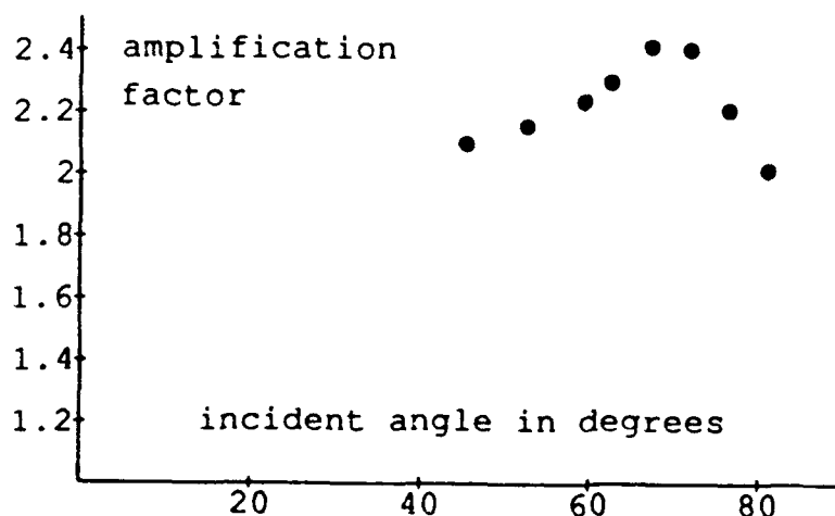
Figure 10.10. Same as Figure 10.9 except the peak pressure is 10.0 kPa, 174 dB.
