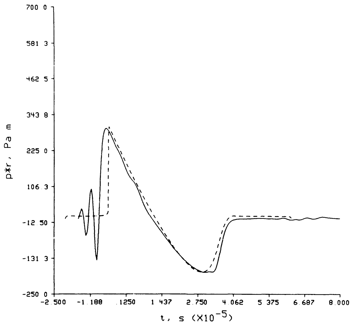
Figure 10.7. Same as Figure 10.1 at d = 0.13976 m, with c_0 \Delta t / \Delta x = 0.5488 and no artificial viscosity.
