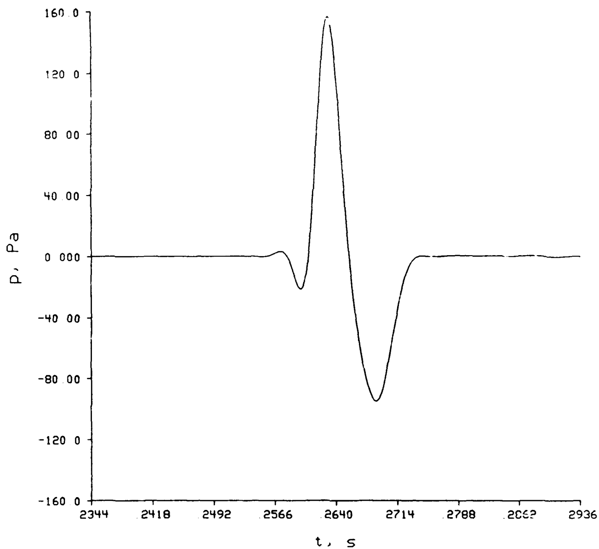
Figure 11.15. Pressure versus time at the 120 m range and the 5 m receiver height for a 150 dB initial peak blast propagating over the hard surface.
