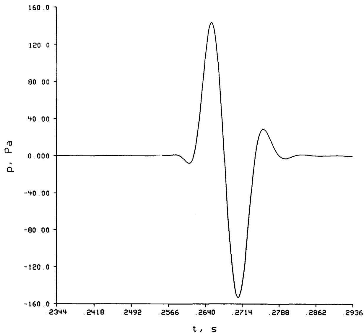
Figure 11.23. Pressure versus time at the 120 m range and the 0 m receiver height for a 150 dB initial peak blast propagating over the porous surface.
