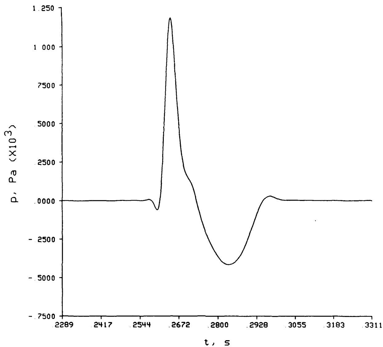
Figure 11.25. Pressure versus time at the 120 m range and the 0 m receiver height for a 162 dB initial peak blast propagating over the porous surface.
