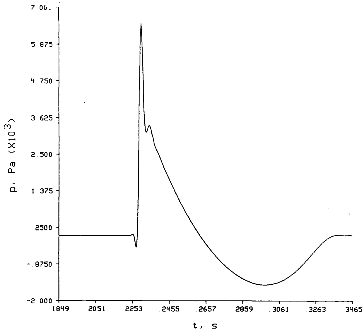
Figure 11.27. Pressure versus time at the 120 m range and the 0 m receiver height for a 174 dB initial peak blast propagating over the porous surface.
