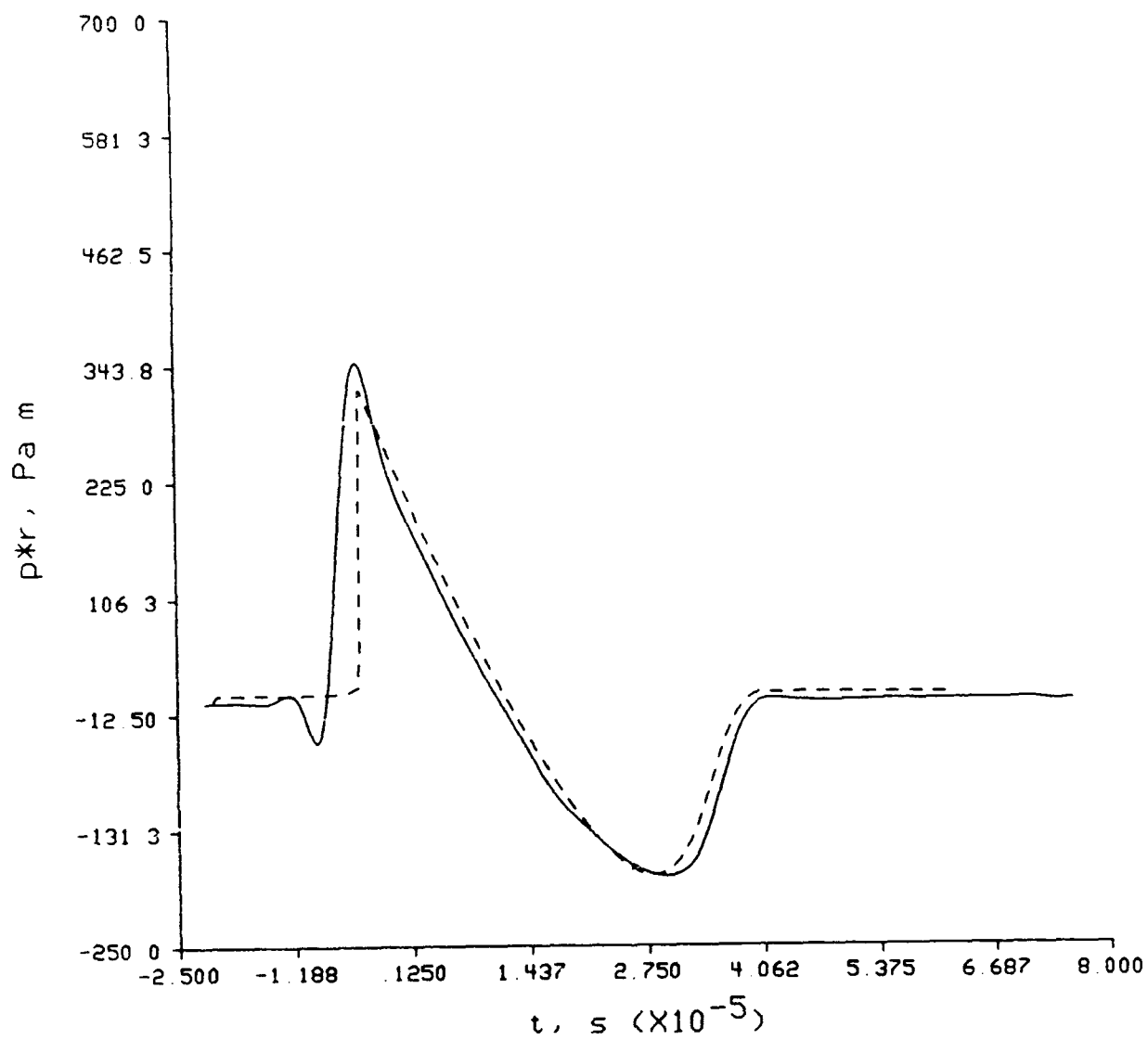
Figure 10.4. Same as Figure 10.1 at d = 0.11232 \text{ m} .
