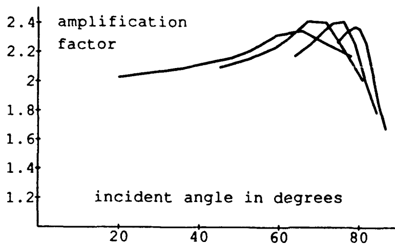
Figure 10.13. A composite of Figures 10.9 to 10.12. Oblique reflection amplification factors versus angle for the four free field incident peak pressures for sparks of 15.0, 10.0, 5.0, and 2.5 kPa.
