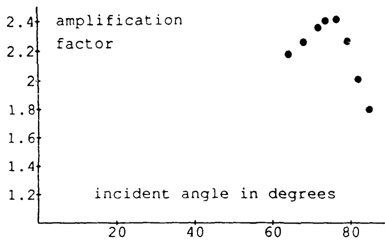
Figure 10.11. Same as Figure 10.9 except the peak pressure is 5.0 kPa, 168 dB.
