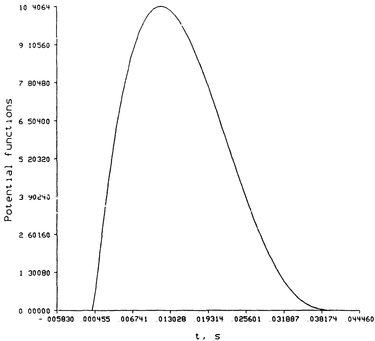
Figure 6.1. Pulse spherical potential from Equation (6.10). The solid line is for the exact I_1 , the dotted line is for the approximate I_1 .
