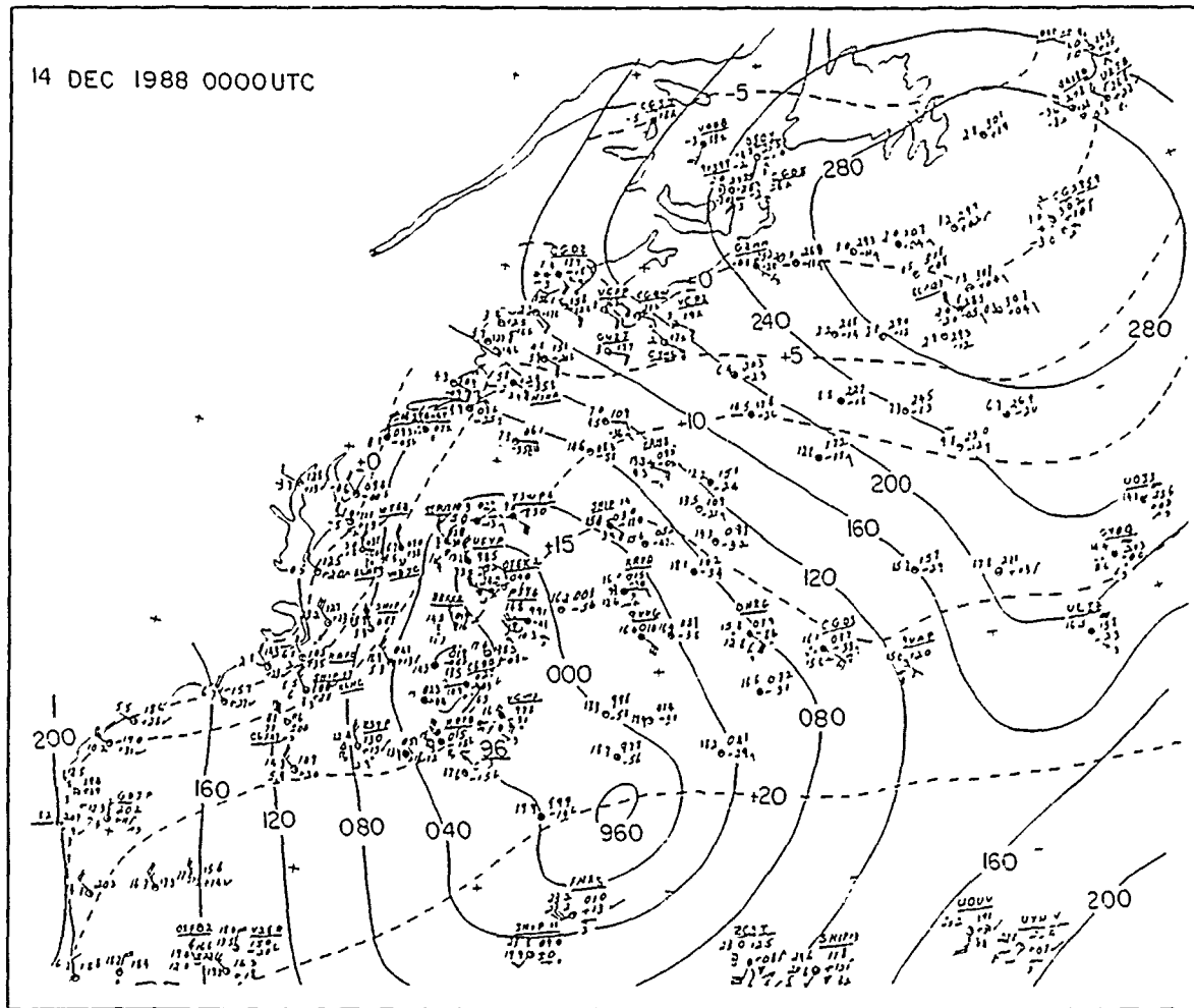
Fig. 13. IOP-2 14/0000 UTC December 1988 surface analysis: Sea-level pressure (solid) in tenths of mb where the leading 9 or 10 has been dropped and surface temperature (dashed) in °C (Sanders, 1989).
