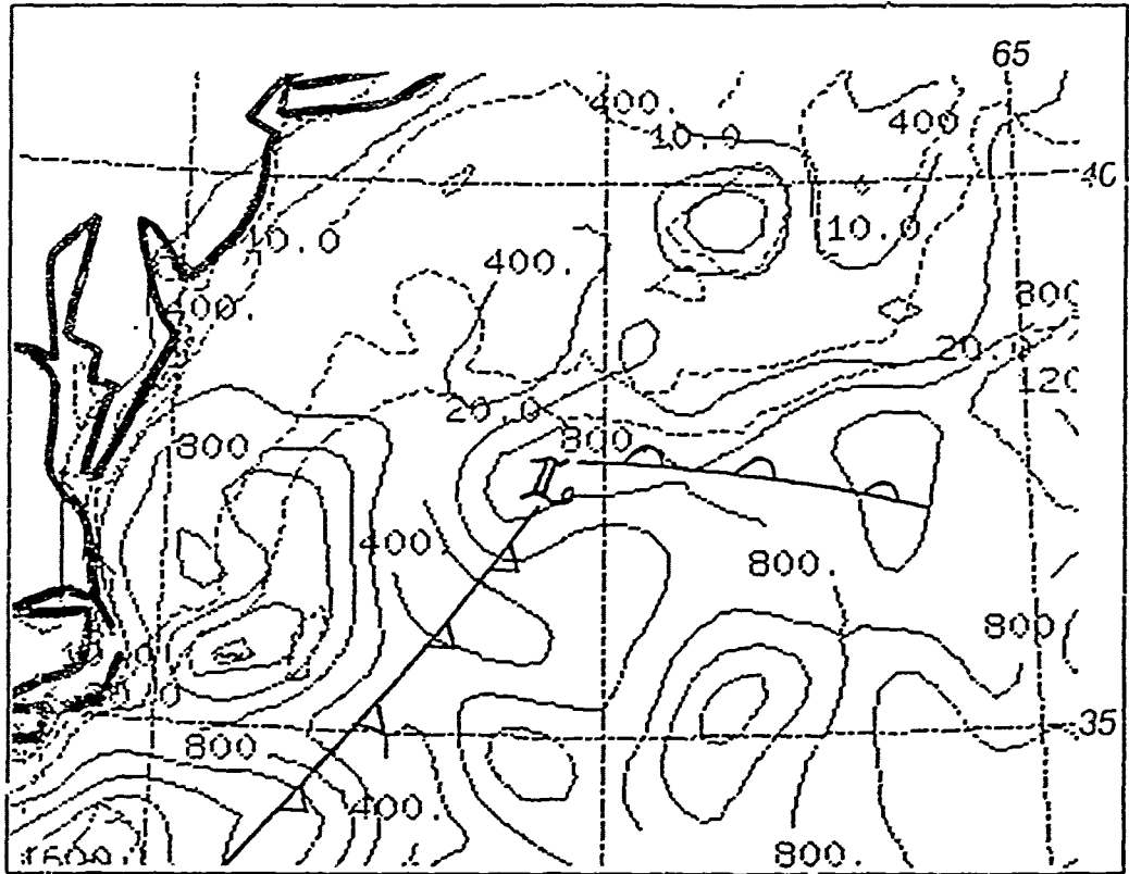
Fig. 28. Latent heat fluxes for 13/1800 UTC: Latent heat fluxes in intervals of 200 \text{ W m}^{-2} , SST (dashed) in ^{\circ}\text{C} .
