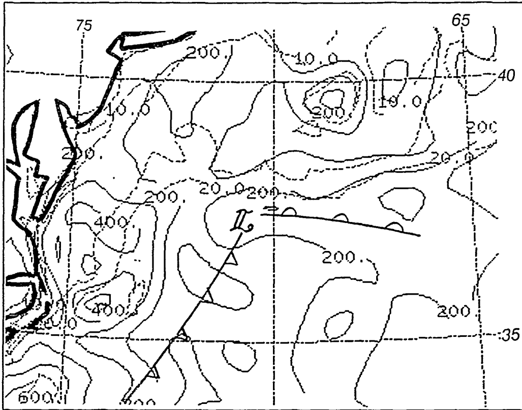
Fig. 27. Sensible heat fluxes for 13/1800 UTC: Sensible heat fluxes in intervals of 100 W m^{-2} , SST (dashed) in ^{\circ}C .
