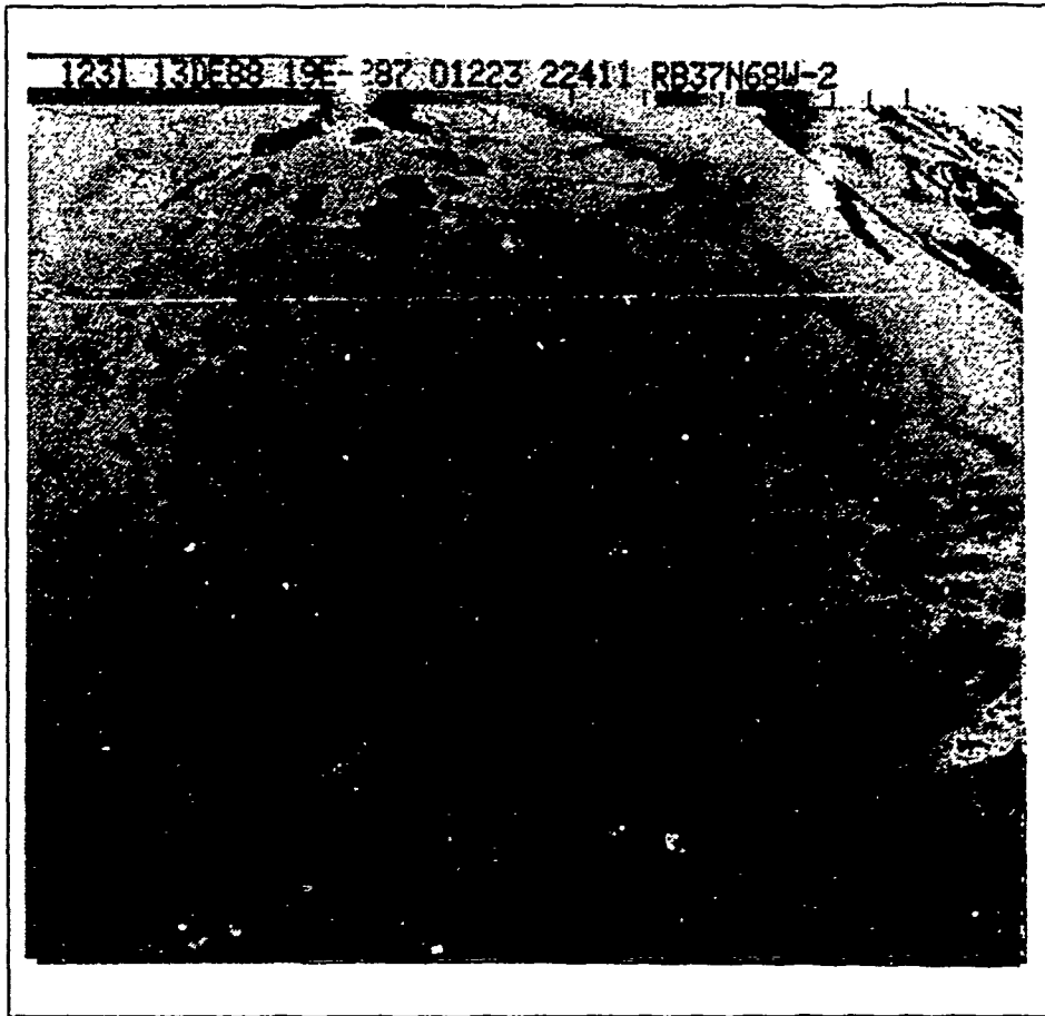
Fig. 4. GOES IR imagery for 13/1231 UTC December 1988: U.S. East Coast sector.
