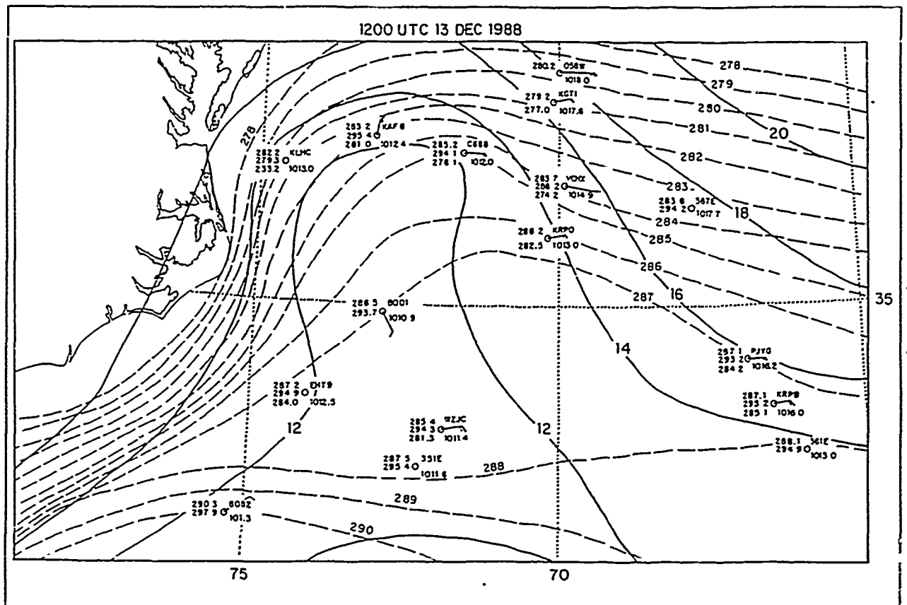
Fig. 6. IOP-2 13/1200 UTC December 1988 mesoscale surface frontal analysis: Sea-level pressure (solid) in mb and surface temperature (dashed) in °C.
