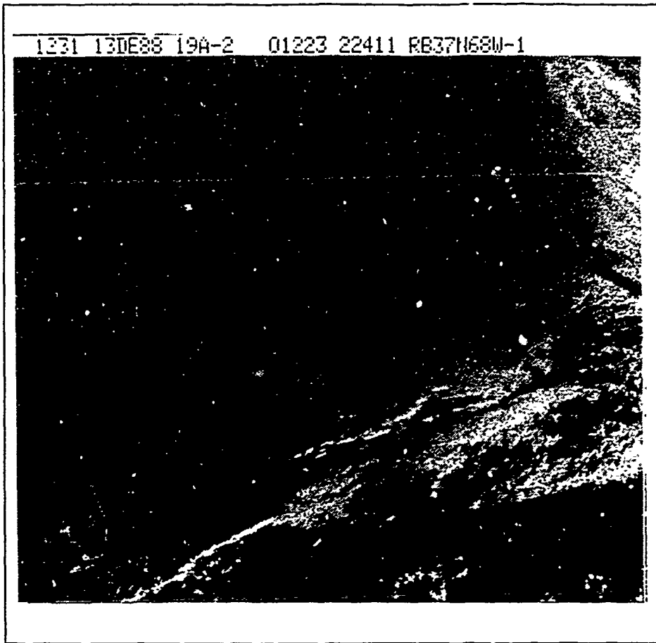
Fig. 5. GOES VIS imagery for 13/1231 UTC December 1988: U.S. East Coast sector.
