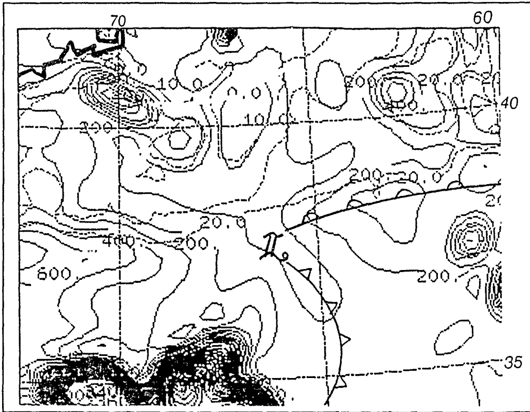
Fig. 29. Sensible heat fluxes for 14/0600 UTC: Sensible heat fluxes in intervals of 100 \text{ W m}^{-2} , SST (dashed) in ^{\circ}\text{C} .
