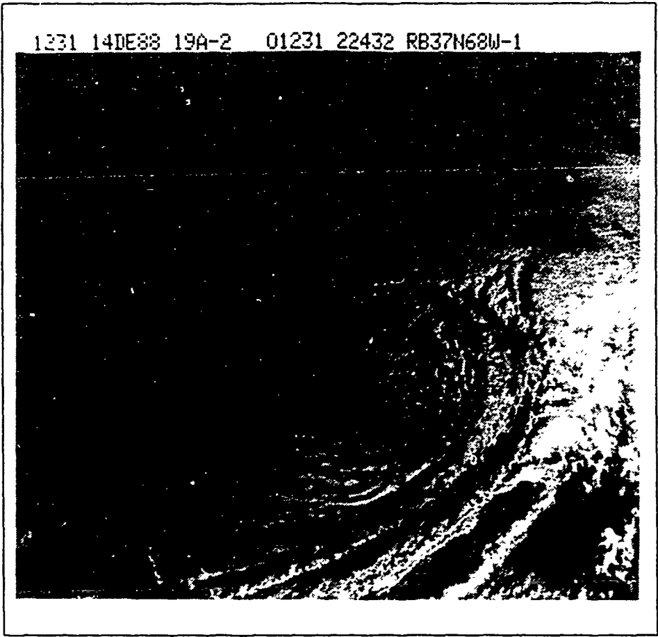
Fig. 18. GOES VIS imagery for 14/1231 UTC December 1988: U.S. East Coast sector.
