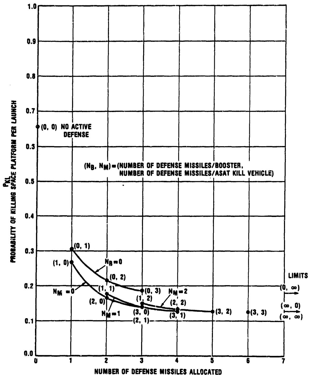
FIGURE 1. PKL vs number of defense missiles allocated assuming all parameter values = 0.90 and N_V = 1
