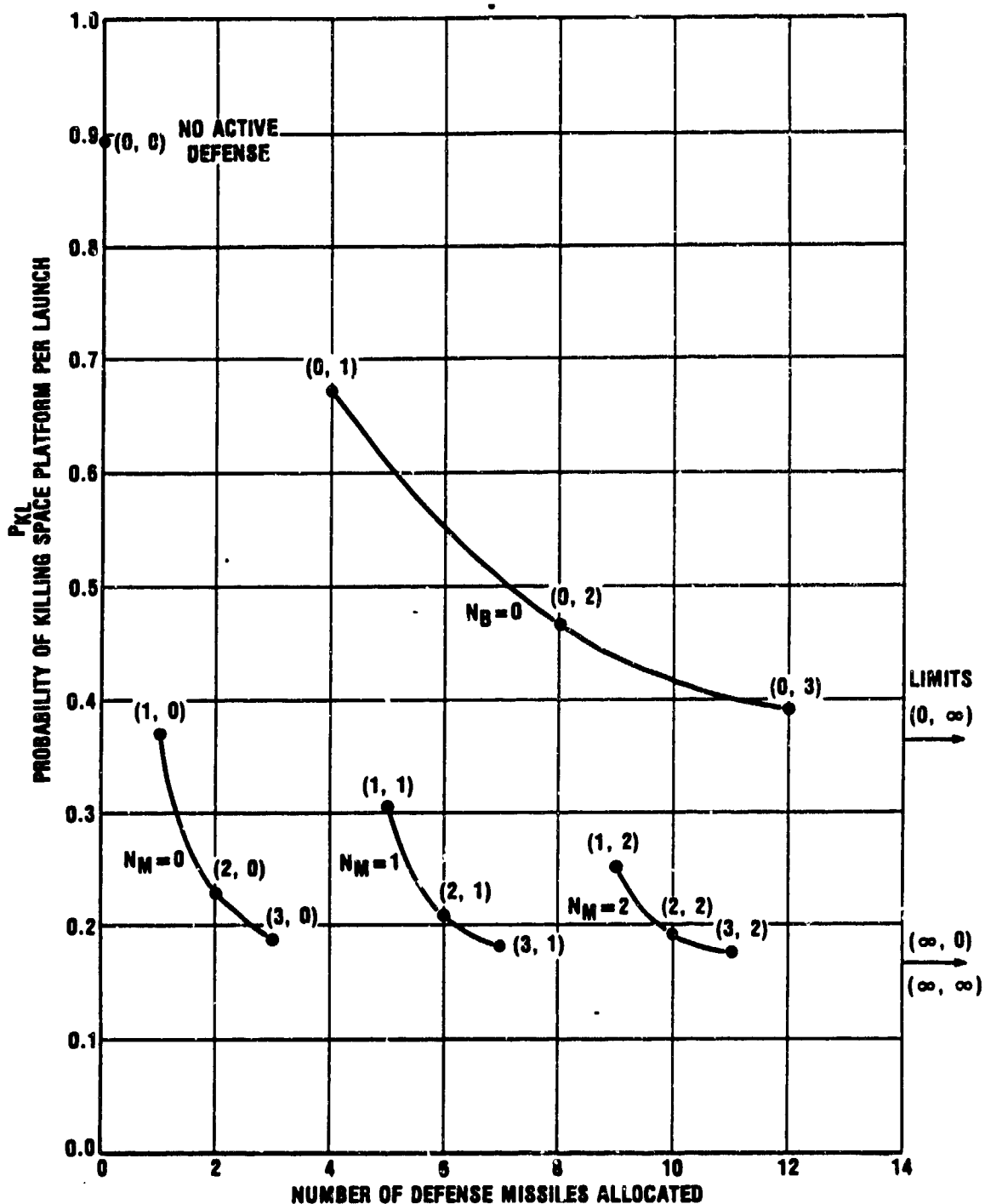
FIGURE 4. P_{KL} vs number of defense missiles allocated assuming all parameter values = 0.90 N_V = 4
