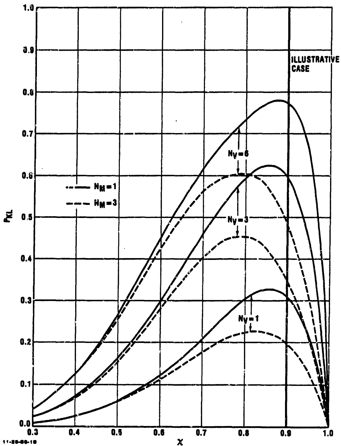
FIGURE 7. P_{KL} vs x , assumed to be the common parameter value for all reliability, detection and kill probability parameters N_B = 0
