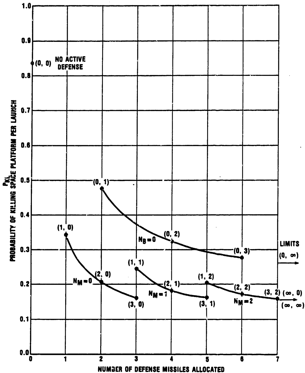
FIGURE 2. P_{KL} vs number of defense missiles allocated assuming all parameter values = 0.90 N_V = 2
