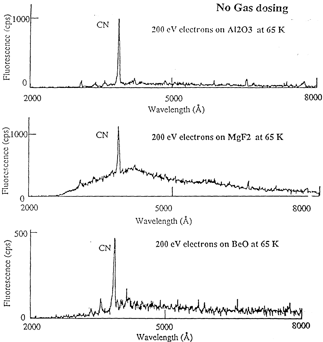
Figure 4 Fluorescence induced by 200 eV electrons impacting on Al 2 O 3 , MgF 2 and BeO surfaces at 65 K
