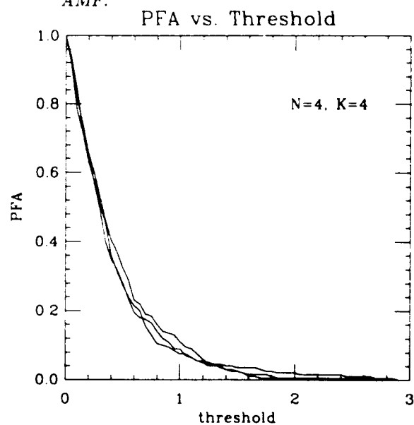
Figure 39. Probability of false alarm vs threshold. Chapter 7 likelihood ratio.
